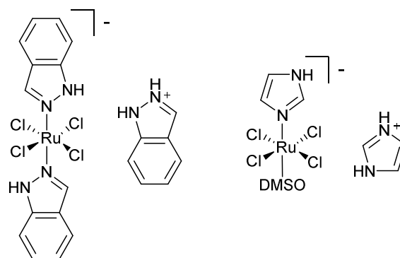
Figure 2. Structures of (from the left) KP1019 and NAMI-A.
