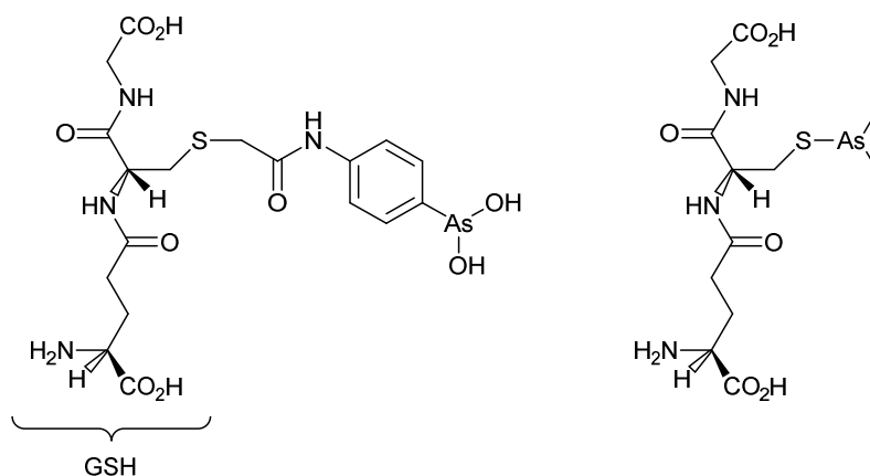
Figure 5. The structures of (from the left) GSAO and darinaparsin.
