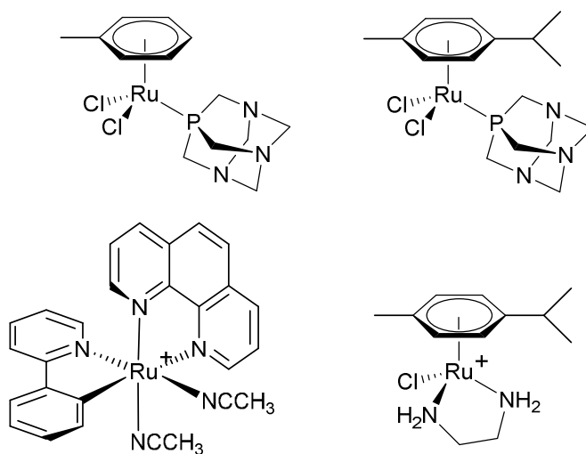
Figure 3. The structures of (from the left) RAPTA-T (top left), RAPTA-C (top right), RDC11 (bottom left) and RAED-C (bottom right). RDC11 and RAED-C are formulated as PF 6 - salts.
