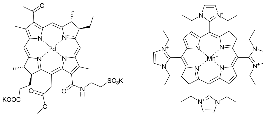
Figure 7. The structure of (from the left) TOOKAD-soluble and AEOL-10150 (formulated as the chloride salt).
