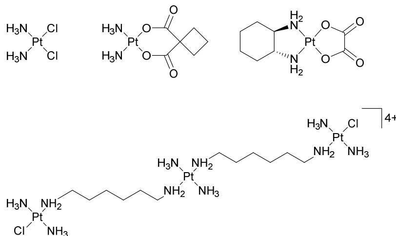
Figure 1. Structures of (from the left) cisplatin, carboplatin, oxaliplatin, and (bottom) triplatin tetranitrate, i.e. BBR3464 (or CT-3610).
