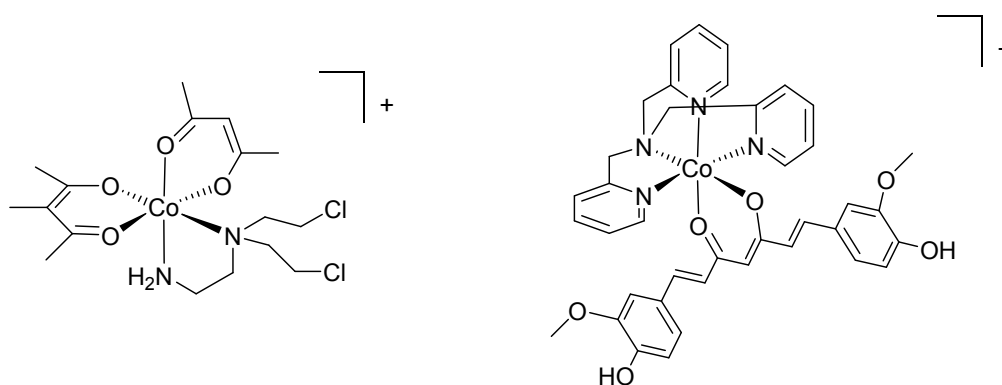
Figure 4. Examples of (from the left) a complex that releases a nitrogen mustard ligand and a curcumin ligand in hypoxic cancer tissue. Both complexes are formulated as \text{ClO}_4^- salts.
