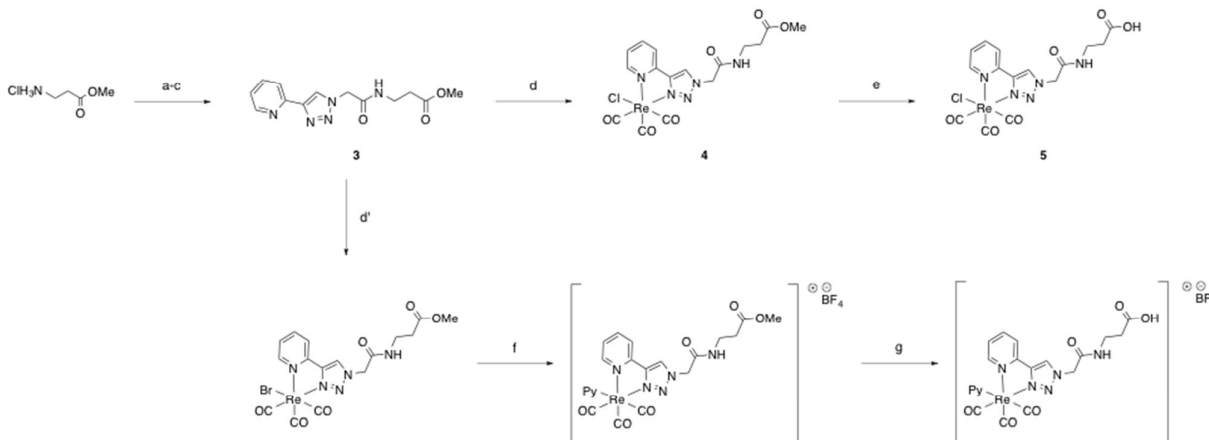
Scheme 1. Synthesis of the SCoMPI derivatives. Reaction conditions : (a) chloroacetyl chloride, DCE, dry DCM, 1h, 0°C to RT, 66%, (b) NaN 3 , NaI, acetone/water (3:1 v:v), 16h, 35°C, 79%, (c) 2-ethynylpyridine, CuSO 4 , sodium ascorbate, acetone/water (2:1 v:v), 2h, RT, 70%, (d) Re(CO) 5 Cl, toluene, 6h, reflux, 100%, (d') Re(CO) 5 Br, toluene, 6h, reflux, 100%, (e) LiOH·H 2 O, THF/H 2 O (2:1 v:v), 45min., RT, 80%, (f) i. AgBF 4 , acetonitrile, 5h, reflux, Ar; ii. pyridine, THF, 20h, reflux, 79%, (g) LiOH·H 2 O, THF/H 2 O (2:1 v:v), 45min., RT, 87%.
