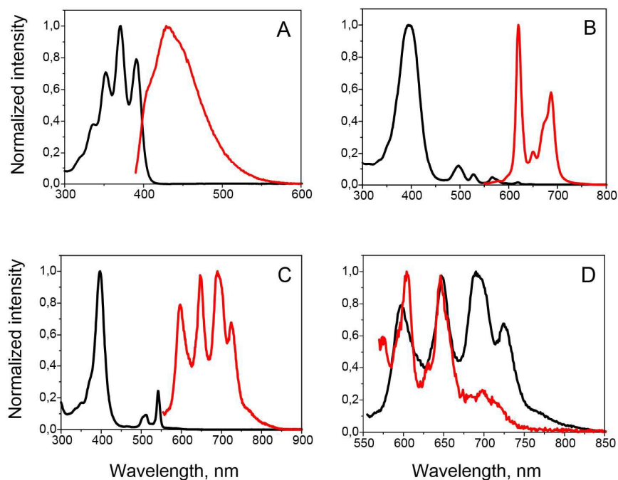
Fig. 2. Absorption (black) and emission (red) spectra of anthracene 3 (A), porphyrins 8 (B) and 9 (C). (D) Comparison of porphyrin 9 ( 3 \times 10^{-5} M) emission under inert atmosphere (black) and under air (red).
