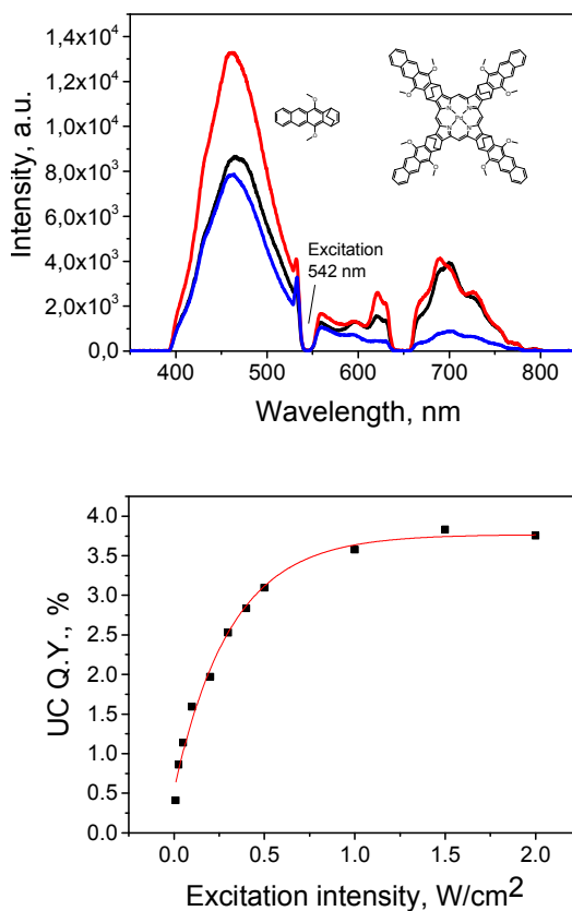
Fig. 8. Upconversion luminescence of the mixture of 9 and 3 and quantum yield dependence on the excitation intensity (for the mixture of 6 \times 10^{-4} M 3 and 3 \times 10^{-5} M 9 respectively). Solvent: toluene. Samples were excited at \lambda = 542 nm ( 10 mWcm -2 ).
