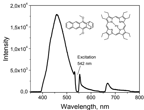
Fig. 5. Upconversion spectrum of PdOEP ( 10^{-5} M) and 5,12-dimethoxy-1,4-dihydro-1,4-ethanotetracene ( 5 \times 10^{-4} M) in air-free toluene.
