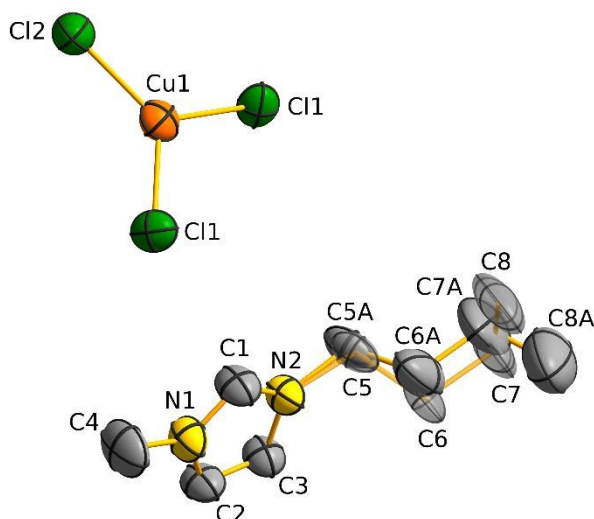
Fig. 7 Asymmetric unit of the high temperature phase of (\text{C}_4\text{mim})_2\text{CuCl}_3 with disordered butyl residue. Relative occupancy CXA: CX = 0.62:0.38(2). Hydrogen atoms are omitted for clarity.
