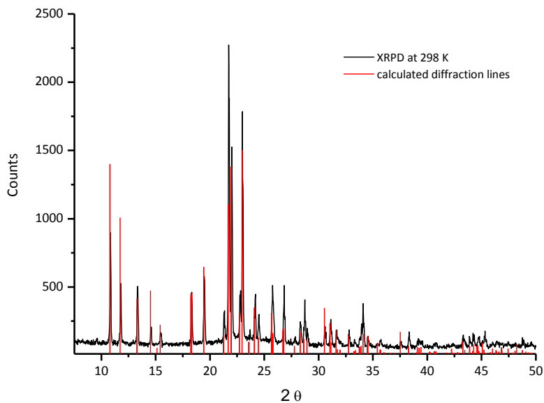
Fig. 1 X-ray powder diffraction pattern of (C_4mim)_2CuCl_3 (Cu- K_\alpha ) at ambient temperature. The simulated diffraction pattern was calculated using the 233 K crystal structure with refined lattice parameters for 298 K (see supplementary information).
