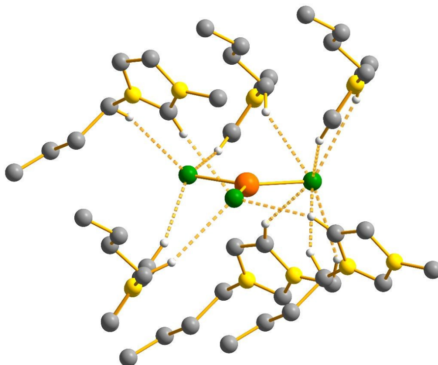
Fig. 8 C-H...Cl contacts of planar [\text{CuCl}_3]^{2-} anions and \text{C}_4\text{mim}^+ cations up to 2.97 Å. Disordered atoms and hydrogen atoms not involved in C-H...Cl contacts have been omitted for clarity.
