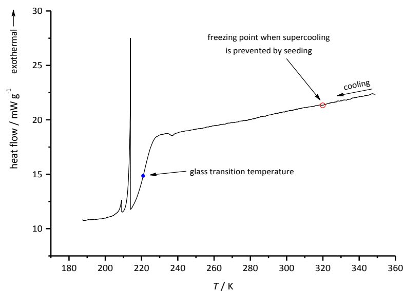
Fig. 5 DSC cooling trace of molten (\text{C}_4\text{mim})_2\text{CuCl}_3 ( 1 \text{ K min}^{-1} ). No crystallisation is observed (red circle). A glass transition occurs at 221 K (blue circle). Small exothermal signals are probably due to a small fraction of the sample crystallising whilst the majority is transformed into the glassy state.
