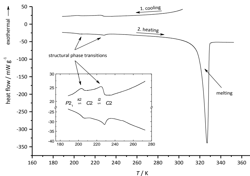
Fig. 3 DSC traces of (C_4mim)_2CuCl_3 crystals at a scan rate of 2\text{ K min}^{-1} showing two reversible solid-solid phase transitions at 227 and 203 K. The solid undergoes congruent melting at 320 K.
