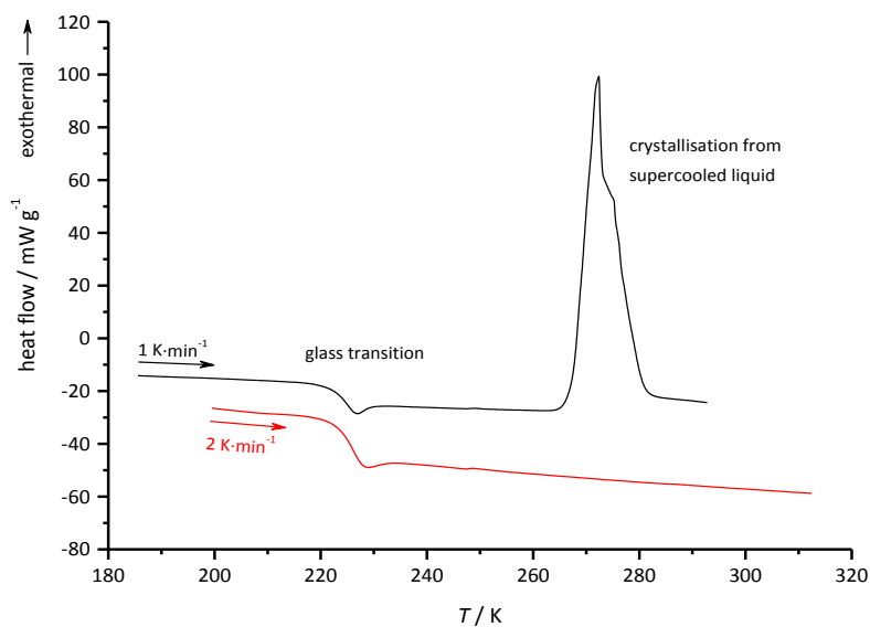
Fig. 6 DSC heating traces of (\text{C}_4\text{mim})_2\text{CuCl}_3 . At the slower scan rate crystallisation occurs from the supercooled liquid at 267 K.
