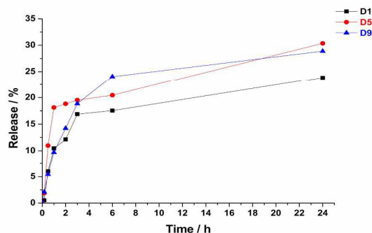
Fig. 5: Release profiles of [\text{Gd}(\text{DTPA})(\text{H}_2\text{O})]^{2-} from \text{Ni}_2\text{Zn}_3\text{-Gd}(\text{DTPA}) .
