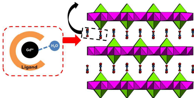
Fig. 2: A schematic illustration of the intercalation of Gd complexes into an HDS. M(OH)_6 octahedra are in purple and M(OH)_4 tetrahedra in green. Nitrate ions can be seen between the layers.
