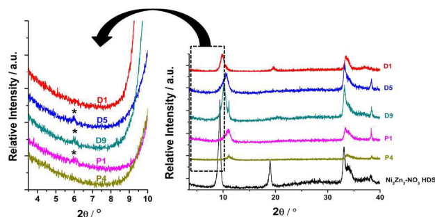
Fig. 3: X-ray diffraction patterns for the products of selected reactions between Ni_2Zn_3-NO_3 and [Gd(DTPA)(H_2O)]^{2-} ("D" samples) and [Gd(DTPMPH_5)(H_2O)]^{2-} ("P" samples), with intercalate reflections marked with *.
