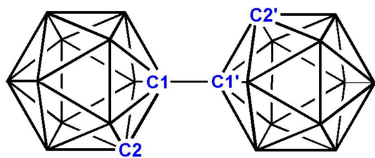
Fig. 1. 1,1'-bis(o-carborane)
