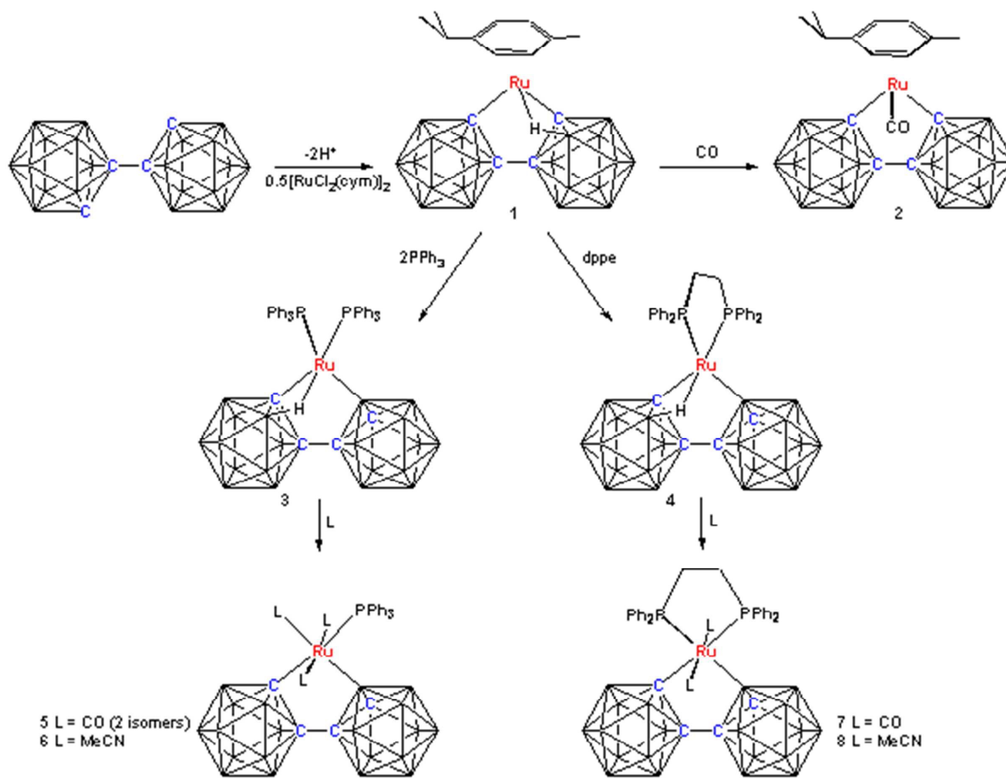
Scheme 1. General reaction scheme for compounds 1-8.
