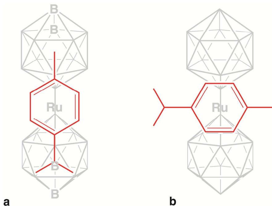
Fig. 3. Possible orientations of the p -cymene ligand above the Ru{ \kappa^2 -2,2'-[1-(1'-1',2'- closo -C 2 B 10 H 10 )-1,2- closo -C 2 B 10 H 10 ]} unit in compound 1 such that the molecular symmetry is C s . The observation of four BH resonances of integral 3 in the 1 H{ 11 B} NMR spectrum is only consistent with conformation a , not conformation b .
