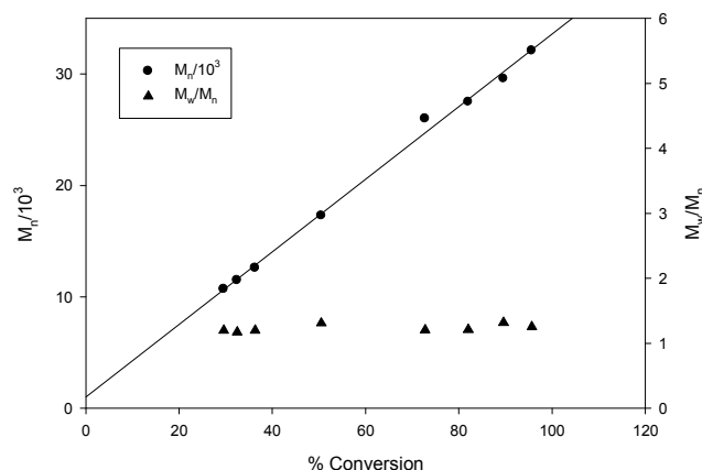
Figure 12. Plot of PLA M_n and dispersity ( M_w/M_n ) as a function of rac -lactide conversion [Conditions: \text{CH}_2\text{Cl}_2 5 mL, 2.95 mmol LA, 250 LA:1 Li:1 BnOH, 25 °C]. Line shown to indicate the linear trend and proportional increases in M_n as conversion increases.
