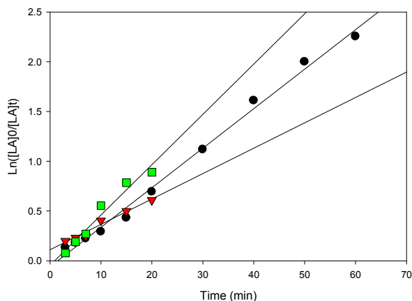
Figure 9. First-order plot of LA consumption initiated by 3 . [Conditions: 2.95 mmol LA, 250 LA:1 Li:0 BnOH, 25 °C]. ● CH 2 Cl 2 (5 mL, y = 0.0397x - 0.0594 , R^2 = 0.9933 ), ■ Toluene (30 mL, 0.0506x - 0.0448 , R^2 = 0.96 ), ▼ THF (20 mL ■ Toluene ( y = 0.0255x + 0.1097 , R^2 = 0.9742 )).
