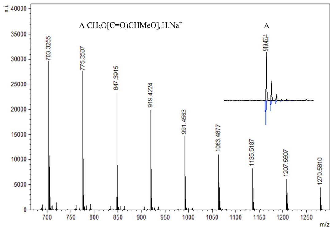
Figure 15. Representative region of the MALDI-TOF mass spectrum (reflectron mode) of PLA formed using 1 under the following conditions: \text{CH}_2\text{Cl}_2 (5 mL), 2.95 mmol LA, 250 LA:1 Li:2 BnOH, 25 °C.
