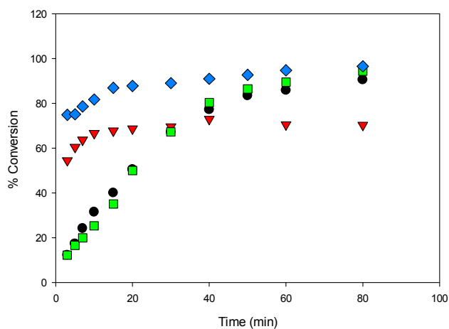
Figure 10. Conversion (%) vs. time for the ROP of LA initiated by 1 , 2 , 3 and 4 in \text{CH}_2\text{Cl}_2 (5 mL) [Conditions: 2.95 mmol LA, 250 LA:1 M:0 BnOH, 25 °C] ● 1 , ▼ 2 , ■ 3 , ◆ 4 .
