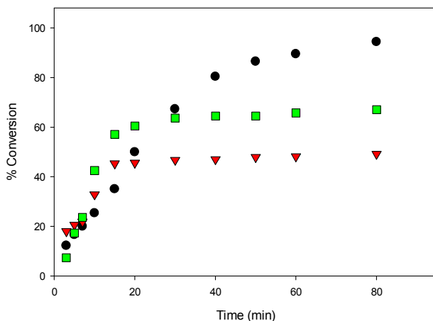
Figure 8. Conversion (%) vs. time for the ROP of LA initiated by 3 [Conditions: 2.95 mmol LA, 250 LA:1 Li:0 BnOH, 25 °C]. ● CH 2 Cl 2 (5 mL), ■ Toluene (30 mL), ▼ THF (20 mL).
