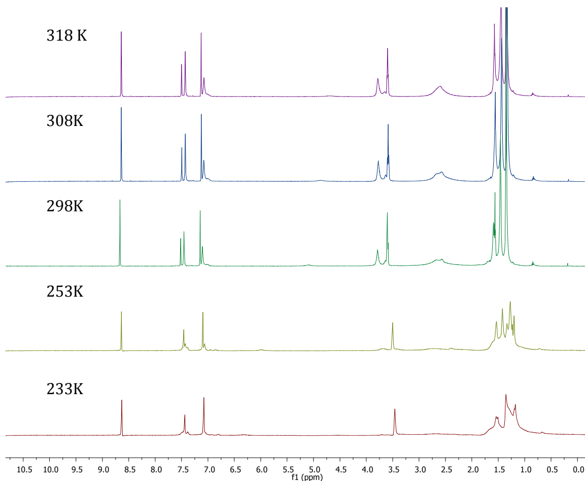
Figure 5. VT ^1\text{H} NMR spectrum (500 MHz, \text{C}_5\text{D}_5\text{N} ) of 1 .
