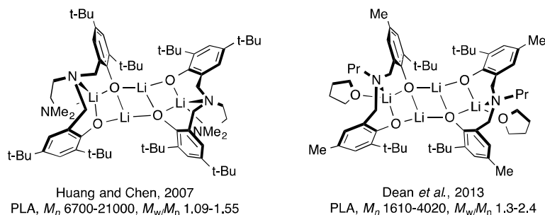
Figure 1. Known tetralithium complexes of amino-bis(phenolate) ligands.
