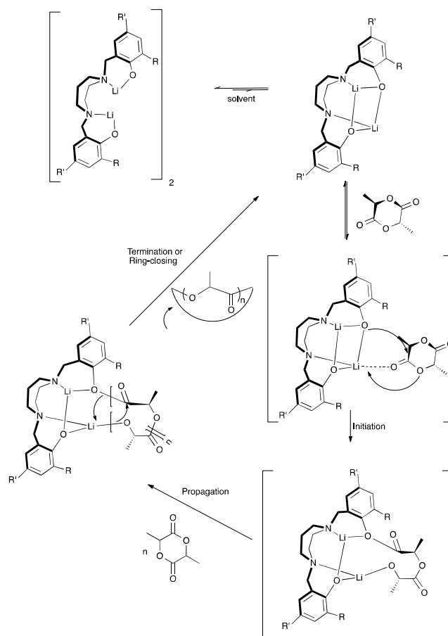
Figure 16. Proposed mechanism of the ROP of rac -LA in the absence of BnOH initiated by lithium and sodium diamino-bis(phenolate) complexes (THF omitted for clarity, coordination
