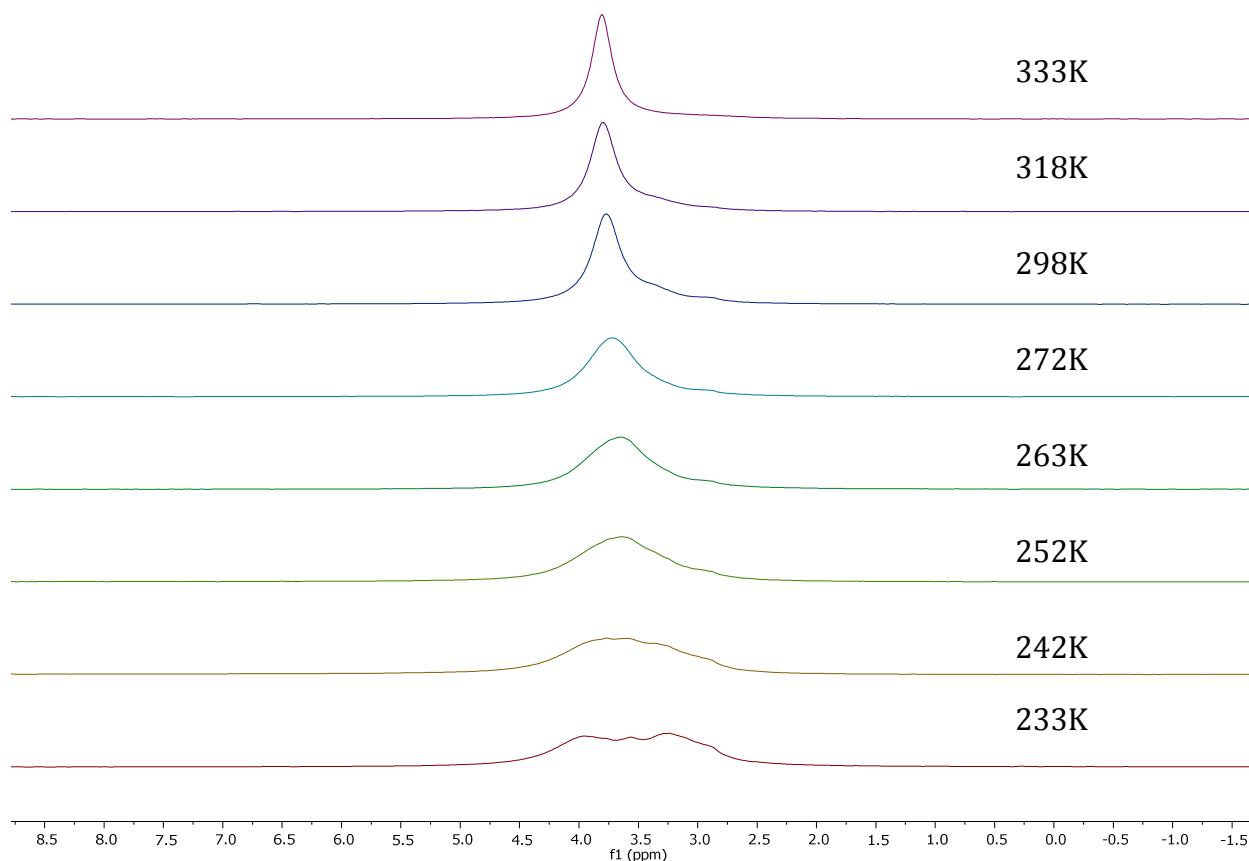
Figure 6. VT 7 Li NMR spectrum (300 MHz, C 5 D 5 N) of 1 ( \omega_{1/2} values were calculated from the line fitting program in MestReNova NMR processing software).
