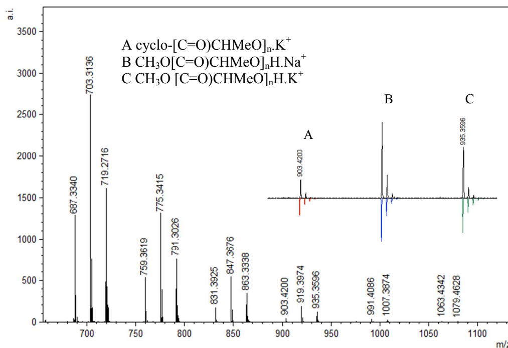
Figure 14. Representative region of the MALDI-TOF mass spectrum (reflectron mode) of PLA formed using 3 under the following conditions: \text{CH}_2\text{Cl}_2 (5 mL), 2.95 mmol LA, 250 LA:1 Li:0 BnOH, 25 °C (similar spectra obtained for PLA from other reactions using no BnOH).
