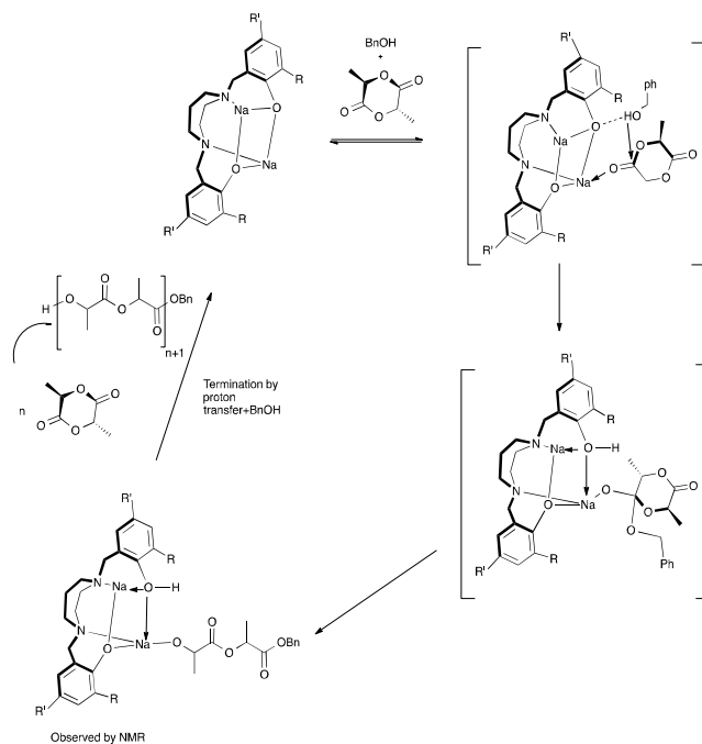
Figure 17. Proposed mechanism of the ROP of rac -LA in the presence of BnOH initiated by sodium diamino-bis(phenolate) complexes (THF omitted for clarity, coordination sphere of the metals will be completed by either LA or THF).
