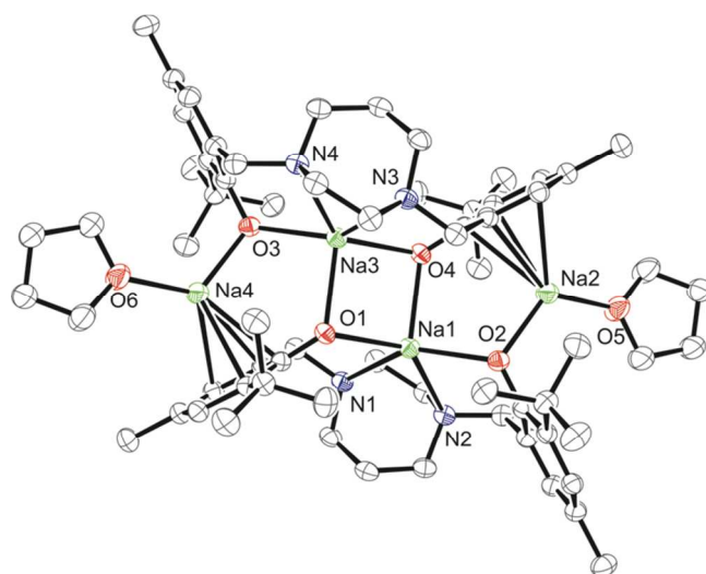
Figure 3. Molecular structure (ORTEP) and partial numbering scheme for 4 . Ellipsoids are shown at the 50% probability level (H-atoms omitted for clarity).
