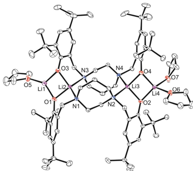
Figure 2. Molecular structure (ORTEP) and partial numbering scheme for 1 . Ellipsoids are shown at the 50% probability level (H-atoms omitted for clarity).
