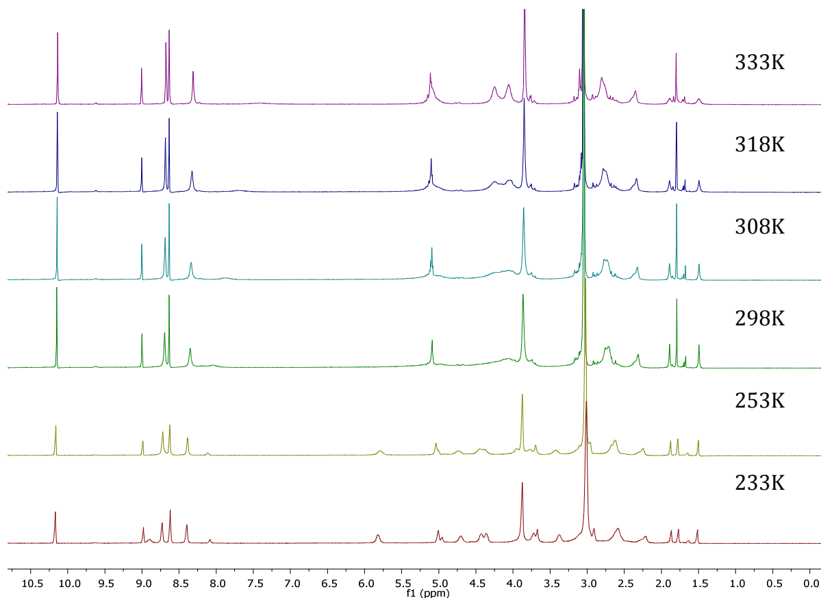
Figure 7. VT 1 H NMR spectrum (500 MHz, C 5 D 5 N) of 4 .
