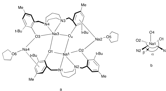
Figure 4. [a] Schematic representation of 4 . [b] Representation of the five-coordinate environment of Na(1).
