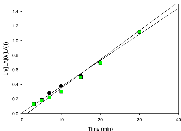
Figure 11. First-order plot of LA consumption initiated by 1 and 3 in \text{CH}_2\text{Cl}_2 (5 mL) [Conditions: 2.95 mmol LA, 250 LA:1 Li:0 BnOH, 25 °C], ● 1 ( y = 0.0358x + 0.0123 , R^2 = 0.9954 ), ■ 3 ( y = 0.0395x - 0.0471 , R^2 = 0.9951 ).
