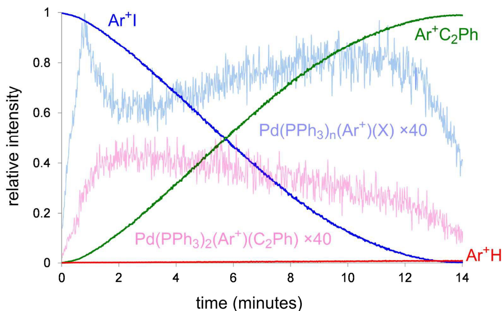
Figure 8: ESI(+)-MS over time for the intensity of all key species bearing the charged tag for the normal reaction in \text{CD}_3\text{OD} in the presence of DBU ( \text{Ar}^+ = [\text{C}_6\text{H}_4\text{CH}_2\text{PPh}_3]^+ ). The reaction conditions were as in Scheme 2 with the exception of \text{CD}_3\text{OD} instead of \text{MeOH} . The intensities of the \text{Pd}(\text{PPh}_3)_n\text{ArX} ( \text{X} = \text{I}^- or DBU) and \text{Pd}(\text{PPh}_3)_2(\text{Ar})(\text{C}_2\text{Ph}) have been multiplied by 40 for illustrative purposes. Traces are ESI(+)-MS data normalized to the total ion current.
