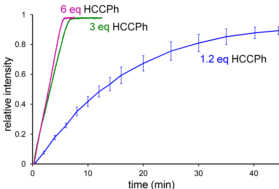
Figure 5: Appearance of product over time when using 1.2 (blue), 3 (green), and 6 (pink) equivalents of phenylacetylene. In this plot, \text{Ar}^+\text{I} (0.5 mM in 20 mL MeOH, \text{Ar}^+ = [\text{C}_6\text{H}_4\text{CH}_2\text{PPh}_3]^+ ) was reacted with phenylacetylene (1.2, 3, or 6 equivalents) in the presence of DBU (10 equivalents) and \text{Pd}(\text{PPh}_3)_4 (6 mol % in 2 mL THF). Traces are ESI(+)-MS data normalized to the total ion current.
