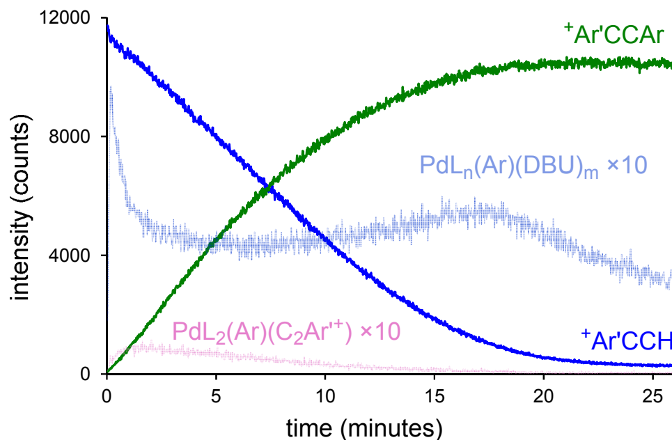
Figure 3: ESI(+)-MS intensities over time of all key species bearing the charged tag [\text{C}_2\text{C}_6\text{H}_4\text{CH}_2\text{PPh}_3]^+ ( \text{Ar} = \text{C}_6\text{H}_5\text{Me} ; \text{L} = \text{PPh}_3 ; \text{X} = \text{I}^- or \text{DBU} ). The intensities of the palladium-containing intermediates have been multiplied by 10 for illustrative purposes. Reaction conditions are as in Scheme 3.
