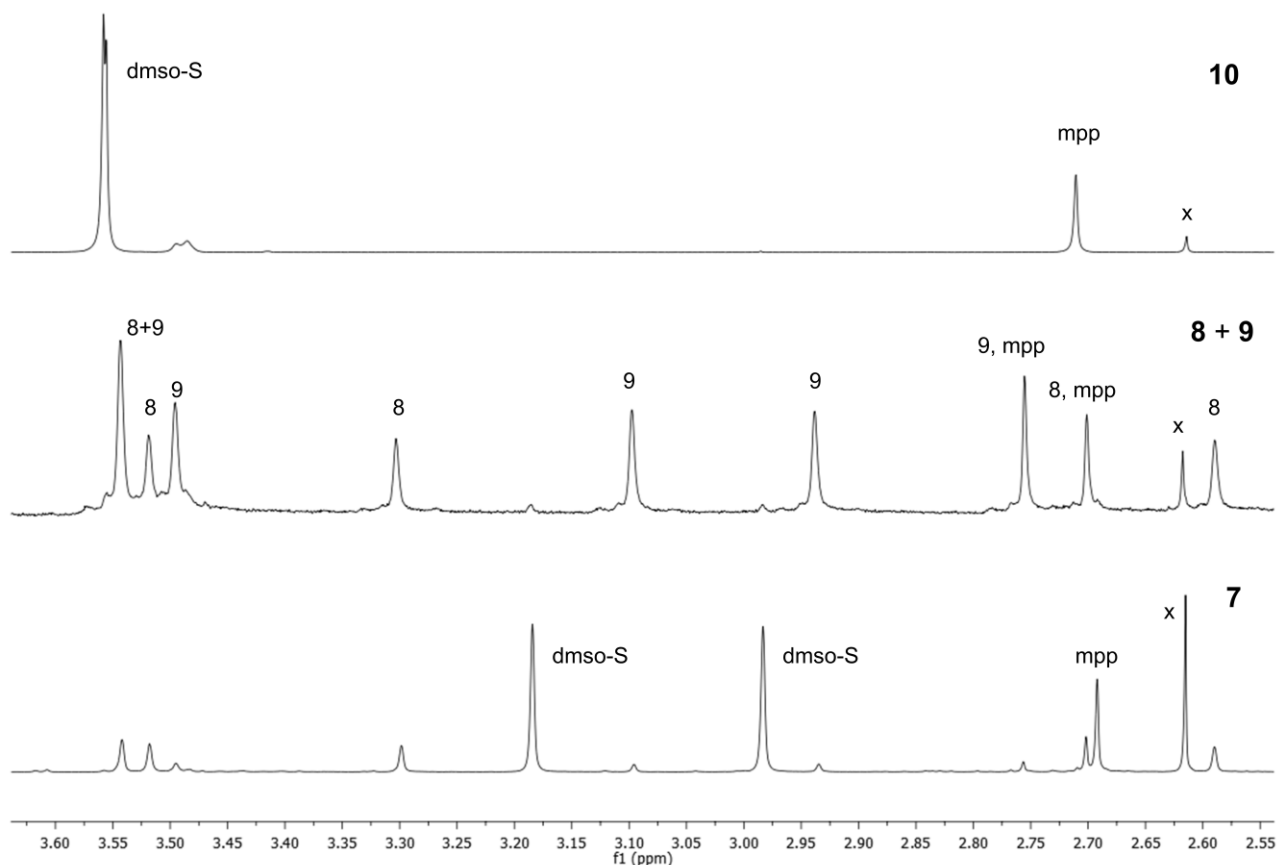
Figure 7. The region of the methyl resonances in the ^1\text{H} NMR spectra ( \text{CDCl}_3 ) of cis,trans - [\text{RuCl}_2(\text{dmsol-S})_2(\text{mpp-}\kappa\text{N}^P)] ( 7 , bottom, with minor amounts of 8 and 9 ), a mixture of the two cis,cis - [\text{RuCl}_2(\text{dmsol-S})_2(\text{mpp-}\kappa\text{N}^P)] isomers ( 8 + 9 , middle), and trans,cis - [\text{RuCl}_2(\text{dmsol-S})_2(\text{mpp-}\kappa\text{N}^P)] ( 10 , top). In the central spectrum, the eight dmsol-S resonances are labeled with the number of the corresponding complex. The peak of residual free DMSO is labeled with x.
