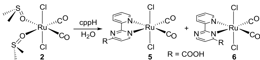
Scheme 2. The reaction between 2 and cppH, yielding the two linkage isomers trans,cis -[RuCl 2 (CO) 2 (cppH-κN p )] ( 5 ) and trans,cis -[RuCl 2 (CO) 2 (cppH-κN o )] ( 6 ). The nature of compound 6 was established on the basis of the 15 N NMR spectra.
