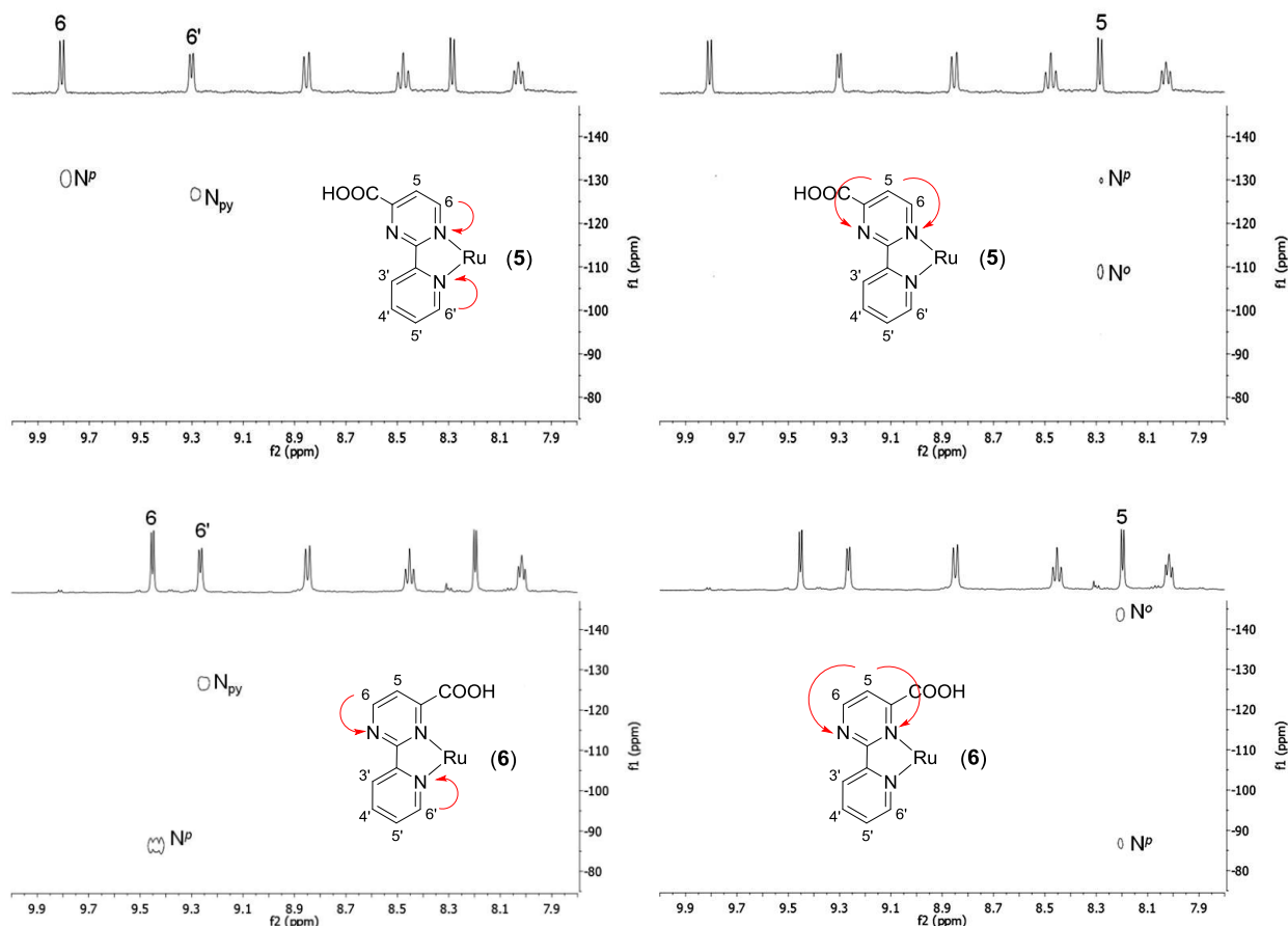
Figure 9. \{^1\text{H}, ^{15}\text{N}\} -HMBC NMR spectra of trans,cis - [\text{RuCl}_2(\text{CO})_2(\text{cppH}-\kappa\text{N}^p)] ( 5 , top) and trans,cis - [\text{RuCl}_2(\text{CO})_2(\text{cppH}-\kappa\text{N}^o)] ( 6 , bottom) in DMSO- d_6 with J = 11 Hz (left) and J = 1.7 Hz (right).
