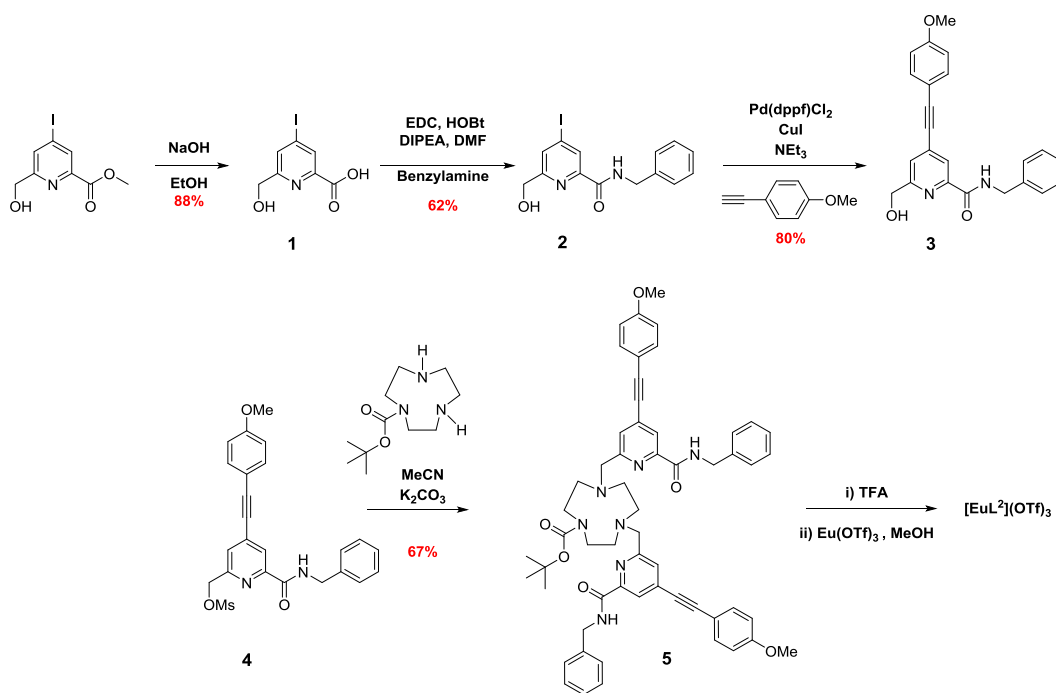
Scheme 1 Synthesis of L^2 and its Eu(III) complex
