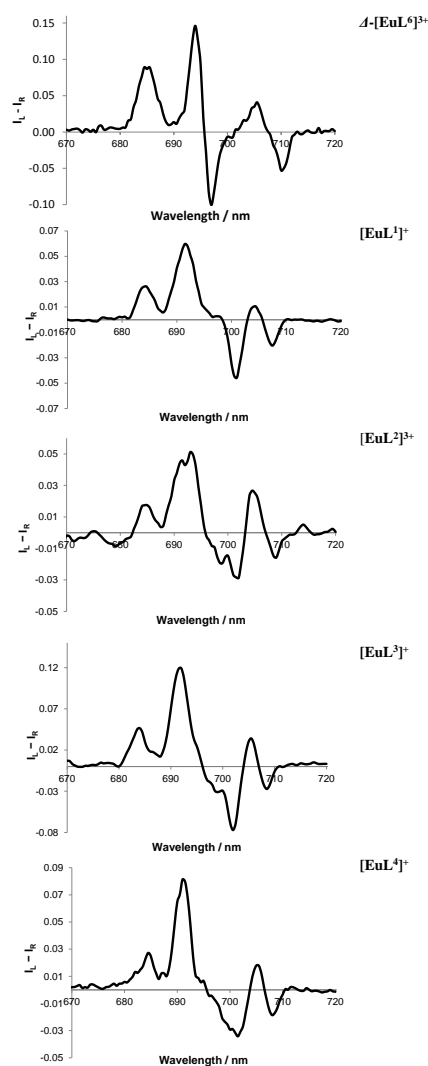
Figure 6 Partial CPL spectra for Eu(III) complexes of L^{1-4} , compared to \Delta -[Eu.L 6 ] 3+ (top), showing the similar \Delta J = 4 manifold in the presence of excess R -cyclohexylhydroxyacetic acid (295K, H 2 O, 10 \mu M complex, 50 \mu M acid), correlating with selective formation of a \Delta -complex in each case. Mirror image profiles were obtained adding S -acid. (see ESI for total emission and full CPL spectra of each system).
