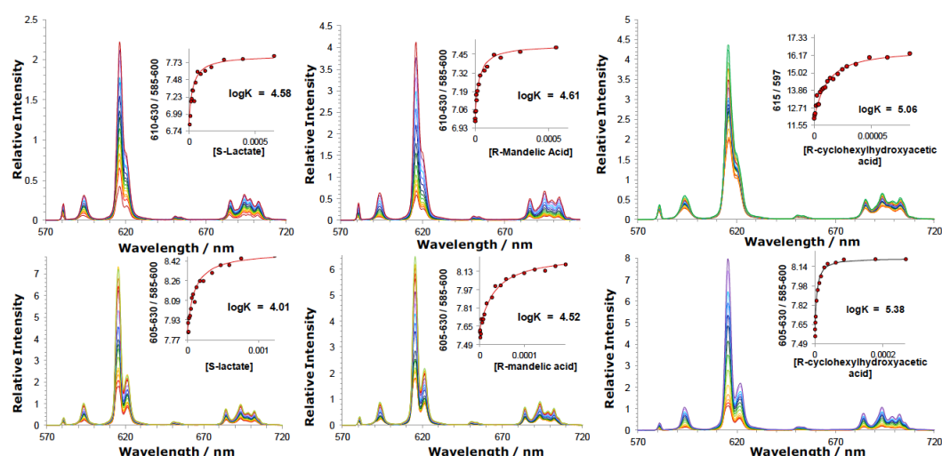
Figure 1 Variation of the europium (III) emission profile as a function of added anion; ( upper ): [\text{Eu.L}^2]^{3+} (5 \mu\text{M} ; \lambda_{\text{exc}} 348 nm, \text{H}_2\text{O} , pH 5.5), ( left to right ) lactate, mandelate and cyclohexylhydroxyacetate; ( lower ): [\text{Eu.L}^3]^+ (5 \mu\text{M} ) ( \lambda_{\text{exc}} = 352 nm, 50% MeOH in \text{H}_2\text{O} , pH 5.5) plus added anions. Insets show fits to experimental data, following iterative non-linear least-squares fitting to a 1:1 binding model (details in the ESI). No significant differences in measured binding constants were found with enantiomeric carboxylates.
