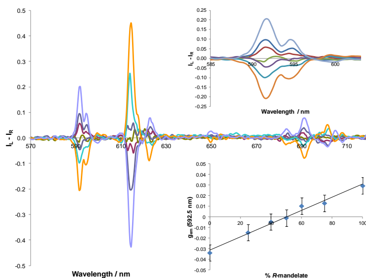
Figure 5 Changes in the CPL spectrum of [\text{Eu.L}^3]^+ following addition of mandelate of varying enantiomeric composition (10 \mu\text{M} , \lambda_{\text{exc}} = 352 nm, MeOH). Inset (top) shows the \Delta J=1 manifold; (bottom) variation of g_{\text{em}} (592.5 nm) with % R -mandelate; error bars indicate the standard deviation averaged over 5 runs ( R^2 0.98 for shown linear fit).
