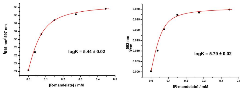
Figure 2 left: Variation of the ratio of two emission wavelengths vs. the concentration of mandelate; right: variation of the emission dissymmetry value g_{em} at 592 nm vs. concentration of mandelate. Experimental data fit to a 1:1 binding model following iterative least-squares fitting. (6 \mu M complex, \lambda_{exc} = 352 nm, MeOH, pH 5.5).
