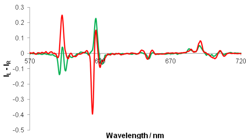
Figure 4 CPL spectra of [\text{Eu.L}^4]^+ following addition of R -phenylpropionic acid (green) and R -cyclohexylhydroxyacetic acid (red). ( \lambda_{\text{exc}} 348 nm, 2 mM anion, 5 \mu\text{M} complex, MeOH, pH 5.5, 295K).
