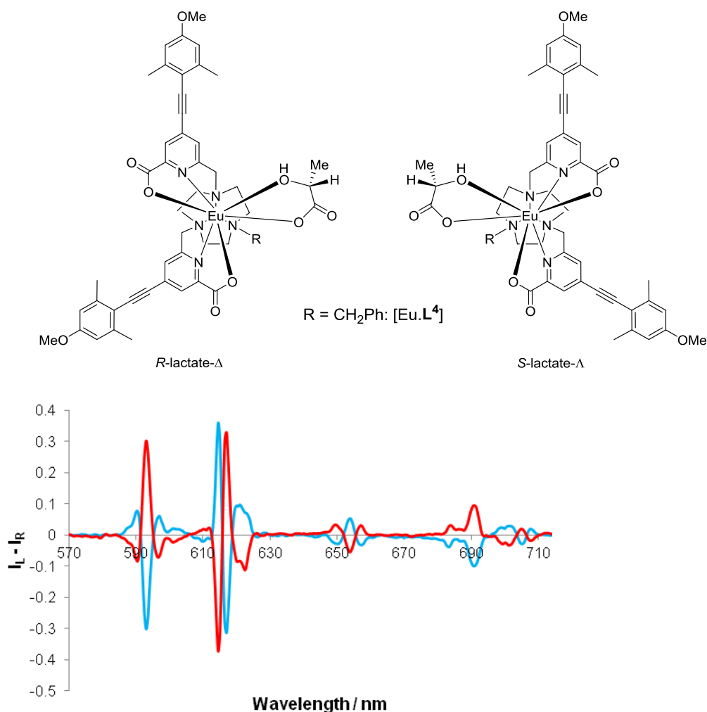
Figure 3 Mirror image CPL spectra of [\text{Eu.L}^4]^+ following addition of R -red and S -blue lactate ( \lambda_{\text{exc}} = 348 nm, 10 \mu\text{M} complex, 50 \mu\text{M} lactate, 295K, MeOH); ( upper ) showing the putative major isomers that gives rise to the observed CPL.
