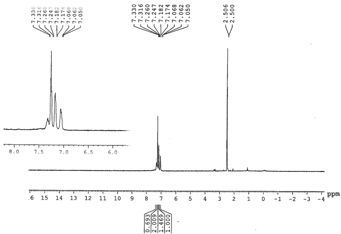
Figure S23: ^1\text{H} NMR (300 MHz, d_6 -DMSO) spectrum of complex [\text{Bi}(\text{BPHA})_3] 7
