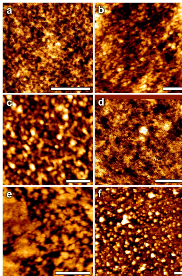
Figure 6 AFM height images of bismuth clusters dried onto mica substrates, where values refer to approximate cluster sizes obtained from analysis of the AFM image: a) \text{K}[\text{Bi}(\text{BHA})_2] 9 : 3.5 nm; b) [\text{Bi}(\text{BPHA})_3] 7 : 4 nm; c) [\text{Bi}(\text{H-SHA})_3] 1 : < 0.5 nm; d) [\text{Bi}(\text{AHA})(\text{H-AHA})] 5 : 5 nm; e) [\text{Bi}(\text{MFHA})_3] 3 : 1.8 nm; f) [\text{Bi}(\text{BHA})(\text{H-BHA})] 6 : < 0.5 nm. The white scale bar in each image represents 200 nm
