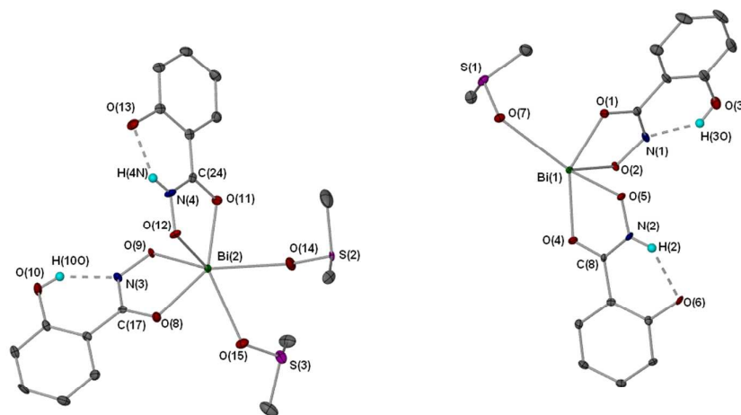
Figure 4 Molecular structure of \{[\text{Bi}(\text{SHA})(\text{H-SHA})(\text{DMSO})_2][\text{Bi}(\text{SHA})(\text{H-SHA})(\text{DMSO})]\cdot\text{DMSO}\}_\infty \cdot [\mathbf{4}(\text{DMSO})_{1.5}\cdot 0.5\text{DMSO}] . Only one of two independent molecules is shown; hydrogen atoms (except NH) and uncoordinated solvent molecules are omitted for clarity. Thermal ellipsoids at 40% probability. Selected bond lengths ( \text{\AA} ) and angles ( ^\circ ): Bi(2)-O(8), 2.346(3); Bi(2)-O(9), 2.268(3); Bi(2)-O(11), 2.284(3); Bi(2)-O(12), 2.231(3); Bi(2)-O(14), 2.748(3); Bi(2)-O(15), 2.710(6); N(3)-O(9), 1.382(4); N(3)-C(17), 1.319(5); N(4)-O(12), 1.390(4); N(4)-C(24), 1.297(5); C(17)-O(8), 1.275(5); C(24)-O(11), 1.288(5); O(13)-H(4N), 1.896(5); O(8)-Bi(2)-O(9), 69.79(10); O(11)-Bi(2)-O(12), 70.18(10).
