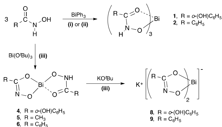
Scheme 1 Synthetic pathways to bismuth(III) hydroxamate complexes 1 , 2 , 4 – 6 , 8 , and 9 .
