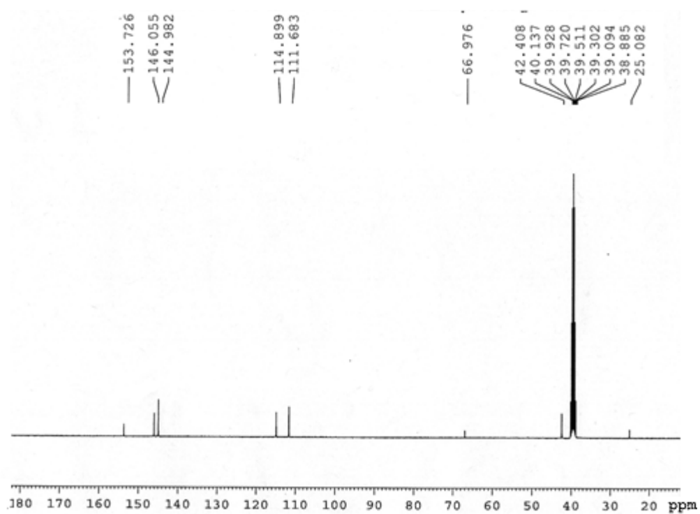
Figure 20: ^{13}\text{C} NMR (400 MHz, d_6 -DMSO) spectrum of complex [\text{Bi}(\text{MFHA})_3] 3
