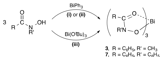
Scheme 2 Synthesis of bismuth(III) hydroxamate complexes 3 and 7 .
