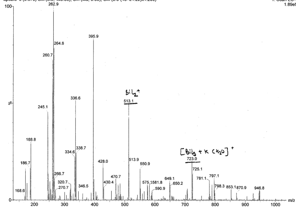
Figure S3: Mass-spectrum (ESI + ) of complex [\text{Bi}(\text{H-SHA})_3] \mathbf{1}
