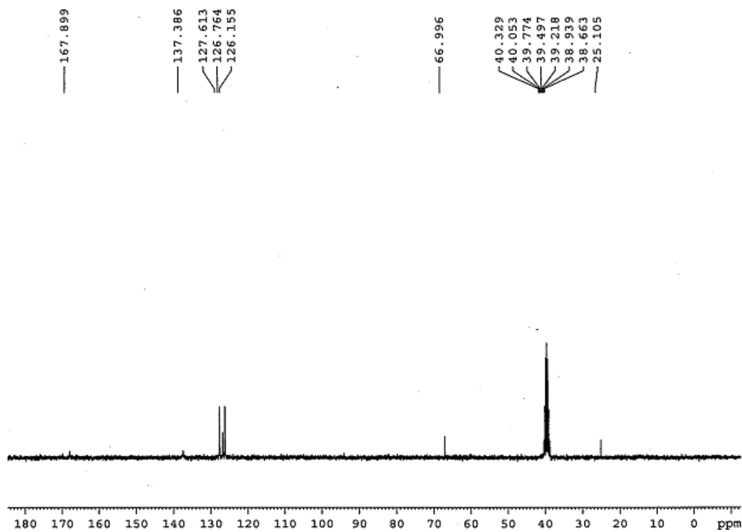
Figure S13: ^{13}\text{C} NMR (300 MHz, d_6 -DMSO) spectrum of complex \text{K}[\text{Bi}(\text{BHA})_2] \mathbf{9}
