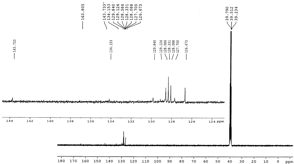
Figure S24: ^{13}\text{C} NMR (300 MHz, d_6 -DMSO) spectrum of [\text{Bi}(\text{BPHA})_3] 7
