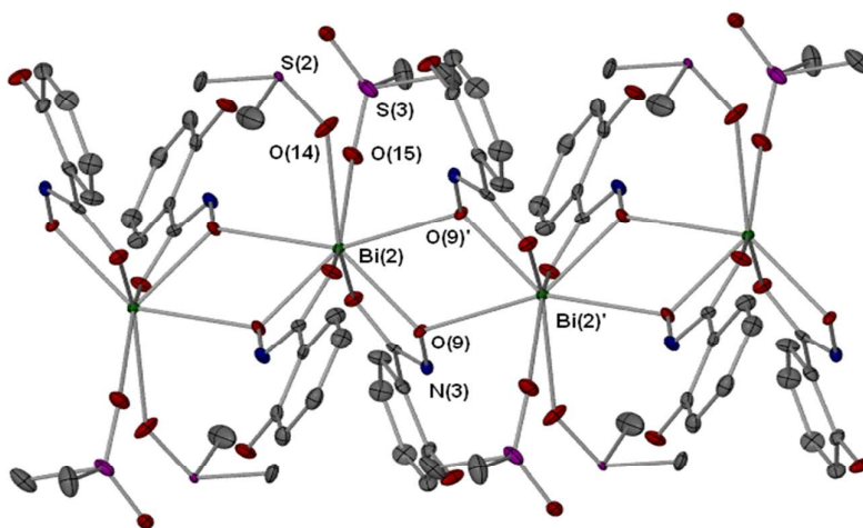
Figure 5 Extended polymeric section of [4(\text{DMSO})_{1.5} \cdot 0.5\text{DMSO}] with selected atom labeling. Symmetry operator ' :1-x, 2-y, 1-z. Selected bond lengths (Å) and angles (°): Bi(2)-O(9)' 2.605(3); Bi(2)-O(9)-Bi(2)', 112.77(6); O(9)-Bi(2)-O(9)', 67.23(8).
