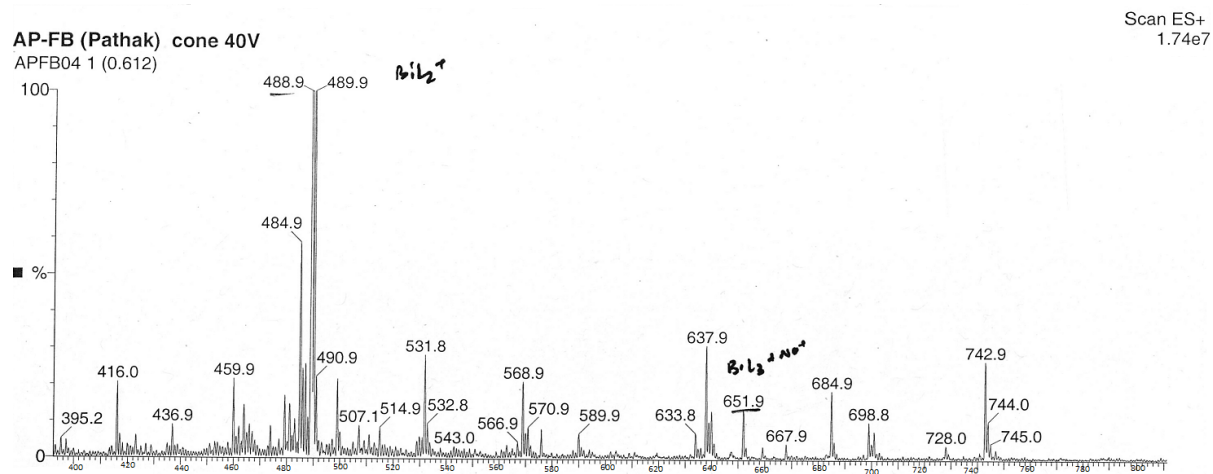
Figure S21: Mass-spectrum (ESI + ) of complex [Bi(MFHA) 3 ] 3
