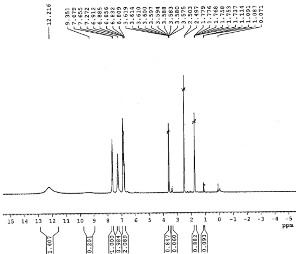
Figure S5: ^1\text{H} NMR (300 MHz, d_6 -DMSO) spectrum of complex \text{Bi}(\text{SHA})(\text{H-SHA})] \mathbf{4}
