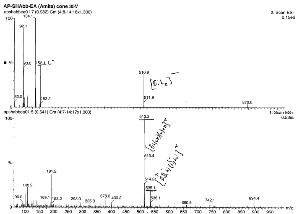
Figure S7: Mass-spectrum (ESI - ) and (ESI + ) of complex Bi(SHA)(H-SHA) 4
