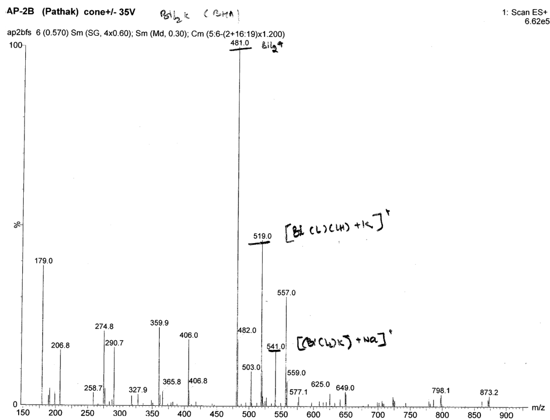
Figure S14: Mass-spectrum ( \text{ESI}^+ ) of complex \text{K}[\text{Bi}(\text{BHA})_2] \mathbf{9}
