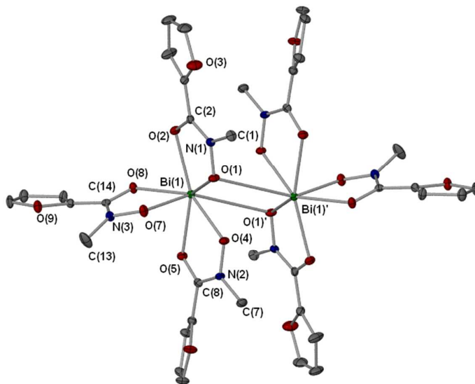
Figure 2 Molecular structure of {[Bi(MFHA) 3 ] 2 •Me 2 C=O} ( 3 •0.5Me 2 C=O) Only one of two independent molecules is shown; hydrogen atoms and uncoordinated solvent molecules are omitted for clarity. Thermal ellipsoids at 40% probability. Symmetry operator ' : 1-x, 2-y, 1-z. Selected bond lengths (Å) and angles (°): Bi(1)-O(1), 2.2586(15); Bi(1)-O(2), 2.4459(16); Bi(1)-O(4), 2.2918(15); Bi(1)-O(5), 2.4734(15); Bi(1)-O(7), 2.1747(16); Bi(1)-O(8), 2.4373(15); N(1)-O(1), 1.372(2); N(1)-C(2), 1.373(3); N(2)-O(4), 1.368(2); N(2)-C(8), 1.317(3); N(3)-O(7), 1.383(2); N(3)-C(14), 1.333(3); C(2)-O(2), 1.273(3); C(8)-O(5), 1.270(3); C(4)-O(8), 1.262(3); O(1)-Bi(1)-O(2), 67.48(5); O(4)-Bi(1)-O(5), 66.88(5); O(7)-Bi(1)-O(8), 69.31(5); Bi(1)-O(1)-Bi(1)', 81.28(8); O(1)-Bi(1)-O(1)', 98.72(9).
