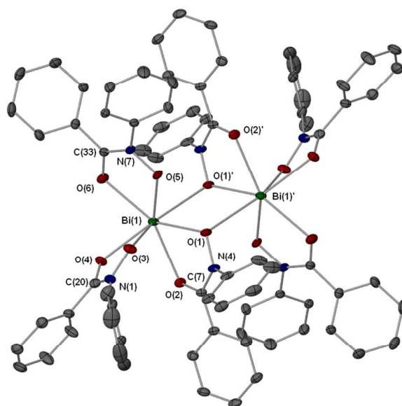
Figure 3 Molecular structure of \{[\text{Bi}(\text{BPHA})_3]_2 \cdot 2\text{EtOH}\} (\mathbf{7} \cdot \text{EtOH}) . Hydrogen atoms and uncoordinated solvent molecules are omitted for clarity. Thermal ellipsoids at 40% probability. Symmetry operator ' : -x, 1-y, -z . Selected bond lengths ( \text{\AA} ) and angles ( ^\circ ): Bi(1)-O(1), 2.2804(19); Bi(1)-O(2), 2.5151(18); Bi(1)-O(3), 2.195(2); Bi(1)-O(4), 2.4994(18); Bi(1)-O(5), 2.2364(17); Bi(1)-O(6), 2.474(2); Bi(1)-O(1'), 2.779(16); N(1)-O(3), 1.388(3); N(1)-C(20), 1.251(3); N(4)-O(1), 1.390(3); N(4)-C(7), 1.342(3); N(7)-O(5), 1.373(3); N(7)-C(33), 1.326(3); O(1)-Bi(1)-O(2), 66.07(6); O(3)-Bi(1)-O(4), 67.71(7); O(5)-Bi(1)-O(6), 68.00(6); O(1)-Bi(1)-O(1'), 72.30(6); Bi(1)-O(1)-Bi(1'), 107.70(8).
