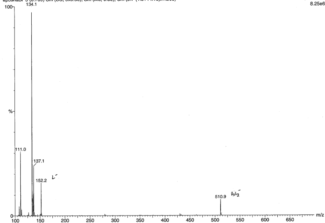
Figure S4: Mass-spectrum (ESI - ) of complex [\text{Bi}(\text{H-SHA})_3] \mathbf{1}
