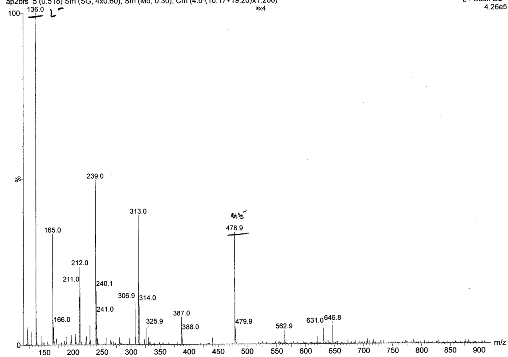
Figure S15: Mass-spectrum (ESI) of complex K[Bi(BHA)_2] 9
