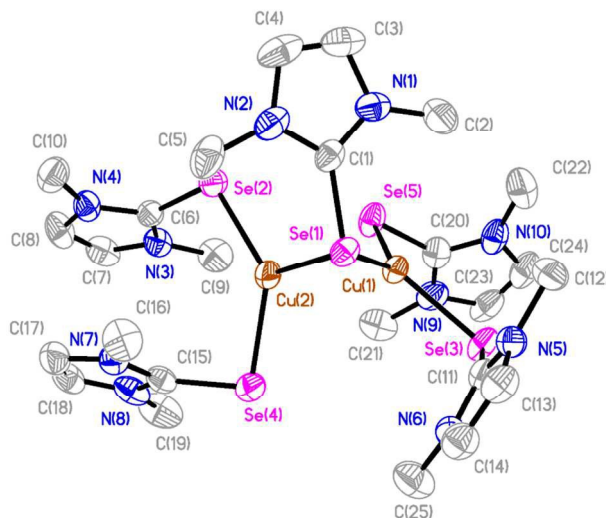
Fig. 2. The crystal structure diagram of the cation in [(\text{dmise})_2\text{Cu}(\mu\text{-dmise})\text{Cu}(\text{dmise})_2](\text{BF}_4)_2 \cdot \text{CH}_3\text{CN} ( 2 ) showing 50% probability ellipsoids. Hydrogen atoms, counterions, and the solvent molecules are omitted for clarity.
