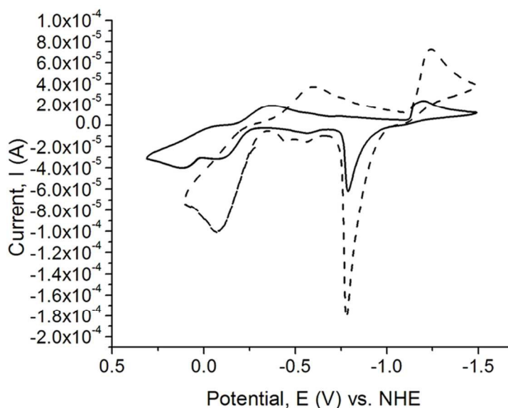
Fig. 9. Cyclic voltammetry (CV) scans for [(\text{dmit})_2\text{Cu}_2(\text{Bsem}^{\text{Me}})_2](\text{BF}_4)_2 ( 7 ) (solid line) and [(\text{dmise})_2\text{Cu}_2(\text{Bsem}^{\text{Me}})_2](\text{BF}_4)_2 ( 9 ) (dashed line). All data were collected with 1 mM compound in acetonitrile with n -butylammonium phosphate as the supporting electrolyte (0.1 M) at a scan rate of 100 mV/s.
