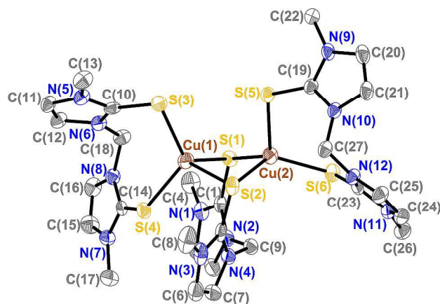
Fig. 3. The crystal structure diagram of the cation in [(\text{Bmm}^{\text{Me}})\text{Cu}(\mu\text{-Bmm}^{\text{Me}})\text{Cu}(\text{Bmm}^{\text{Me}})](\text{BF}_4)_2 ( 3 ) showing 50% probability ellipsoids. Hydrogen atoms and counterions are omitted for clarity.
