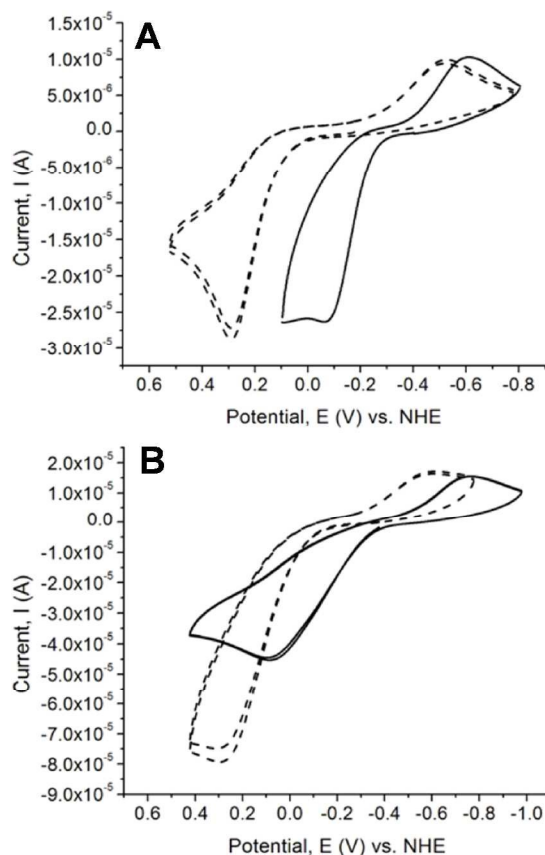
Fig. 8. Cyclic voltammetry (CV) scan for A) Bmm^{Me} (dashed lines) and Bsem^{Me} (solid lines), B) Bme^{Me} (dashed lines) and Bsee^{Me} (solid lines). All data were collected with 1 mM complex in acetonitrile.
