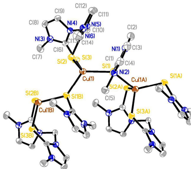
Fig. 7. Crystal structure diagram of the cationic portion of [(\text{Bmm}^{\text{Mc}})\text{Cu}(\mu\text{-dmit})]_n(\text{BF}_4)_n ( 10 ) showing three repeating units of the coordination polymer and 50% probability ellipsoids. Hydrogen atoms and counterions are omitted for clarity.
