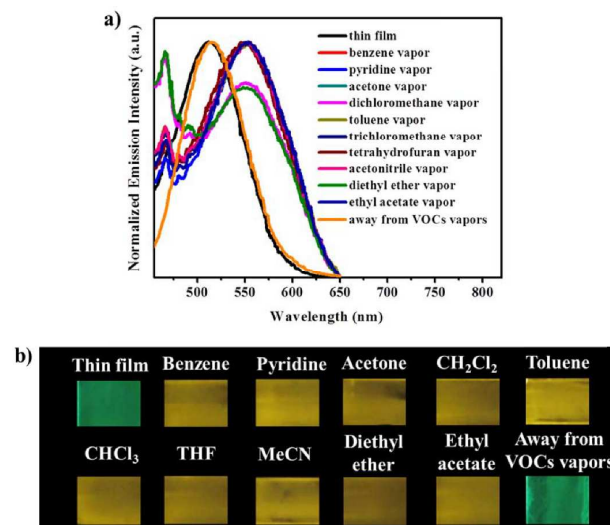
Fig. 5 a) Emission spectra changes of 1 thin film, exposing to VOCs vapors and away from VOCs vapors. Excitation wavelength: 365 nm; b) Photographic images of 1 thin film, upon exposure to vapors of VOCs and away from VOCs vapors under 365 nm UV light.
