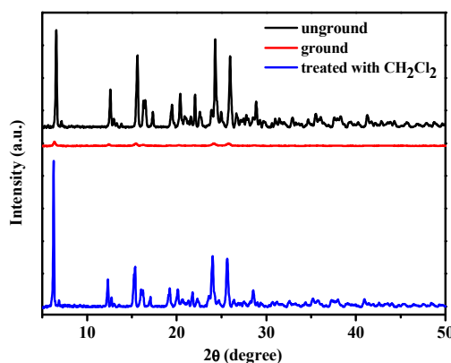
Fig. 2 XRD patterns of solid sample 1 : unground, ground and after treatment with dichloromethane vapor.
