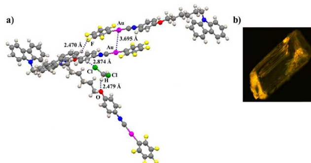
Fig. 6 a) The structural organization of single crystal with dichloromethane molecules of complex 1 ; b) Photographic image of yellow light-emitting crystal of 1 under 365 nm UV irradiation.
