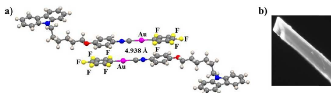
Fig. 3 (a) The structural organization of white light-emitting complex 1 ; (b) The fluorescence image of white light-emitting crystal of 1 under 365 nm UV irradiation.
