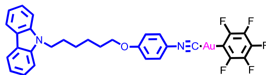
Scheme 1 The molecular structure of complex 1 .
