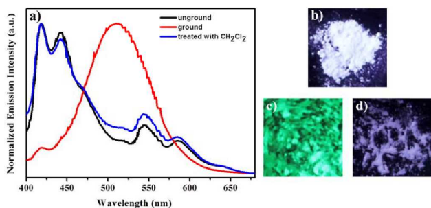
Fig. 1 (a) Luminescence spectra of unground solid sample 1 , after being ground and fumed with dichloromethane solvent vapor. The excitation wavelength is 365 nm. Fluorescence imaging of 1 taken under irradiation of a 365 nm UV light: (b) as-synthesized solid sample; (c) ground sample; (d) sample after treatment with dichloromethane vapor.
