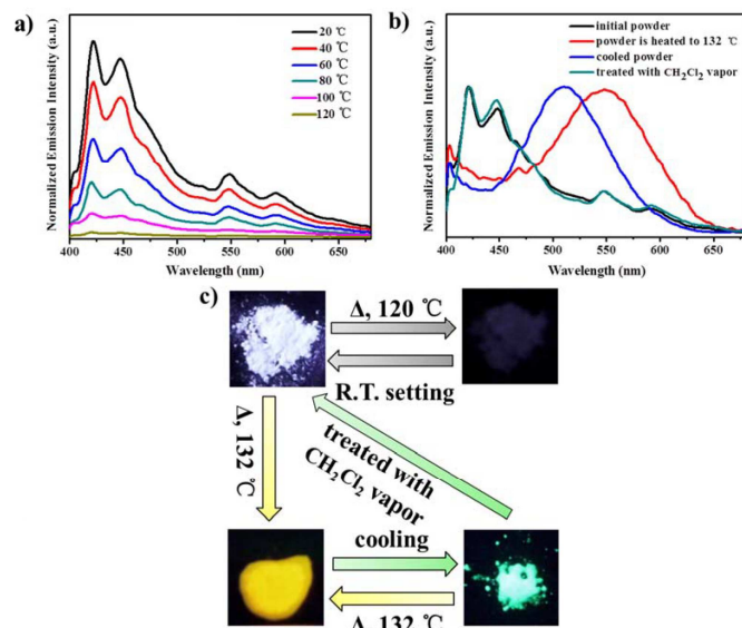
Fig. 4 a) PL spectra of luminogen 1 over a temperature range of 20–120 °C. Excitation wavelength: 365 nm. b) PL spectra of 1 initial powder, heated powder (132 °C), cooled powder and treated with CH 2 Cl 2 vapor. Excitation wavelength: 365 nm. c) The diagram of dual-responsive thermochromism behavior of 1 .
