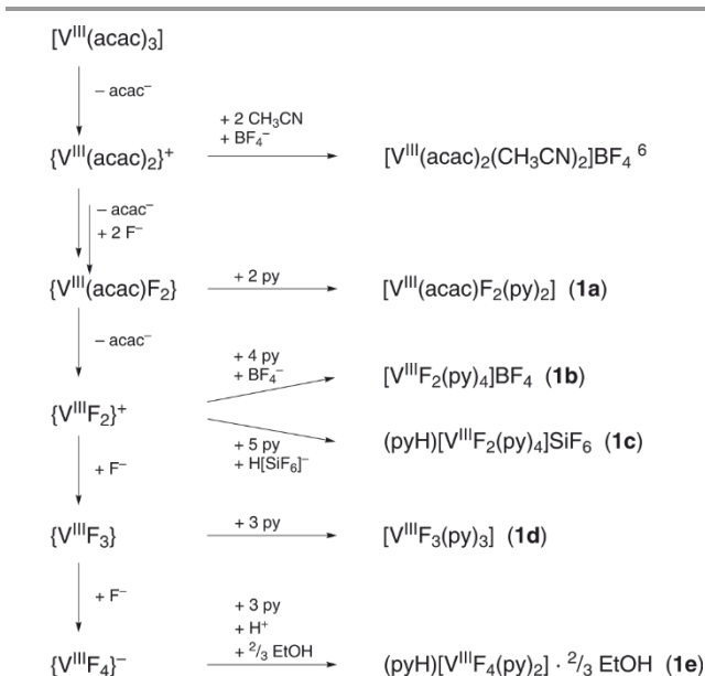
Scheme 2. Stepwise fluorination of [\text{V}(\text{acac})_3] and formation of the isolated complexes.
