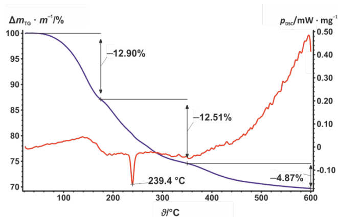
Fig. 3. TG/DSC during decomposition of the \text{Li}_3\text{VF}_6 precursor (synthesised in EtOH) in a dinitrogen atmosphere. Blue curve: TG signal, red curve: DSC signal, black arrows: mass changes. \Delta m_{\text{TG}} \cdot \text{m}^{-1}/\% : mass loss in per cent.
