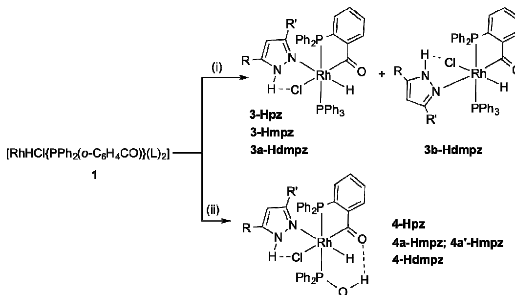
Scheme 3. In \text{CH}_2\text{Cl}_2 , 298 K. (i) \text{PPh}_3 : 3-Hpz , \text{R} = \text{R}' = \text{H} ; 3-Hmpz , \text{R} = \text{Me} , \text{R}' = \text{H} ; 3a-Hdmpz and 3b-Hdmpz , \text{R} = \text{R}' = \text{Me} . (ii) \text{PPh}_2(\text{O})\text{H} : 4-Hpz , \text{R} = \text{R}' = \text{H} ; 4a-Hmpz , \text{R} = \text{Me} , \text{R}' = \text{H} ; 4a'-Hmpz , \text{R} = \text{H} , \text{R}' = \text{Me} ; 4-Hdmpz , \text{R} = \text{R}' = \text{Me} .
