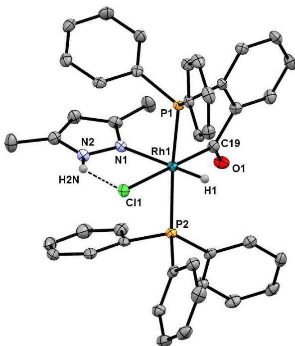
Figure 2. ORTEP view of 3a-Hdmpz showing the atomic numbering and the intramolecular hydrogen bond (30% probability ellipsoids). The hydrogen atoms except two have been omitted for clarity
