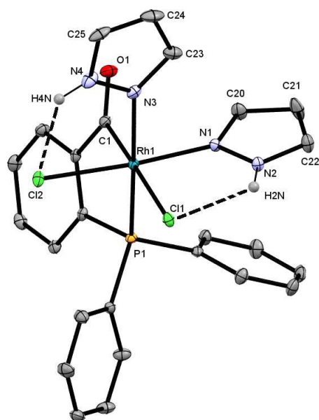
Figure 1. ORTEP view of 2-Hpz showing the atomic numbering and the intramolecular hydrogen bonds (30% probability ellipsoids). The hydrogen atoms except two have been omitted for clarity
