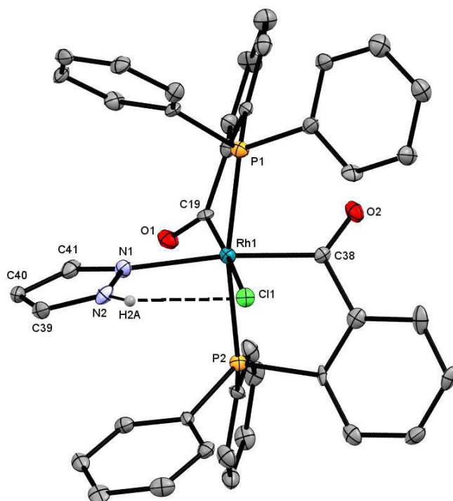
Figure 3. ORTEP view of 7-Hpz showing the atomic numbering and the intramolecular hydrogen bond (30% probability ellipsoids). The hydrogen atoms except one have been omitted for clarity
