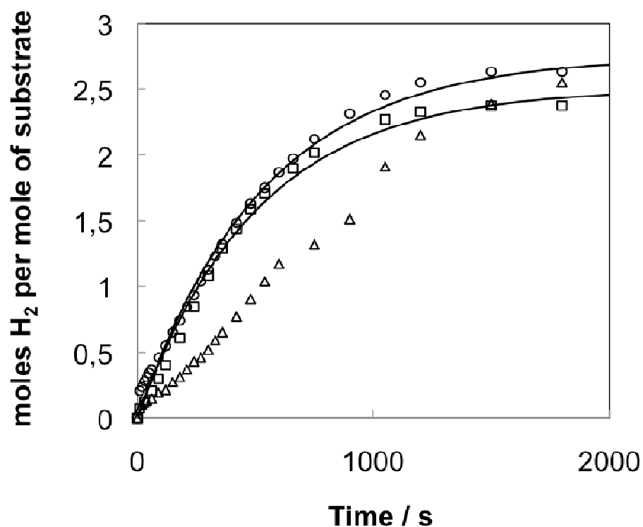
Figure 4. Hydrogen release from AB ( \circ ), TBAB ( \square ), or DMAB ( \triangle ) as substrates, with initial substrate concentration of 0.46 M, in the presence of 0.5 mol% of 1-Hdmpz as catalyst in THF/H 2 O mixtures. T, 298 K. Open marks represent the experimental points. Solid lines represent the regression line.
