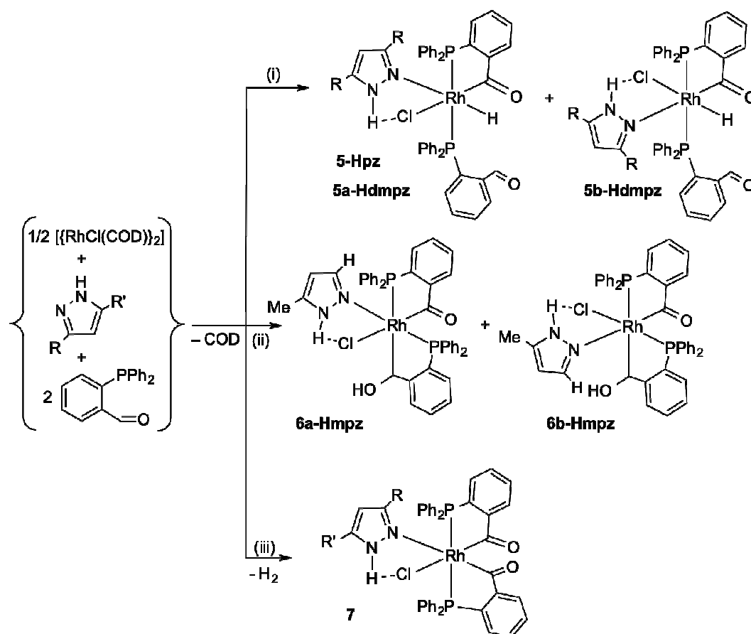
Scheme 4. (i) In \text{C}_6\text{H}_6 , 298K. 5-Hpz , R = R' = H; 5a-Hdmpz and 5b-Hdmpz , R = R' = \text{CH}_3 . (ii) In \text{C}_6\text{H}_6 , 353K, 5 min. (iii) In \text{C}_6\text{H}_6 , 353K, 90 min. 7-Hpz , R = R' = H; 7-Hmpz , R = H, R' = \text{CH}_3 ; 7-Hdmpz , R = R' = \text{CH}_3 .
