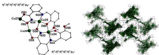
Figure 9 (left) The two distinct bonding modes exhibited by the L_1^{3-} ligands in [Cu 30 ] ( 5 ). (right) Packing of the crystals in 5 as viewed along the a cell direction. All hydrogen atoms and perchlorate counter anions have been omitted for clarity.
