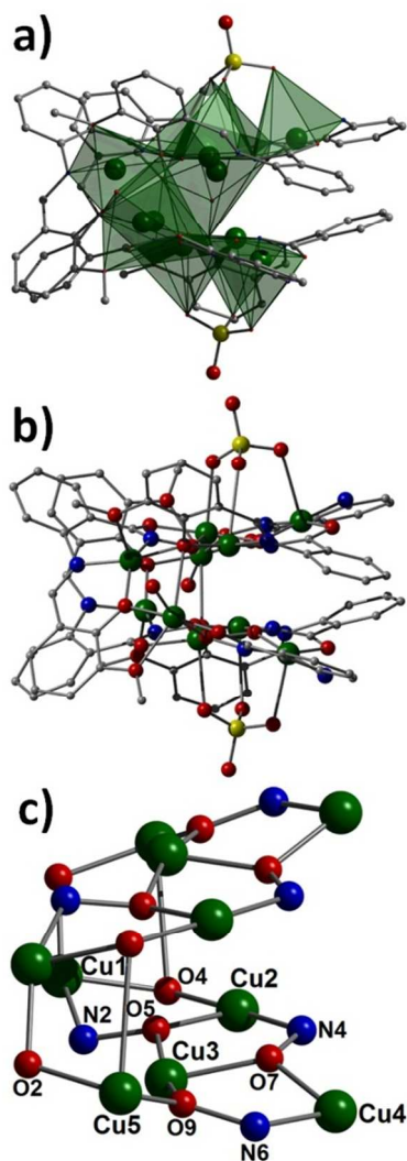
Figure 1 Polyhedral (a) and standard (b) representation of the crystal structure in 1. All hydrogen atoms have been omitted for clarity. (c) The
