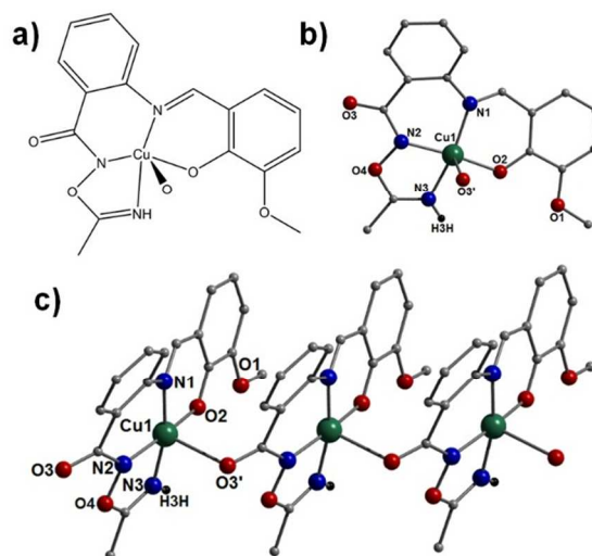
Figure 10 (a) ChemDraw representation and crystal structure (b) of one [Cu(II)(L 4 )] unit in 6 including the next bridging oxygen (O3') atom. (c) Representation of the repeating 1D structure in 6 (comprising three [Cu(II)(L 4 )] units). The majority of hydrogen atoms and all H 2 O solvents of crystallisation were omitted for clarity.
