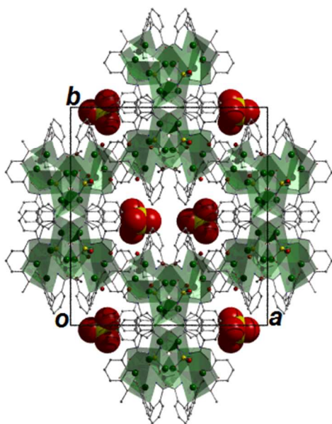
Figure 3 Crystal packing in 1 as viewed along the c unit cell direction. Note: Only the non-coordinated \text{ClO}_4^- counter anions are represented in space-fill mode. Hydrogen atoms have been omitted for clarity.
