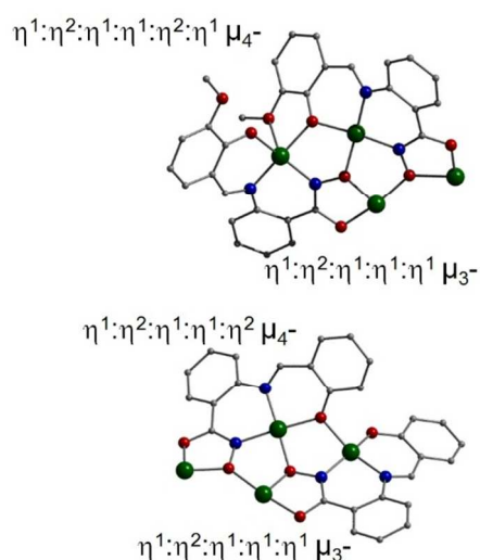
Figure 6 The two different bonding modes exhibited by the \text{L}_1^{3-} ligands in 2 (top) and \text{L}_3^{3-} ligands in 4 (bottom). All hydrogen atoms have been omitted for clarity.
