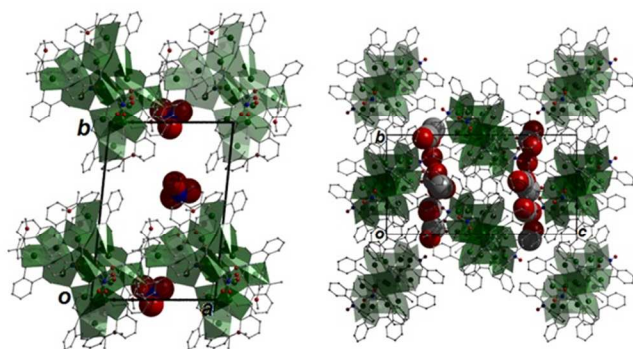
Figure 7 (Left) Polyhedral packing diagram of 2 as viewed along the c unit cell axis. Only the non-coordinating \text{NO}_3^- anions are shown in the space-fill mode. (Right) Polyhedral representation of the packing in 4 as viewed along the a axis of the unit cell. MeOH solvents of crystallisation are represented using the space-fill mode.
