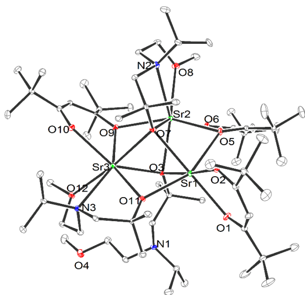
Figure 2. ORTEP diagram for complex 3 .
