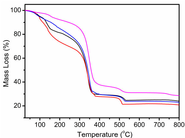
Figure 5. TGA plot of complexes 1 (black), 2 (red), 3 (blue), and 4 (violet).
