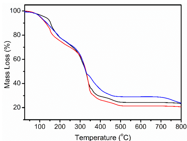
Figure 6. TGA plot of complexes 5 (black), 6 (red), and 7 (blue).
