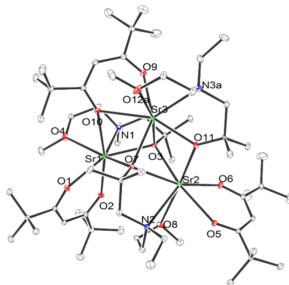
Figure 1. ORTEP diagram for complex 2.
