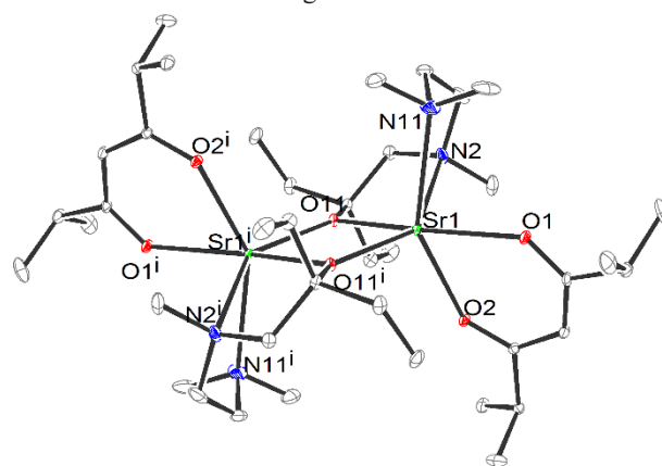
Figure 4. ORTEP diagram for complex 7 .
