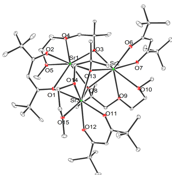
Figure 3. ORTEP diagram for complex 4 .
