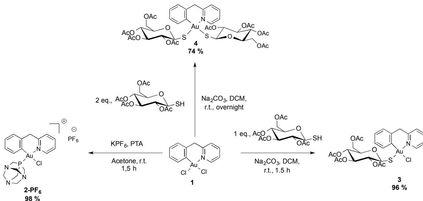
Scheme 1: Synthesis of novel (C N )gold(III) cyclometallated compounds.
