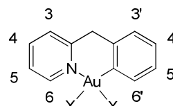
Scheme 2: 1 H and 13 C labelling used for the attribution of the NMR signals of the cyclometallated ligand.
