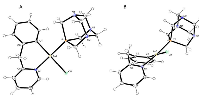
Figure 1 - ORTEP view of the cation in complex 2-PF 6 ; top (A) and side (B) views.
