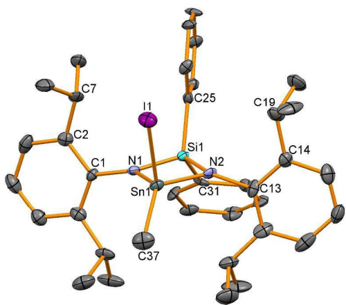
Figure 5. Molecular structure of 14 . All hydrogen atoms have been removed for clarity and thermal ellipsoids are set at 50% probability.
