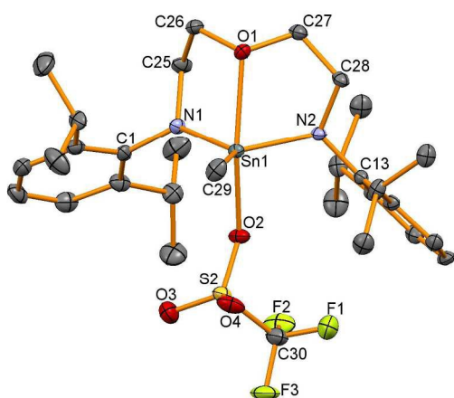
Figure 6. Molecular structure of 19 . All hydrogen atoms have been removed for clarity and thermal ellipsoids are set at 50% probability.
