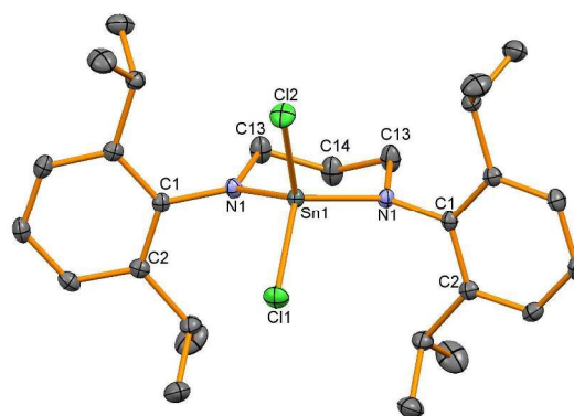
Figure 2. Molecular structure of 4 . Hydrogen atoms have been removed for clarity and thermal ellipsoids are set at 50% probability.
