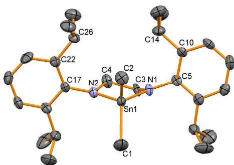
Figure 1. Molecular structure of 1 . Hydrogen atoms have been removed for clarity and thermal ellipsoids are set at 50% probability.
