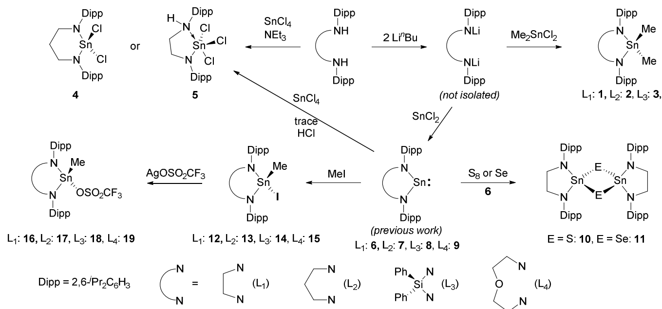
Scheme 1. Synthesis of tin compounds
