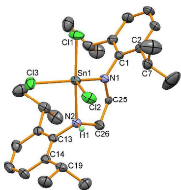
Figure 3. Molecular structure of 5 . All hydrogen atoms except the N-H have been removed for clarity and thermal ellipsoids are set at 50% probability.
