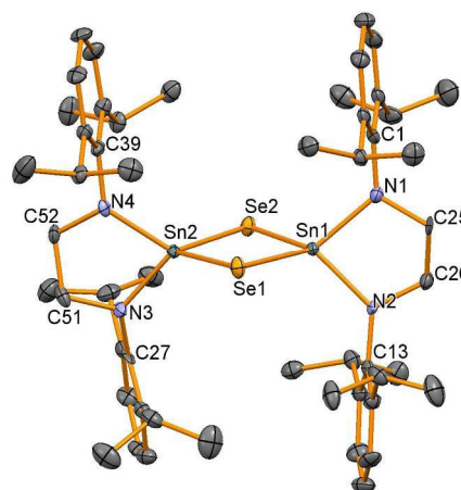
Figure 4. Molecular structure of 11 . All hydrogen atoms have been removed for clarity and thermal ellipsoids are set at 50% probability.
