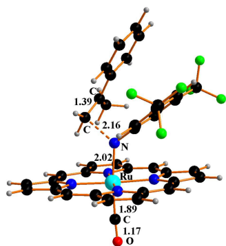
Figure 4. Structure of 5_{\text{TS}} resulting from the incipient interaction between the triplet imido complex \text{C}_T and \alpha -methylstyrene \text{Ph}(\text{Me})\text{C}=\text{CH}_2 .
