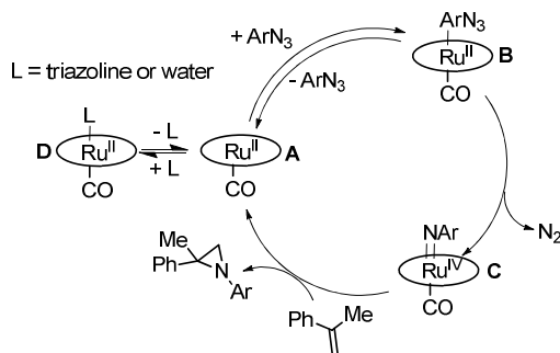
Scheme 3. Suggested mechanism for the aziridination of α-methylstyrene by aryl azide.
