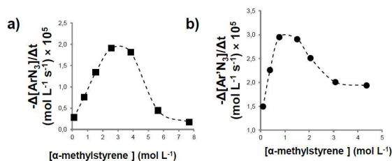
Figure 2. Dependence of the reaction rate with respect to \alpha -methylstyrene concentration for the aziridination by a) \text{ArN}_3 catalysed by 2a and b) \text{Ar}'\text{N}_3 catalysed by 2e .
