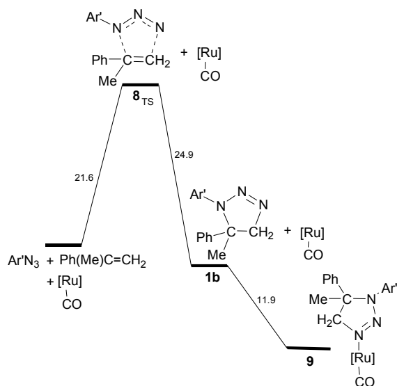
Scheme 6. Energy profile for the formation of triazoline 1b . The eventual coordination of 1b to [Ru](CO) is exergonic.
