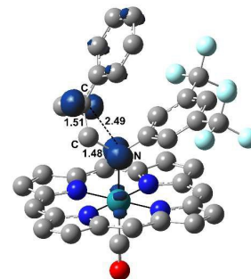
Figure 5. Structure of 6 T with the associated spin density shapes.
