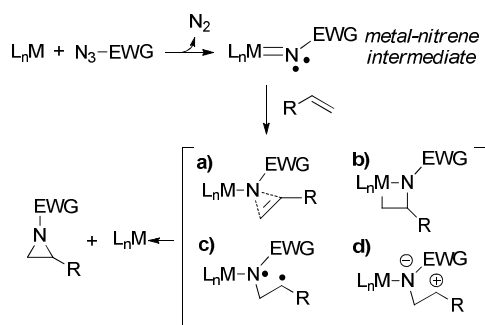
Scheme 1. Selection of possible pathways for the olefin aziridination by organic azides; a) concerted insertion, b) via azametallacyclobutane, c) stepwise radical reaction, d) stepwise carbocationic reaction.
