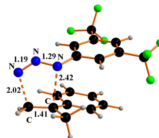
Figure 8. Optimised structure of 8 TS species in the 1,3-cycloaddition between Ar' 1 N 3 and α-methylstyrene.
