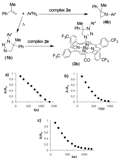
Figure 1. Kinetic dependence on \text{Ar}'\text{N}_3 using [\alpha\text{-methylstyrene}] = 0.1 \text{ M} (a), 2.1 \text{ M} (b) and 3.0 \text{ M} (c).
