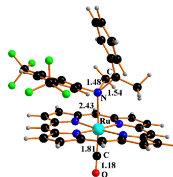
Figure 6. Structure of compound [\text{Ru}](\text{4b})(\text{CO}) 7 S .
