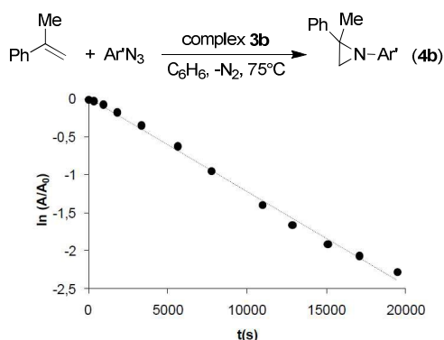
Figure 3. The Ar 1 N 3 consumption by using catalyst 3b and [α-methylstyrene] = 0.1 M
