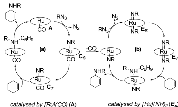
Scheme 4. Overall mechanism of the [Ru](CO)-catalysed allylic amination of cyclohexene by RN 3 .
