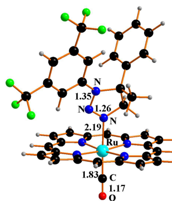
Figure 9. Optimised structure of complex 9 .
