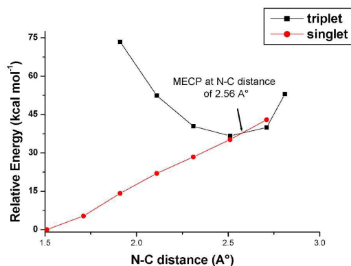
Figure 7. Relaxed scan plots over triplet and singlet Potential Energy Surface (Electronic energy) for the models 6 T and 7 S , derived from methyl azide and isobutene reactants.
