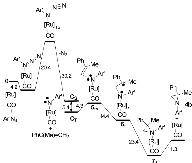
Scheme 5. The overall energy profile for the aziridine 4b synthesis from \text{Ar}^t\text{N}_3 and \alpha -methylstyrene, \text{Ph}(\text{Me})\text{C}=\text{CH}_2 .
