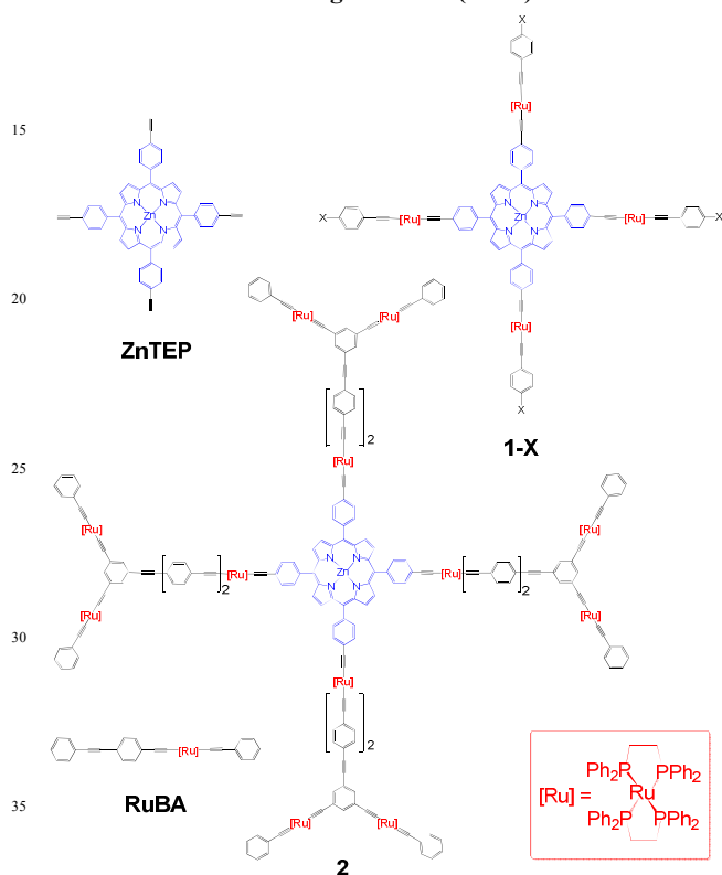
Scheme 1: Selected TPP-based molecules and the model complex RuBA.
