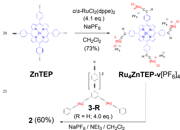
Scheme 2: Synthesis of compound 2 .
