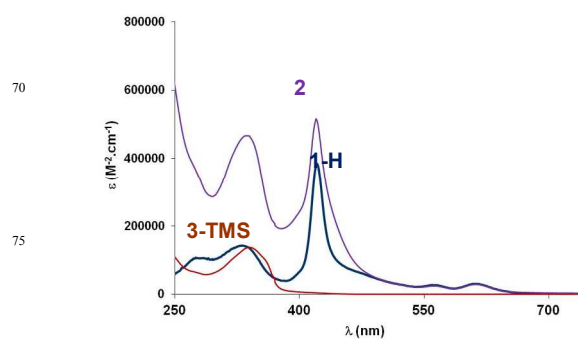
Figure 1: UV-Vis absorption spectra of the zinc porphyrins 1-H , 2 and of the wedge model 3-TMS in \text{CH}_2\text{Cl}_2 at 25 °C.
