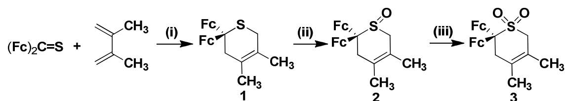
Scheme 1. Synthesis of 1 – 3 (MCPBA = m -chloroperoxybenzoic acid, Fc = ferrocenyl group). (i) 75 °C, 50 h; (ii) 30 % H 2 O 2 , SeO 2 , CH 3 OH, 0 °C to r.t., 10 min; (iii) MCPBA, CH 2 Cl 2 , -20 °C, 2 h, then r.t. 24 h and 2 nd portion MCPBA at r.t. 24 h.
