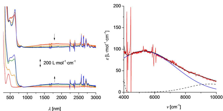
Figure 8. Left: UV-Vis/NIR spectra of 3 at 25 °C in dichloromethane (2.0 mmol·L -1 ) at rising potentials (bottom: -200 to 375 mV; top: 375 to 1200 mV vs Ag/AgCl); supporting electrolyte [Bu 4 N][B(C 6 F 5 ) 4 ]. Right: Deconvolution of the NIR absorptions of 3 + using three Gaussian shaped bands determined by spectroelectrochemistry in an OTTLE cell.
