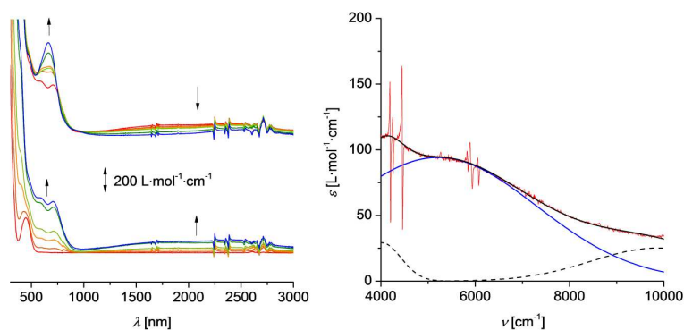
Figure 6. Left: UV-Vis/NIR spectra of 1 at 25 °C in dichloromethane (2.0 mmol·L -1 ) at rising potentials (bottom: -200 to 475 mV; top: 475 to 1200 mV vs Ag/AgCl); supporting electrolyte [Bu 4 N][B(C 6 F 5 ) 4 ]. Right: Deconvolution of the NIR absorptions of 1 + using three Gaussian shaped bands determined by spectroelectrochemistry in an OTTLE cell.
