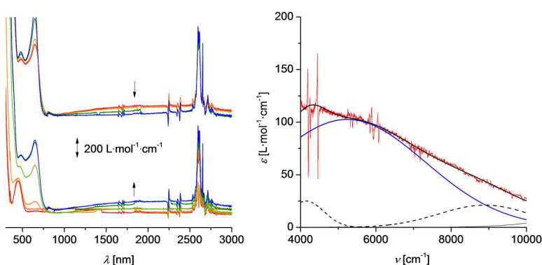
Figure 7. Left: UV-Vis/NIR spectra of 2 at 25 °C in dichloromethane (2.0 mmol·L -1 ) at rising potentials (bottom: -200 to 375 mV; top: 375 to 1200 mV vs Ag/AgCl); supporting electrolyte [Bu 4 N][B(C 6 F 5 ) 4 ]. Right: Deconvolution of the NIR absorptions of 2 + using three Gaussian shaped bands determined by spectroelectrochemistry in an OTTLE cell.
