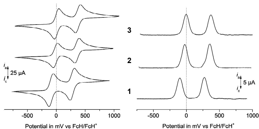
Figure 5. Left: Cyclic voltammograms of 1 – 3 , scan rate: 100 \text{ mV} \cdot \text{s}^{-1} . Right: Square wave voltammograms of 1 – 3 in dichloromethane solutions ( 1.0 \text{ mmol} \cdot \text{L}^{-1} ) at 25 \text{ }^\circ\text{C} , supporting electrolyte 0.1 \text{ mol} \cdot \text{L}^{-1} [\text{Bu}_4\text{N}][\text{B}(\text{C}_6\text{F}_5)_4] , working electrode: glassy carbon electrode (surface area 0.031 \text{ cm}^2 ).
