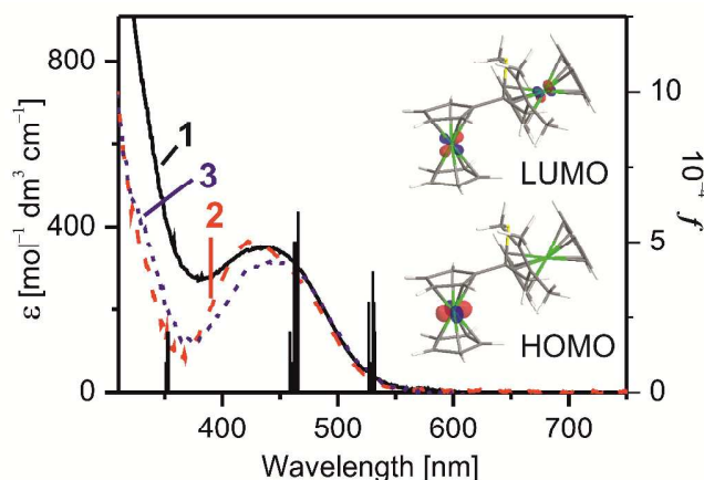
Figure 3. UV-Vis absorption spectra of 1 – 3 in dichloromethane at ambient temperature ( 1 : black solid line; 2 : red dashed line; 3 : blue dotted line) and TD-DFT calculated electronic transitions for 1 (vertical bars; oscillator strengths are given on the y axis (right)). Contour plots of the frontier orbitals HOMO and LUMO for 1 .
