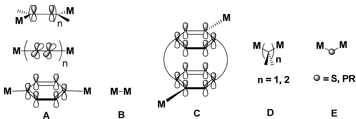
Figure 1. Classification of homobimetallic mixed-valence (= MV) metal complexes. M represents a metal containing redox centre. In type A molecules the centres are connected by a conjugated bridge consisting of C, C double or triple bonds, or aromatic moieties. 5,6 In type B molecules the M termini are directly connected to each other, 36 while in type D and E species the metal centres are separated by an aliphatic 37,38 or heteroatom fragment, respectively. 37-39 Type C molecules represent a special variety of type A compounds, in which the two M termini in the mixed-valent species interact most likely "through space". 34
