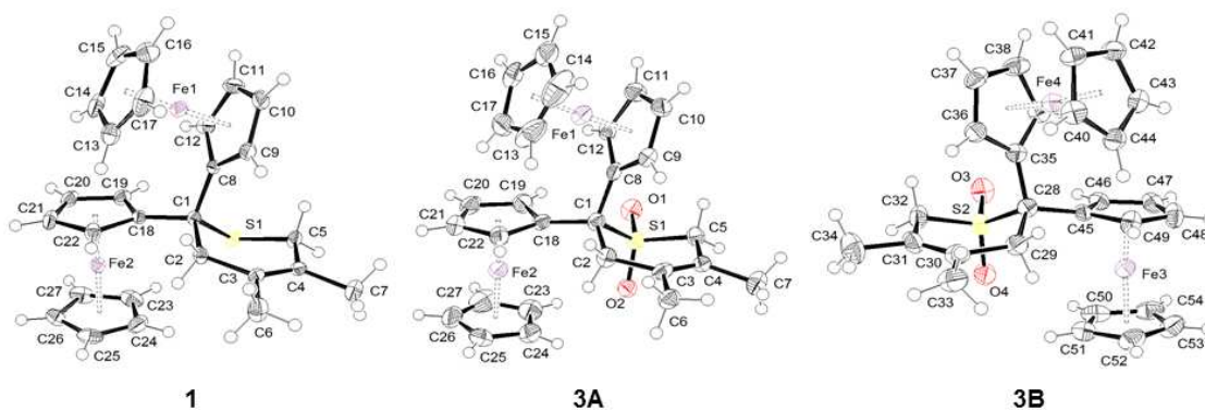
Figure 2. ORTEP diagrams of 1 and 3 (two independent molecules in the crystal, 3A and 3B ) at 50 % probability level.
