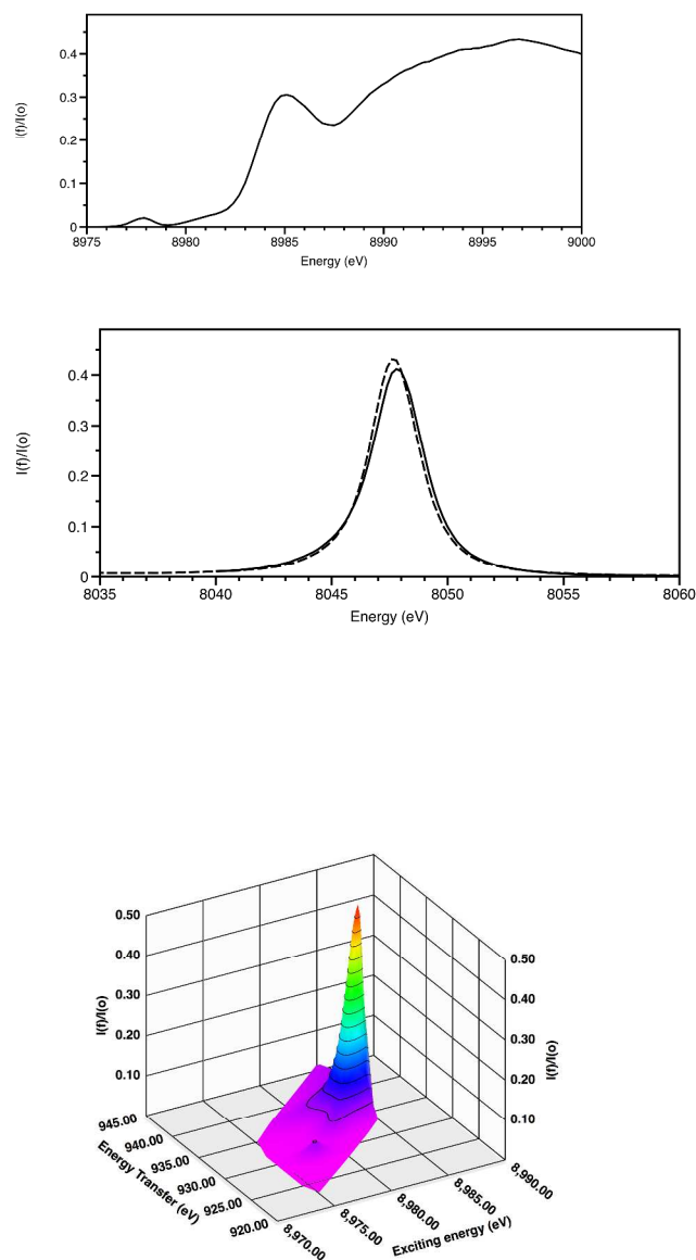
Fig 2 Cu K-edge XANES of CuO showing the HERFD spectrum (top), K \alpha_1 emission spectra of CuO (solid) and Cu (dashed) with the exciting energy above the absorption edge (middle) and K \alpha_1 RIXS (bottom). Energy transfer = Exciting energy – emission energy. Data recorded on I20 of the Diamond Light Source.
