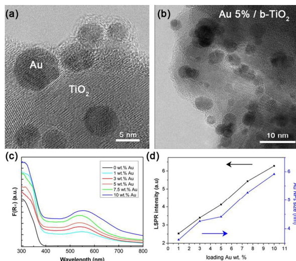
Figure 3. HRTEM image showing the sharp interface formed between Au NPs and (a) w- and (b) b-TiO 2 . (c) UV-vis absorption spectra of the x%Au/w-TiO 2 samples. (d) Effect of Au loading on LSPR intensity and Au NPs size for w-TiO 2 .
