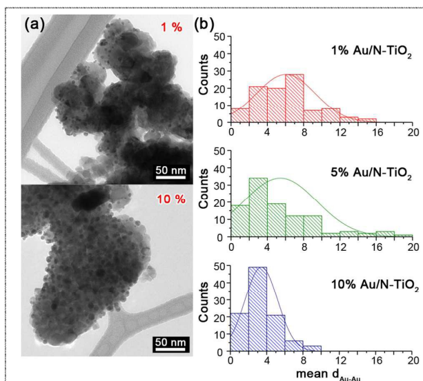
Figure 5. TEM images showing the increased Au NPs density for 1% and 10 % Au/N-TiO 2 samples. (b) Mean Au inter-particles distance ( d_{Au-Au} ) determined from the TEM images of the three representative samples 1, 5 and 10% Au/N-TiO 2 .
