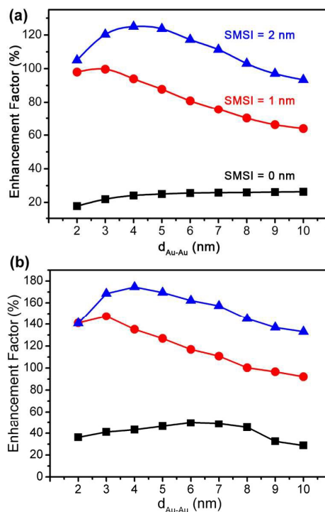
Figure 8. Photocatalytic Enhancement factor of the plasmon-generated electric field for d_{\text{Au}} = 6 \text{ nm} diameter as a function of Au interparticles distance ( d_{\text{Au-Au}} ) at SMSI=0 nm (black line), SMSI=1 nm (red line), SMSI=2 nm (blue line) for w- \text{TiO}_2 (a) and N- \text{TiO}_2 catalysts (b).
