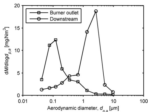
Fig. 4 Mass based size distributions obtained during injection of a 0.1 M KCl solution at 420 mL/h at the burner outlet (flue gas temperature = 1075 °C) as well as downstream the burner (flue gas temperature = 550 °C).
