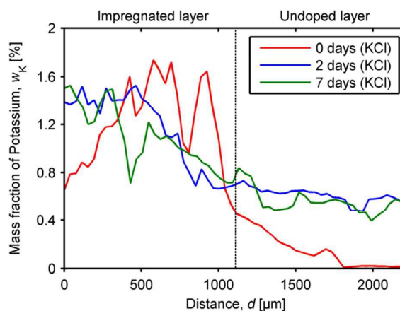
Fig. 9 Potassium profiles in KCl impregnated (1.6 wt.% K, nominal) two-layer pellets of 3%V 2 O 5 -WO 3 /TiO 2 catalyst, exposed to a flow (1000 NmL/min) of 6 vol.% O 2 and 3 vol.% H 2 O in N 2 at 350 °C for 0-7 days.
