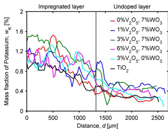
Fig. 14 Potassium profiles in KCl impregnated (1.6 wt.% K, nominal) two-layer pellets of \text{V}_2\text{O}_5 - (\text{WO}_3)/\text{TiO}_2 catalysts, exposed to a flow (1000 NmL/min) of 6 vol.% \text{O}_2 and 3 vol.% \text{H}_2\text{O} in \text{N}_2 at 350 °C for 7 days.
