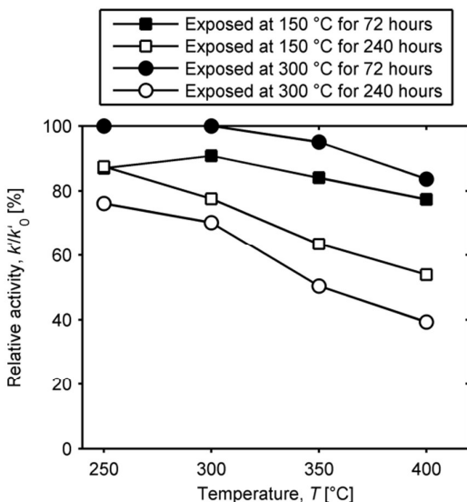
Fig. 7 Relative catalytic activities of K 2 SO 4 exposed 3%V 2 O 5 -7%WO 3 /TiO 2 catalysts as functions of temperature. Measurement conditions: [NO] = 500 ppmv, [NH 3 ] = 600 ppmv, [O 2 ] = 5 vol.%, [H 2 O] ≈ 1.4 vol.%, balance N 2 . Total flow = 2800 mL/min.
