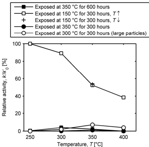
Fig. 6 Relative catalytic activities of KCl exposed 3%V 2 O 5 -7%WO 3 /TiO 2 catalysts as functions of temperature. Measurement conditions: [NO] = 500 ppmv, [NH 3 ] = 600 ppmv, [O 2 ] = 5 vol.%, [H 2 O] ≈ 1.4 vol.%, balance N 2 . Total flow = 2800 mL/min.
