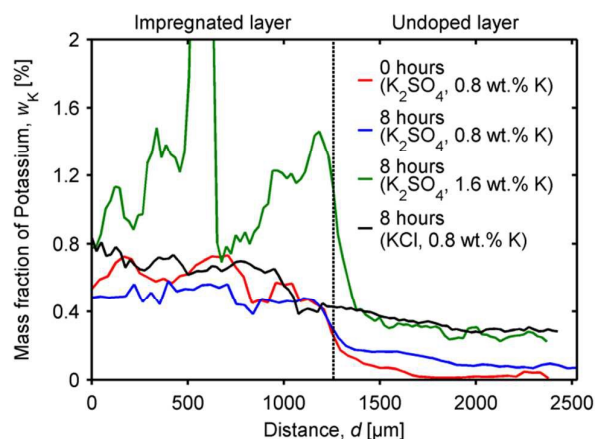
Fig. 12 Potassium profiles in K 2 SO 4 or KCl impregnated (0.8-1.6 wt.% K, nominal) two-layer pellets of 3%V 2 O 5 -WO 3 /TiO 2 catalyst, exposed to a flow (1000 NmL/min) of 6 vol.% O 2 and 3 vol.% H 2 O in N 2 at 350 °C for 0-8 hours.
