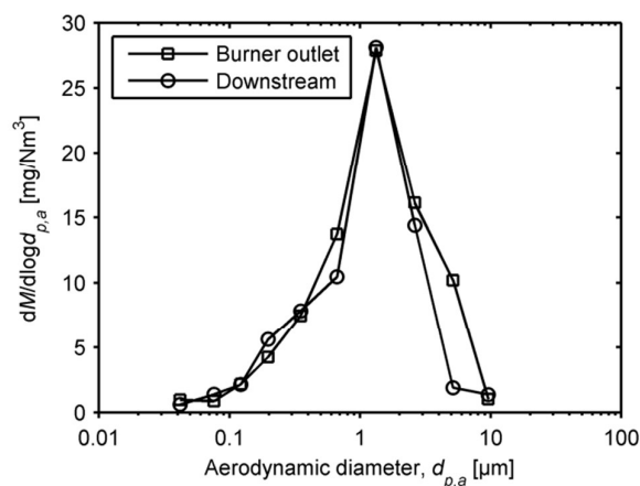
Fig. 5 Mass based size distributions obtained during injection of a 0.05 M K 2 SO 4 solution at 420 mL/h at the burner outlet (flue gas temperature = 1075 °C) as well as downstream the burner (flue gas temperature = 550 °C).
