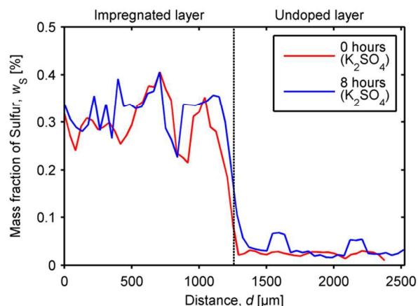
Fig. 13 Sulfur profiles in K 2 SO 4 impregnated (0.8 wt.% K, nominal) two-layer pellets of 3%V 2 O 5 -WO 3 /TiO 2 catalyst, exposed to a flow (1000 NmL/min) of 6 vol.% O 2 and 3 vol.% H 2 O in N 2 at 350 °C for 0-8 hours.
