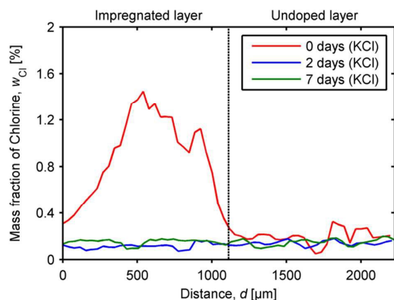
Fig. 10 Chlorine profiles in KCl impregnated (1.6 wt.% K, nominal) two-layer pellets of 3%V 2 O 5 -WO 3 /TiO 2 catalyst, exposed to a flow (1000 NmL/min) of 6 vol.% O 2 and 3 vol.% H 2 O in N 2 at 350 °C for 0-7 days.
