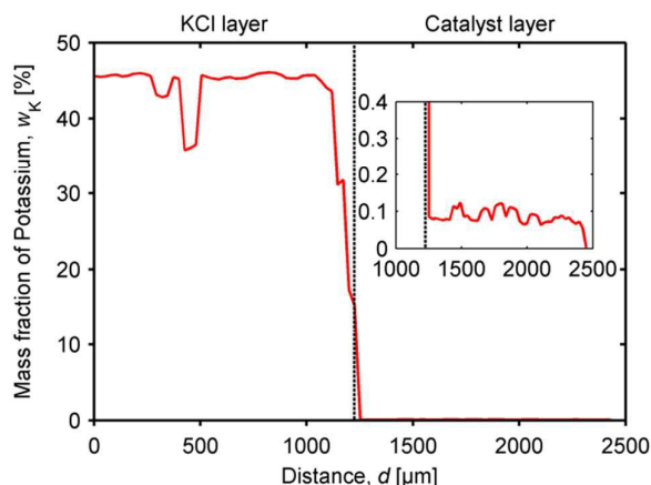
Fig. 11 Potassium profile in a two-layer pellet containing a layer of pure KCl and a layer of a 3%V 2 O 5 -7WO 3 /TiO 2 catalyst, exposed to a flow (1000 NmL/min) of 6 vol.% O 2 and 3 vol.% H 2 O in N 2 at 350 °C for 7 days.
