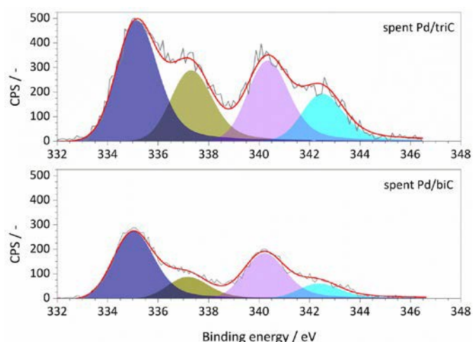
Fig. 5 Pd 3d core level XPS spectra of the spent Pd/triC and Pd/biC catalysts.
