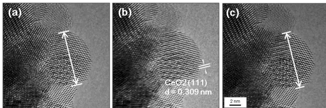
Fig. 10: A sequence of time resolved dynamic real time observations in CO+ water (WGS) mixture up to 350°C showing essentially stable bulk ceria (the same area of the sample); (a) after 1.1 sec ; (b) 9.9 sec and (c) 55 secs. The images reveal evolution of Au clusters of 0.3 nm in ceria grains). Sintering and bulk grain growth of ceria were not discernible even after several hours. Au species are discernible.
