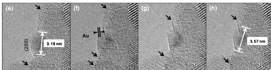
Fig. 9 (e-h): Dynamic real time visualisation of the movement of several gold atoms and Au clusters towards the gold nanoparticle (NP) and the growth of the NP are shown in e-h, leading to the decrease of Au surface atoms and Au clusters. Au (200) planar spacing is indicated. Time resolved atomic images taken from video sequences are, after : (e) 0.4 sec; (f) 21 sec; (g) 65 sec ; and (h) 95 sec.
