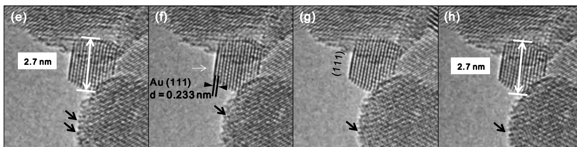
Fig. 12 e-h: Dynamic Au/ceria catalyst in CO+H 2 O environment (WGS) shows faceted gold single crystal NP in [110] with atomically clean {111} surfaces. The NP stops sintering, suggesting a lower surface energy configuration is reached. Time resolved real time ETEM atomic images in WGS video sequences: after (e) 6.8 sec; (f) 8.35 sec; (g) 14.3 sec and (h) 37 sec. Once this lower energy configuration is achieved Au NPs do not grow even after a long
