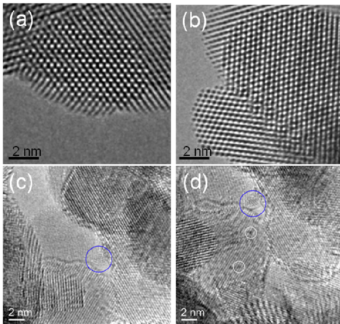
Fig. 7 a,b: In-situ real time ETEM experimental observations of gold/ceria catalyst in [110] orientation: (a) Au clusters were not observed in CO; and in CO/N 2 shown in (b);
