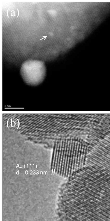
Figure 12 a,b. Dynamic sintering and faceting of gold NPs in WGS reaction, in real time: a , ESTEM showing a large sintered Au NP. (A few small (0.3nm) Au clusters are still visible in the image -arrowed). Au clusters sinter into NPs. b , [110] Au single crystal NP with atomically clean {111} facets (surfaces) in CO+ water in wet ETEM. The NP growth appears to cease in CO+H 2 O indicating a lower surface energy configuration for the NP shown below.
