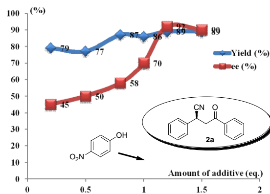
Figure 1. The effect of para -nitrophenol (PNP) on the catalytic asymmetric conjugate addition of cyanide to chalcone 1a .
