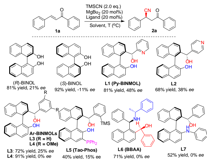
Scheme 1. Catalytic asymmetric conjugate hydrocyanation of chalcone with TMSCN
