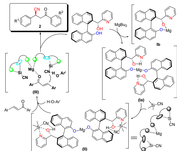
Scheme 2. Proposed mechanism for Py-BINMOL-Mg catalysed hydrocyanation
