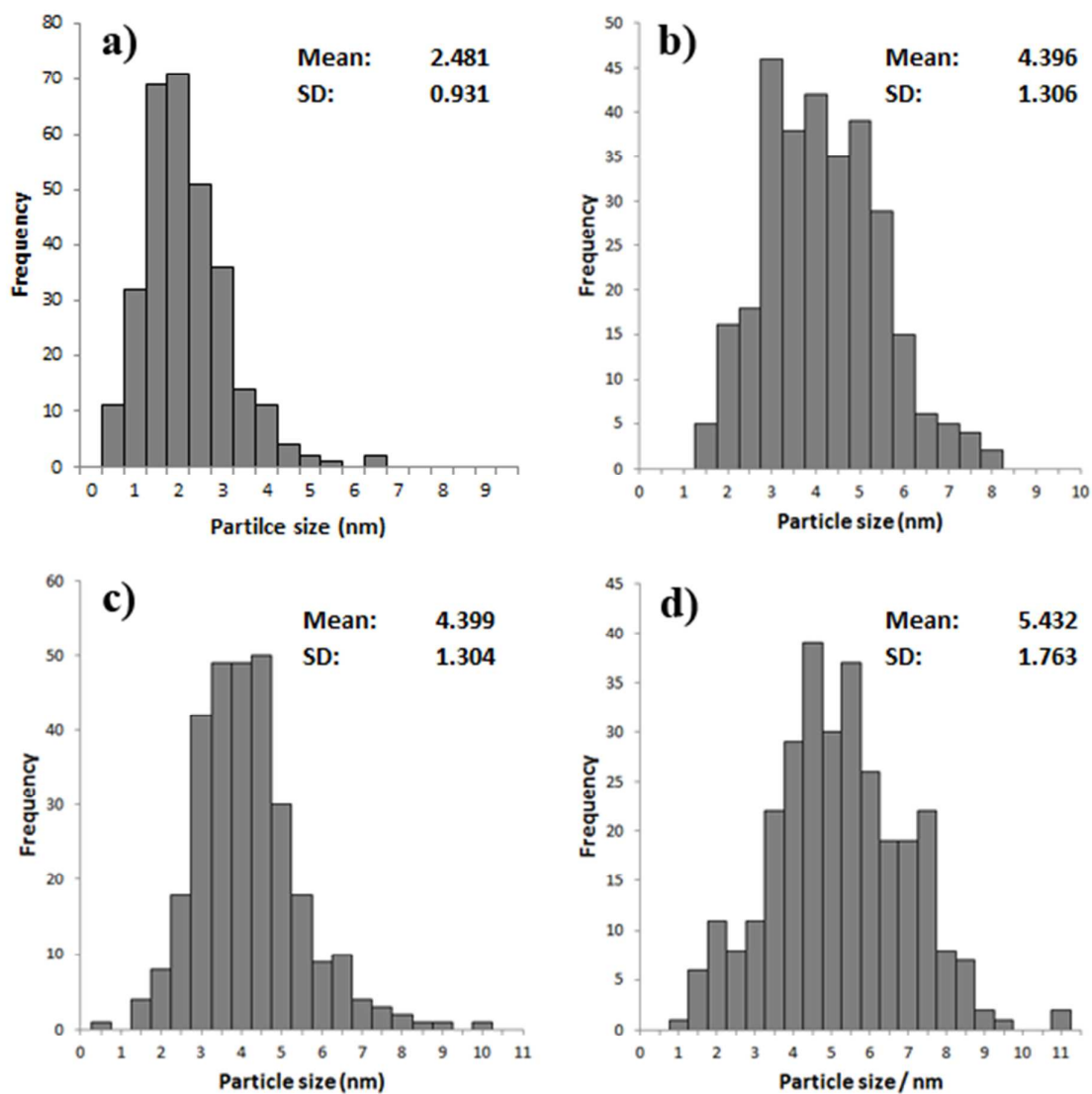
Figure 7: Particle size distribution for %Au/TiO 2 SIM calcined at a) 250 °C, b) 350 °C, c) 450 °C and 550 °C.
