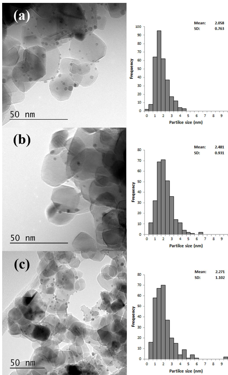
Figure 4 Representative TEM images and associated particle size distributions for 1%Au/TiO 2 prepared by SIM a) no treatment, b) calcined at 250 °C and c) refluxed. Particle size distributions based on 300 particles.
