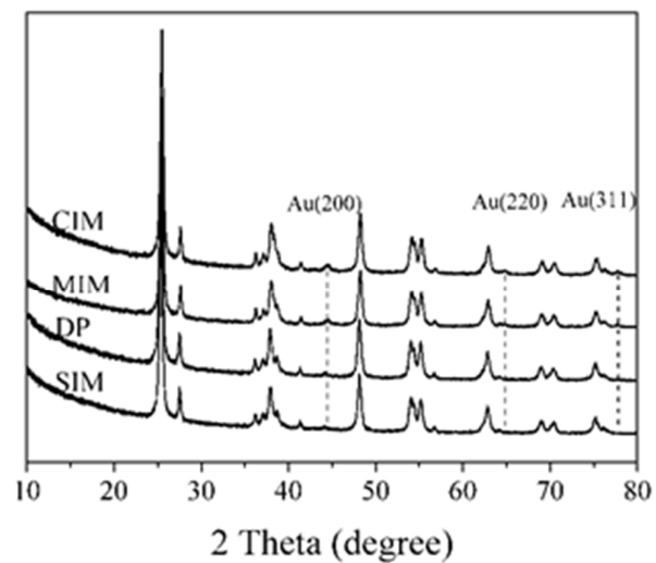
Figure 1 XRD pattern of 1%Au/TiO 2 catalysts prepared with different methods
