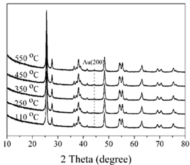
Figure 5 XRD patterns of 1%Au/TiO 2 catalysts calcined at different temperatures
