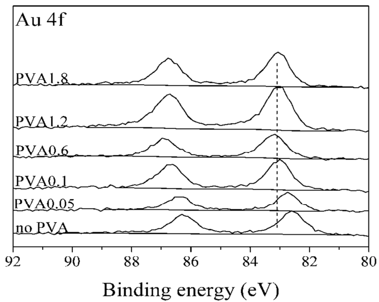
Figure 8 Au(4f) spectra for 1%Au/TiO 2 SIM samples prepared with different ratio of PVA to Au (w/w)
