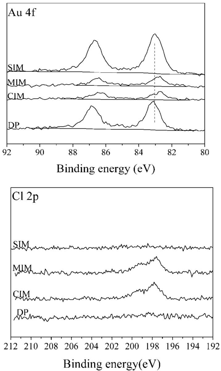
Figure 3 Au(4f) and Cl(2p) spectra for 1%Au/TiO 2 samples prepared by different methods
