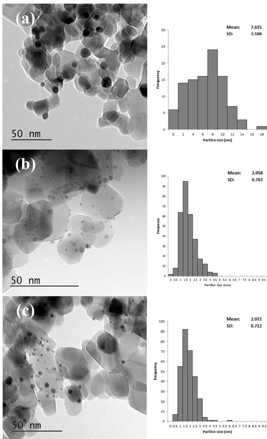
Figure 9 Representative TEM images and associated particle size distributions for 1%Au/TiO 2 prepared by SIM with different PVA: Au ratios a) 0.1, b) 1.2 and c) 1.8. Particle size distributions based on 300 particles except for a) where 100 particles were counted.
