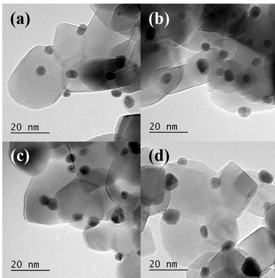
Figure 6. Representative TEM images of 1%Au/TiO 2 SIM calcined at a) 250 °C, b) 350 °C, c) 450 °C and 550 °C.
