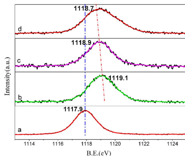
Fig. 6 Ga 2p 3/2 XPS spectra of different samples. (a) Ga 2 O 3 ; (b) Ga/calced; (c) Ga/SNSA; (d) H-Ga/SNSA.
