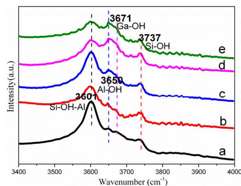
Fig. 2 DRIFT spectra in the OH stretching region of as-prepared ZSM-5 zeolites. (a) HZSM-5; (b) H-HZ/SNSA (c) Ga/calced; (d) Ga/SNSA; (e) H-Ga/SNSA.
