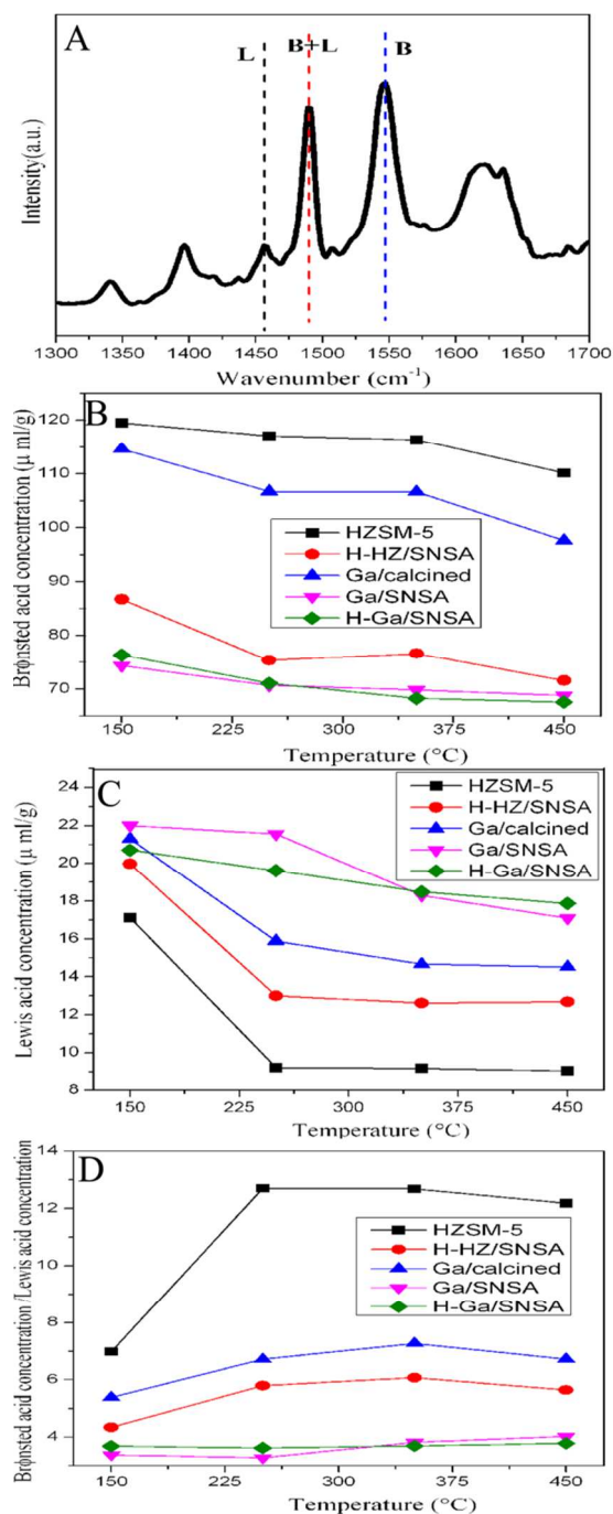
Fig. 3 The FTIR spectra of the pyridine adsorption on the catalysts and the quantified results of different acid sites. (A) Spectrum of HZSM-5 after evacuation at 450 °C; (B) Brønsted acid site concentration of samples at different temperatures; (C) Lewis acid site concentration of samples at different temperatures; (D) Brønsted acid site concentration/Lewis acid site concentration ratios of samples at different temperatures.
