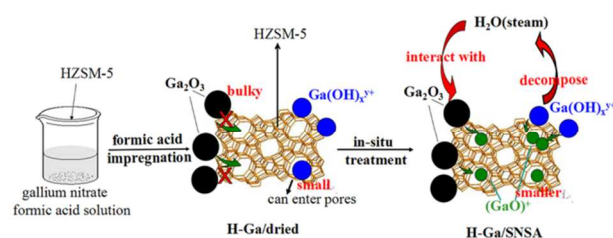
Scheme 1 Probable mechanistic route of H-Ga/SNSA
