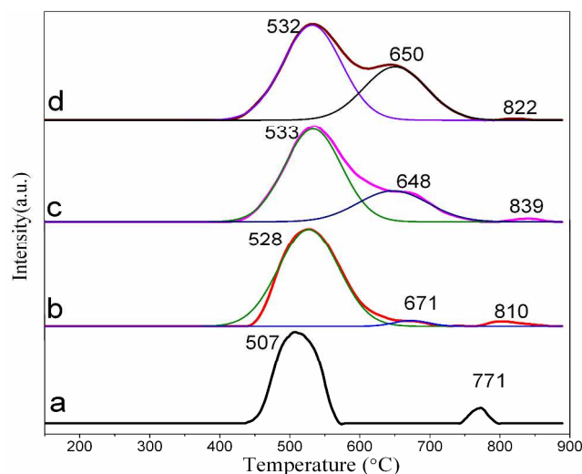
Fig. 5 H 2 -TPR profiles of different samples. (a) Ga 2 O 3 ; (b) Ga/calced; (c) Ga/SNSA; (d) H-Ga/SNSA
