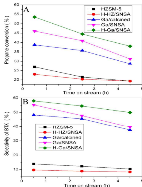
Fig. 1 Propane conversion (A) and selectivity of BTX (B) as a function of time on stream for as-prepared catalysts. Reaction conditions: P = 100 kPa, T = 540 °C, WHSV = 6000 ml/(g·h) and N 2 /C 3 H 8 molar ratio = 2.
