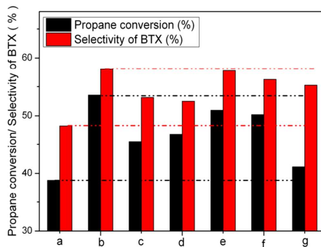
Fig. 7 Propane conversion and selectivity of BTX on as-prepared ZSM-5 zeolites. Reaction conditions: P = 100 kPa, T = 540 °C, WHSV = 6000 ml/(g·h), \text{N}_2/\text{C}_3\text{H}_8 molar ratio = 2, time on stream is 0.5h. (a) Ga/calced; (b) H-Ga/SNSA; (c) H(half)-Ga/SNSA; (d) H(double)-a/SNSA; (e) H(acetic)-Ga/SNSA; (f) H(nitric)-Ga/SNSA; (g) H(citric)-Ga/SNSA.
