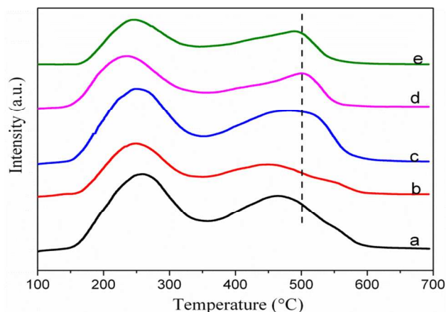
Fig.4 NH 3 -TPD profiles of different as-prepared ZSM-5 zeolites. (a) HZSM-5; (b) H-HZ/SNSA (c) Ga/calced; (d) Ga/SNSA; (e) H-Ga/SNSA.
