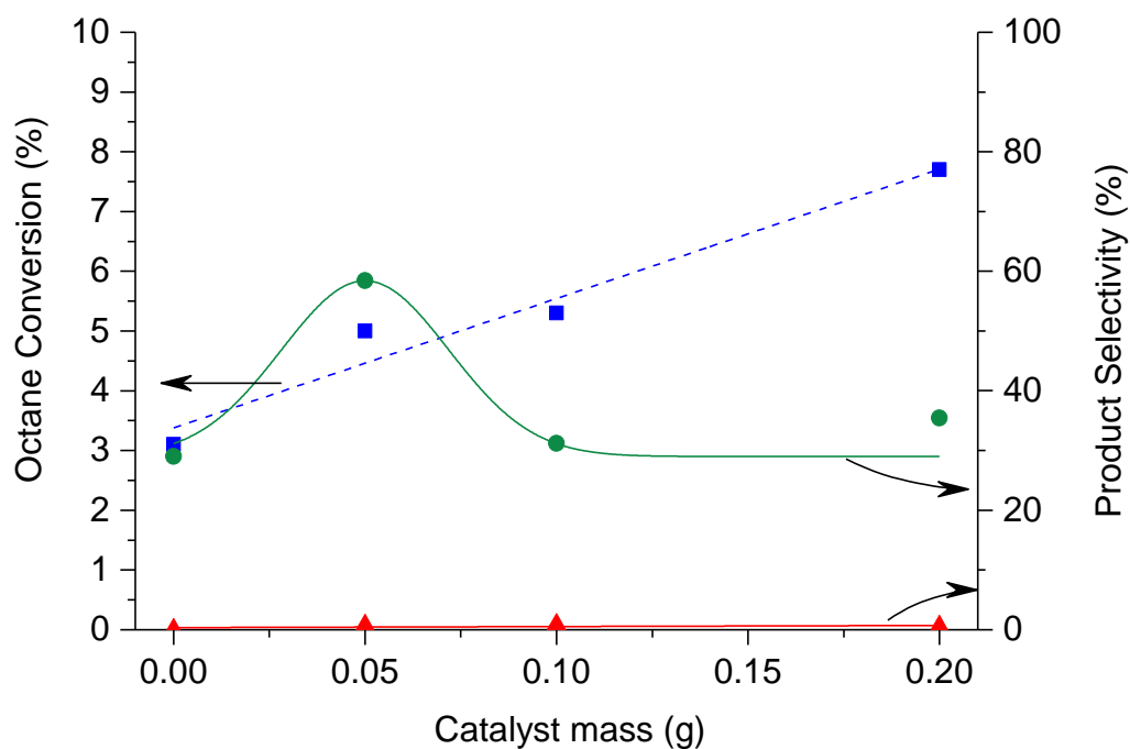
Figure 4 – Effect of 1 % AuPd/ C mass for octane oxidation. Conversion of octane (■) and product selectivity. Octanone/octanol (●) and octylbenzoate (▲). Reaction conditions: Octane (60 mmol), oxygen, ratio octane (mol) / benzaldehyde (mol) = 9:1, 20 h, 80 °C, 1500 rpm.
