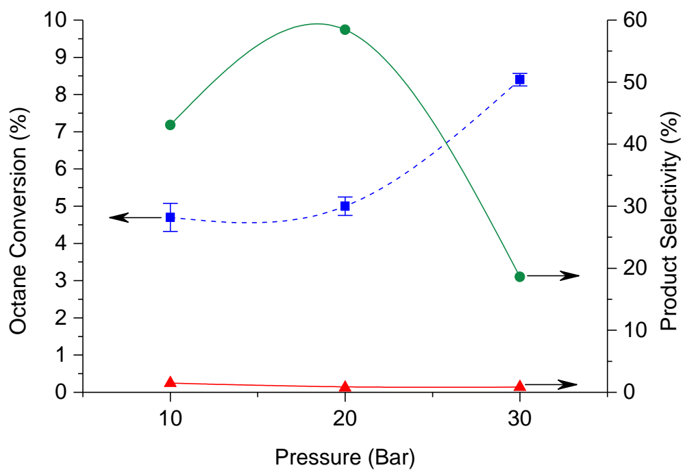
Figure 3 – Effect of pressure for octane oxidation. Conversion of octane (■) and product selectivity. Octanone/octanol (●) and octylbenzoate (▲). Reaction conditions: Octane (60 mmol), oxygen (10 to 30 bar), ratio octane (mol) / benzaldehyde (mol) = 9:1, 1 % AuPd/ C (50 mg), 20 h, 80 °C, 1500 rpm.
