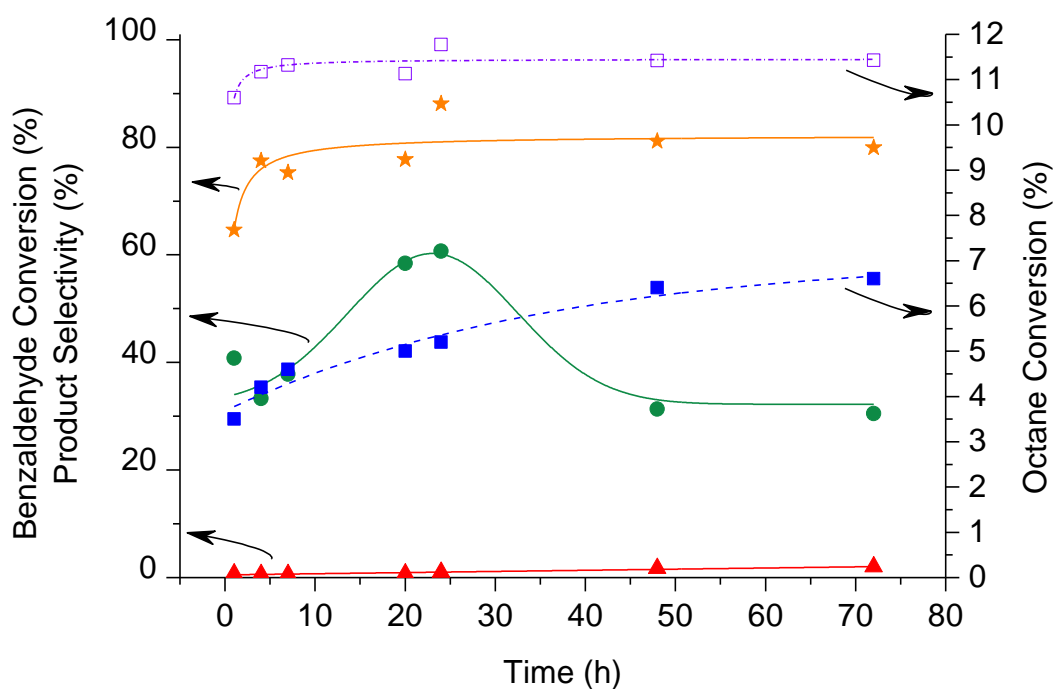
Figure 5 – Effect of reaction time for benzaldehyde conversion. Conversion of octane (■), octanone/octanol selectivity (●), octylbenzoate (▲). Conversion of benzaldehyde (□) and benzoic acid selectivity (★). Reaction conditions: Octane (60 mmol), oxygen, ratio octane (mol) / benzaldehyde (mol) = 9:1, 1 % AuPd/ C (50 mg), 80 °C, 1500 rpm.
