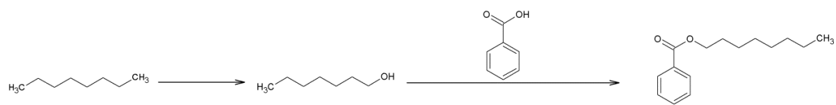
Scheme 1 – Proposed scheme for the coupling of octane with benzaldehyde
