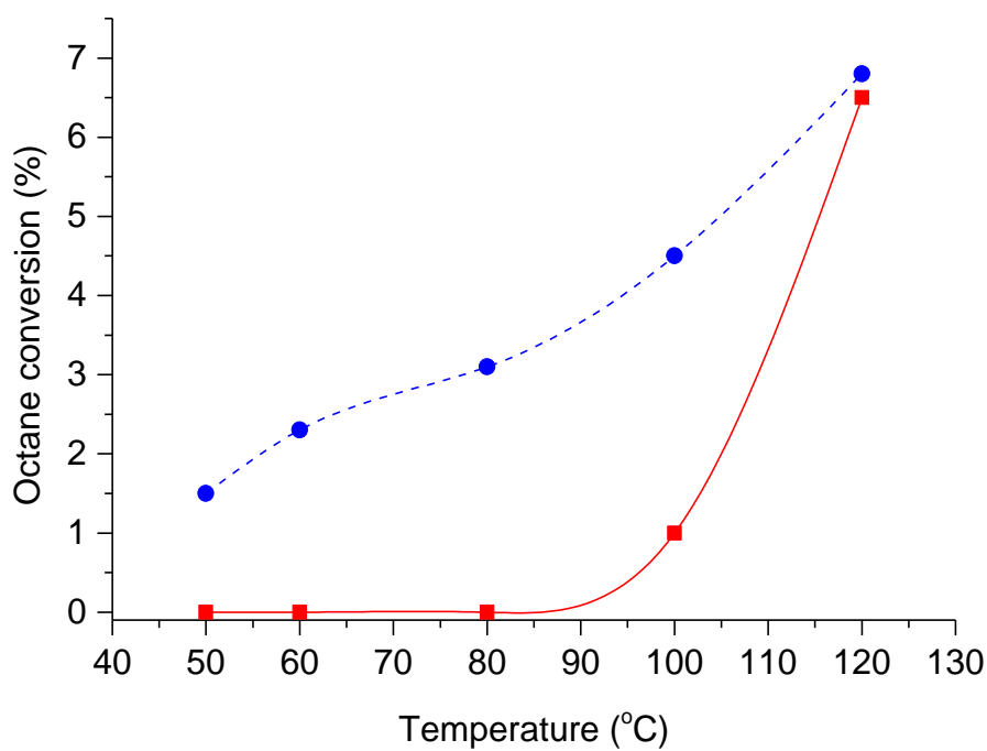
Figure 1 – Effect of reaction temperature on octane conversion with (●) and without (■) benzaldehyde in the absence of catalyst. Reaction conditions: Octane (60 mmol), oxygen, ratio octane (mol) / benzaldehyde (mol) = 9:1, no catalyst, 20 h, 1500 rpm.
