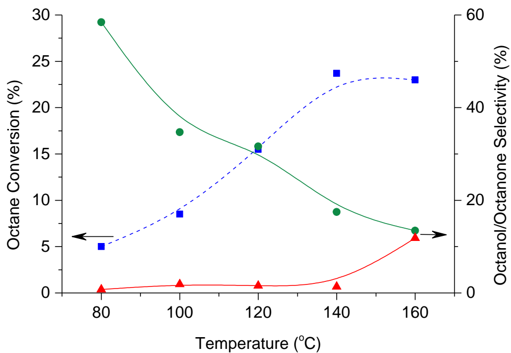
Figure 6 – Effect of temperature on octane oxidation. Conversion of octane (■) and products selectivity. Octanone/octanol (●) and octylbenzoate (▲). Reaction conditions: Octane (60 mmol), oxygen, ratio octane (mol) / benzaldehyde (mol) = 9:1, 1 % AuPd/ C (50 mg), 20 h, 1500 rpm.
