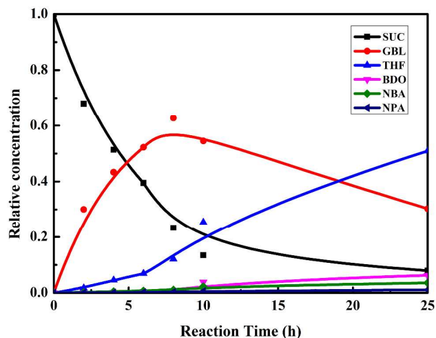
Fig. 5 Time course of succinic acid hydrogenolysis over Re/C-5 catalyst. (Reaction conditions: 20 g solution (concentration=10 wt.%), 0.2 g catalyst, 240 °C, 8.0 MPa, 800 rpm)
