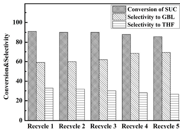
Fig. 6 Aqueous hydrogenation of succinic acid over Re/C-5 catalyst with respect to recycle run.
