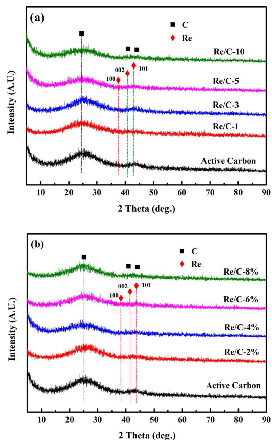
Fig. 2 XRD patterns of supported Re catalysts with different irradiation time and different Re loading.
