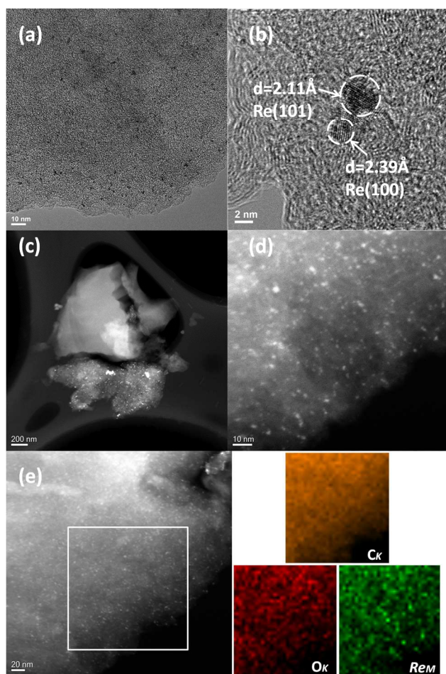
Fig. 3 TEM images (a), HRTEM images (b), HAADF-STEM (c), (d) and elemental mapping (e) of Re/C-5 catalyst which is pre-reduced by H 2 .
