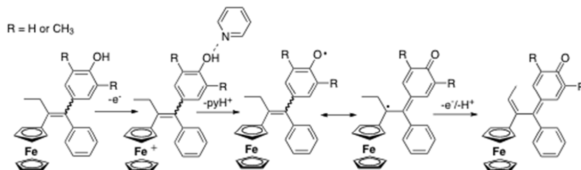
Scheme 4 : Mechanism for the formation of quinone methides 68,72
