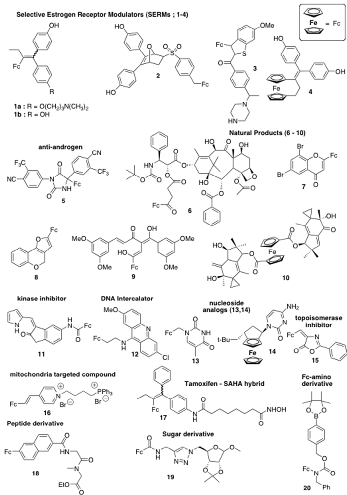
Chart 3 : Selected bioferrocene compounds
