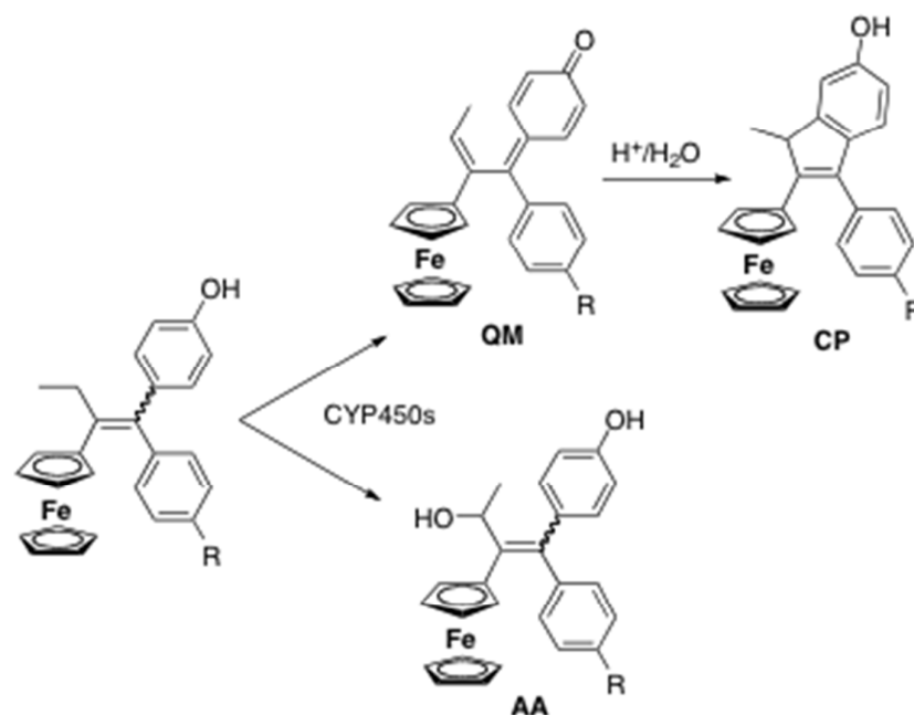
Scheme 5 : Main metabolites formed upon oxidation of ferrocifens by rat microsomes (CYP 450). R = \text{H, OH, O}(\text{CH}_2)_3\text{N}(\text{CH}_3)_2 . 74
