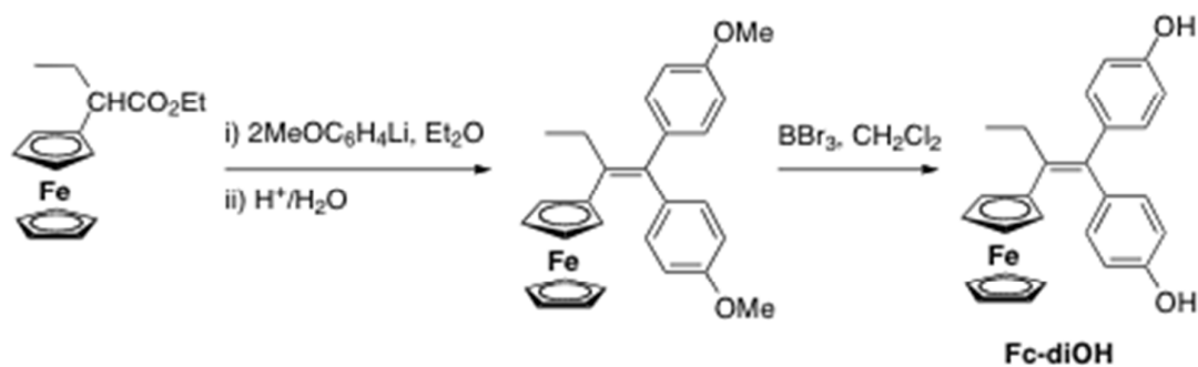
Scheme 1 : First pathway of synthesis of Fc-diOH
