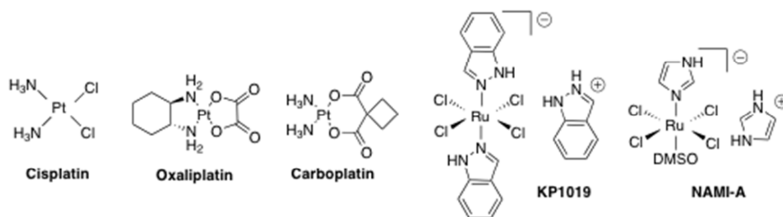
Chart 1 : Selected examples of inorganic anticancer drugs
