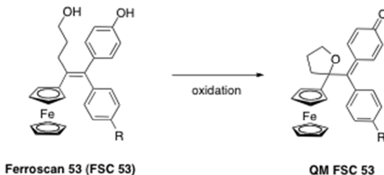
Scheme 8 : Ferrocifens with modified alkyl chain
