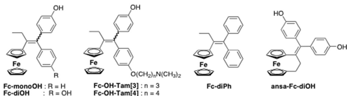
Chart 5 : Selection of ferrocifens of interest
