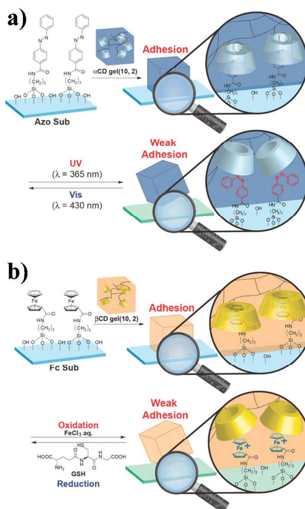
Figure 11. a) Reversible adhesion of an \alpha CD-hydrogel onto an azobenzene-functionalized surface via UV-promoted azobenzene isomerization. b) Redox-responsive reversible adhesion of a \beta CD-hydrogel onto a ferrocene-functionalized surface. Reprinted from ref. 65 with permission from John Wiley & Sons.
