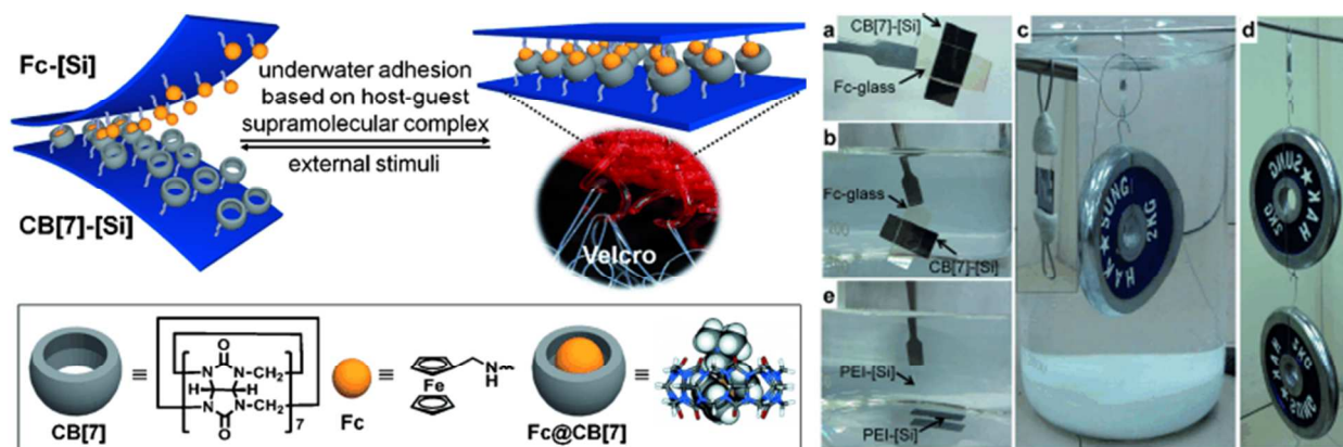
Figure 9. Redox-active adhesive based on CB[7]-Fc host-guest interactions and demonstration of underwater adhesion. Reprinted from ref. 61 with permission from John Wiley & Sons.
