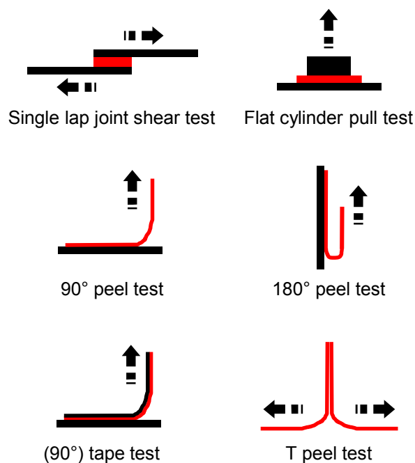
Figure 2. Overview of common test layouts to quantify the adhesive strength of an adhesive (red) to a substrate (black) or to itself.
