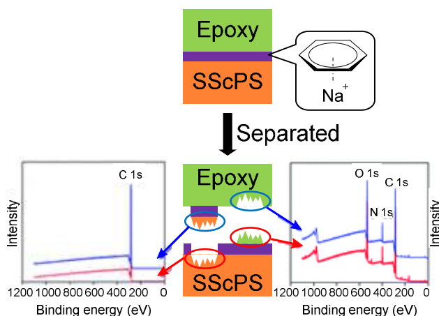
Figure 13. Approach to achieve adhesion between rigid surfaces with the use of metal cation- \pi interactions between epoxy resin and sulfonated polystyrene surfaces and determination of cohesive failure mechanism via XPS. Adapted from ref. 72 with permission from the Royal Society of Chemistry.
