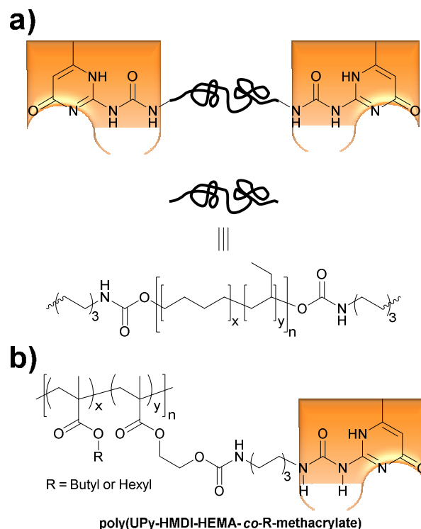
Figure 5. Chemical structures of the supramolecular polymers used by Weder and coworkers to achieve UV-light triggered debonding adhesives a) A telechelic poly(ethylene- co -butylene) (PEB) was functionalized with hydrogen bonding units (2-ureidopyrimidinone; UPy), capable of intermolecular chain-extension via UPy-UPy-dimerization. 51 b) A side-chain functionalized methacrylate copolymer with UPy as the supramolecular cross-linking unit. 52
