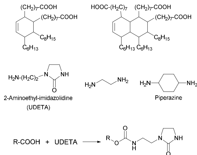
Figure 6. Chemical structures of fatty acid dimers and trimers and difunctional amines (top) that form the basis of the polyamides used by Leibler and coworkers in blends with supramolecular polymers formed by the reaction of fatty acids (and derivatives) with UDETA (bottom). 54
