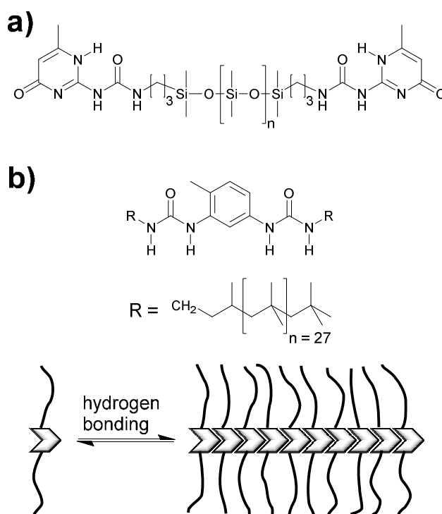
Figure 4. a) Chemical structure of UPy-functionalized telechelic PDMS, which forms a supramolecular adhesive upon linear chain extension via hydrogen bonding. 48 b) Schematic representation of the self-assembly of low-molecular weight PIB containing urea groups in the center of the chain molecules. 49
