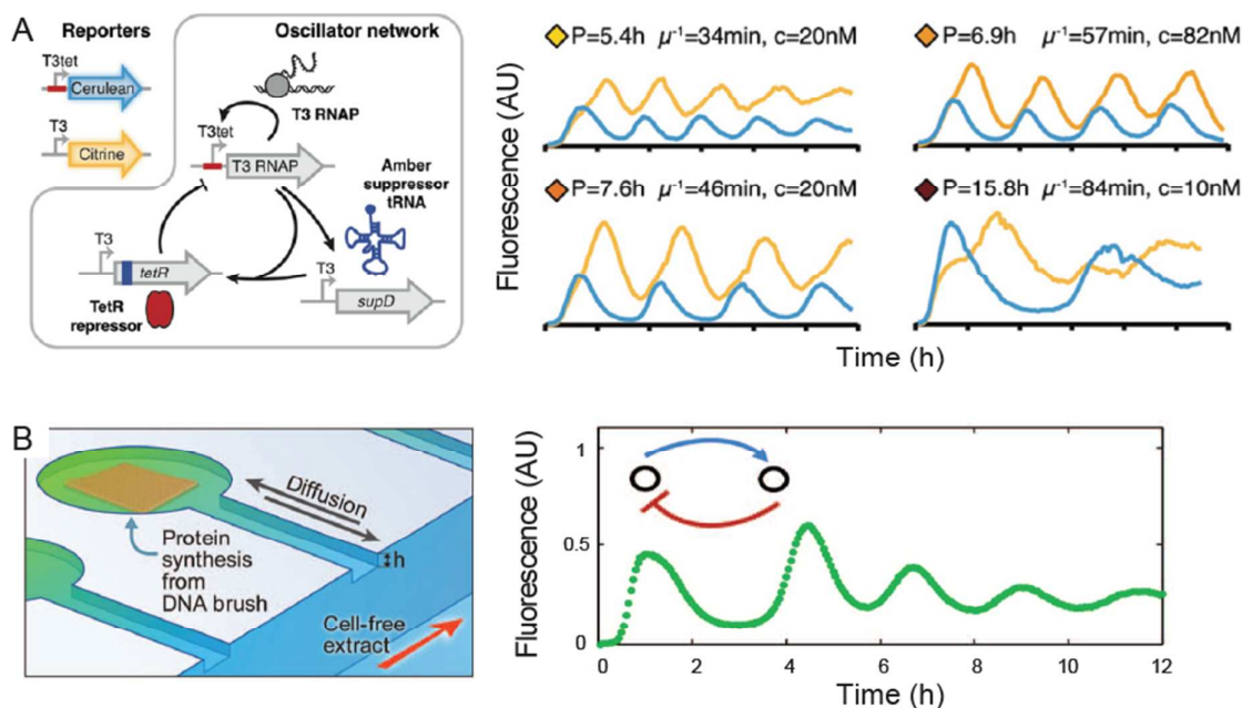
Fig. 8 In vitro oscillators based on transcription and translation chemistry and adaptation in the genelet-toolbox. (A) Operation scheme of the genetic oscillator consisting of an autocatalytic loop and delayed inhibition (left). The dynamic state of the system is measured using Cerulean and Citrine which are produced in parallel to T3RNAP and TetR repressor respectively. Oscillatory traces of Cerulean and Citrine show varying profiles and periods ( P ) at different supD gene concentrations ( c ) and different residence times ( \mu^{-1} ) (right). Reprinted with permission from ref. 33. (B) Left: Design of the microfluidic chip in which DNA brushes are assembled in circular compartments and are connected through a capillary to a feed channel. Activator-repressor genetic networks are assembled with sigma factor for activation and the lambda phage cI for repression. Right: GFP profile of oscillatory gene dynamics in an activator-repressor network measured in the compartment. Reprinted with permission from ref. 34 Copyright 2014 © American Association for the Advancement of Science.
