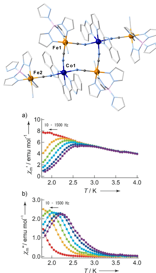
Fig. 10 (Top) Representation of the molecular structure of [\text{Co}_2\text{Fe}_4(\text{bimp})_2(\text{CN})_6(\mu\text{-CN})_6(\text{pzTp})_4] \cdot 2(1\text{-PrOH}) \cdot 4\text{H}_2\text{O} ( 30 ) at T = 100 \text{ K} . Hydrogen atoms and lattice-solvent molecules are omitted for clarity. Fe, Co, N, C, and B atoms are indicated in orange, dark blue, light blue, light grey, and pink, respectively. (Bottom) \chi' versus T (a) and \chi'' versus T (b) data for compound 30 after light irradiation ( H_{\text{ac}} = 3 \text{ Oe} oscillating at 10–1500 Hz and H_{\text{ext}} = 500 \text{ Oe} ) demonstrating the slow relaxation of the magnetization in the light-induced paramagnetic phase. Reprinted with permission from ref. 81 . Copyright 2012 Wiley-VCH.
