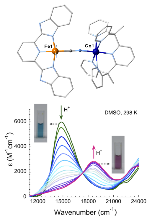
Fig. 7 (Top) Representation of the molecular structure of [(\text{bbp})\text{Fe}(\text{CN})_3\text{Co}(\text{PY5Me}_2)] \cdot 2.5\text{MeOH} ( 26 ) at T = 370 K. Hydrogen atoms, triflate and lattice-solvent molecules are omitted for clarity. Fe, Co, N and C atoms are indicated in orange, dark blue, light blue and light grey, respectively. (Bottom) Evolution of the UV-Vis spectra upon TFA (TFA: trifluoroacetic acid) addition to a solution of 26 in DMSO, showing the colour change from dark green (paramagnetic, [\text{Fe}^{\text{III}}\text{Co}^{\text{II}}]_{\text{HS}} ) to purple (diamagnetic, [\text{Fe}^{\text{II}}\text{Co}^{\text{III}}]_{\text{LS}} ). Reproduced from ref. 76 with permission from The Royal Society of Chemistry.
