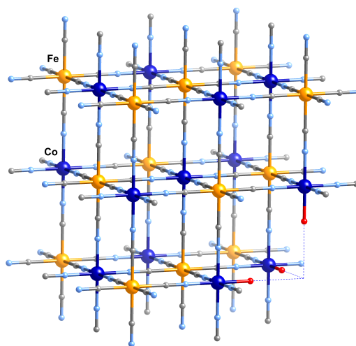
Fig. 1 Schematic representation of a Fe/Co Prussian blue network with formula A x Co y [Fe(CN) 6 ] n •nH 2 O (A: alkaline ion; C: grey; N: light blue; Co: blue; Fe: yellow; O: red).
