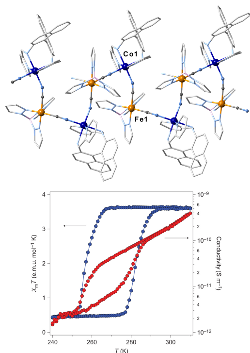
Fig. 12 (Top) Representation of the one-dimensional structure of [\text{Co}^{\text{II}}((R)\text{-pabn})][(\text{Tp})\text{Fe}^{\text{III}}(\text{CN})_3](\text{BF}_4)\cdot\text{MeOH}\cdot 2\text{H}_2\text{O} ( 35\text{R}\cdot\text{MeOH}\cdot 2\text{H}_2\text{O} ) shown at 360 K. Hydrogen atoms, tetrafluoroborate and lattice-solvent molecules are omitted for clarity. Fe, Co, N, C, and B atoms are indicated in orange, dark blue, light blue, light grey, and pink, respectively. (Bottom) Temperature dependence of the \chi T product (blue dots) and the dc conductivity (red dots) of 35\text{R}\cdot\text{H}_2\text{O} . Reprinted with permission from ref. 87. Copyright (2012) Nature Chemistry, McMillan Publishers Ltd.
