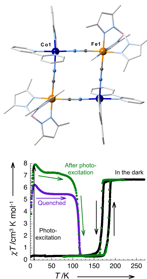
Fig. 6 (Top) Representation of the molecular structure of \{[(\text{Tp}^*)\text{Fe}^{\text{III}}(\text{CN})_3]_2[\text{Co}^{\text{II}}(\text{bpy})_2]_2\} \cdot [\text{OTf}]_2 \cdot 4\text{DMF} \cdot 2\text{H}_2\text{O} ( 14 ) at T = 230 K. Hydrogen atoms, triflate and lattice-solvent molecules are omitted for clarity. Fe, Co, N, C, and B atoms are indicated in orange, dark blue, light blue, light grey, and pink, respectively. (Bottom) \chi T versus T data of 14 at 0.4 \text{ K min}^{-1} before (black dots, 0.1 T) and after (green dots, 1 T) white light irradiation, and after thermal quenching (purple dots, 0.1 T). Reprinted with permission from ref. 61. Copyright 2010 Wiley-VCH.
