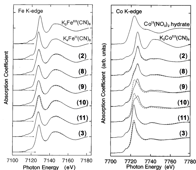
Fig. 3 Fe K -edge (left) and Co K -edge (right) XANES spectra for compounds 2 , 8 , 9 , 10 , 11 and 3 at 30 K (solid lines) and 296 K (dashed lines). Spectra for \text{K}_3\text{Fe}^{\text{III}}(\text{CN})_6 and \text{K}_4\text{Fe}^{\text{II}}(\text{CN})_6 (Fe K -edge) and for \text{K}_3\text{Co}^{\text{III}}(\text{CN})_6 and \text{Co}(\text{NO}_3)_2 hydrate (Co K -edge) were added for comparison. Adapted with permission from Ref. 43. Copyrighted by the American Physical Society.
