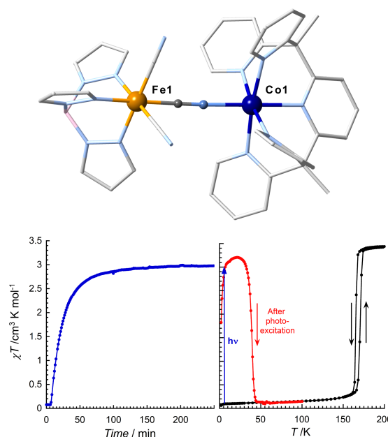
Fig. 8 (Top) Representation of the molecular structure of [(Tp)Fe(CN) 3 Co(PY5Me 2 )](OTf)•2DMF ( 27 •2DMF) at T = 180 K. Hydrogen atoms, triflate and lattice-solvent molecules are omitted for clarity. Fe, Co, N and C atoms are indicated in orange, dark blue, light blue and light grey, respectively. (Bottom) \chi T versus time (blue circles) of the desolvated compound, 26 , at 1 T and 10 K under white light irradiation (3 mW/cm 2 ), and \chi T versus temperature before (black dots) and after (red dots) white light irradiation with a sweep rate of 0.4 K min -1 . Reprinted with permission from ref. 77. Copyright 2014 American Chemical Society.
