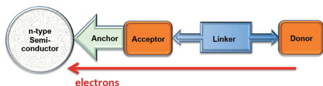
Fig. 5. Schematic representation of a 'push-pull' dye to direct electron transfer from the periphery of the dye to the n-type semiconductor. In a copper(I) complex, the 'linker' is the copper(I) centre, the 'donor' is the ancillary ligand, and the 'acceptor and anchor' are combined in the anchoring ligand.
