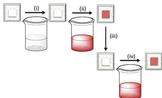
Fig. 14. Stepwise, on-surface assembly of [\text{Cu}(\text{L}_{\text{anchor}})(\text{L}_{\text{ancillary}})]^+ dyes (steps (i) and (ii), see Fig. 6) followed by (iii) exposure to iodide ion which bleaches the electrode, and regeneration of the dye by (iv) soaking in a solution of [\text{Cu}(\text{L}_{\text{ancillary}})_2]^+ (a repeat of step (ii)).
