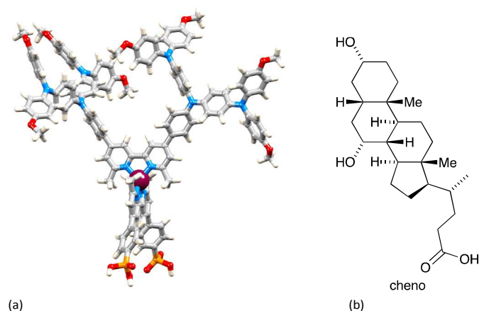
Fig. 11. (a) Modelled structure of [\text{Cu}(\mathbf{3})(\mathbf{8}_{\text{methyl}})]^+ (molecular mechanics level, Spartan 14 v. 1.1.8, Wavefunction, Inc.). (b) Structure of co-adsorbant chenodeoxycholic acid (cheno).
