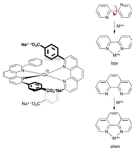
Scheme 1. The first bis(diimine) copper(I) dye used in DSCs by Sauvage and coworkers, and chelate formation by bpy and phen emphasizing the conformational change required by bpy contrasting with the preorganized metal-binding domain offered by phen.
