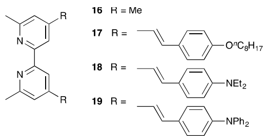
Scheme 9. Structures of ancillary ligands 16–19 .
