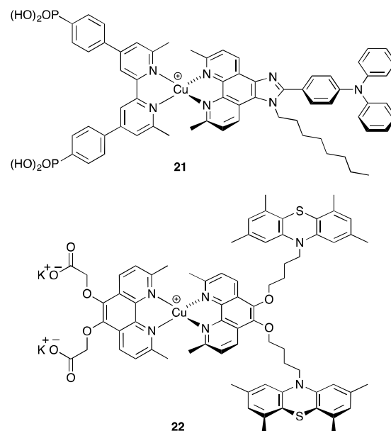
Scheme 11. Structures of copper(I) sensitizers used in DSCs with Co^{2+}/Co^{3+} electrolytes.
