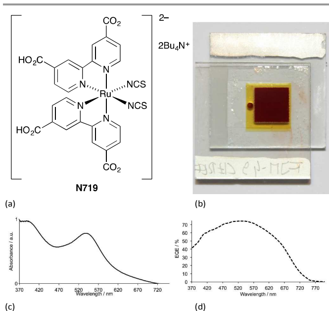
Fig. 4. (a) The structure of ruthenium dye N719. (b) A sealed DSC containing N719 sensitizer adsorbed on TiO 2 ; the device also contains [I - /I 3 - ] electrolyte. (c) The solid-state absorption spectrum of a TiO 2 electrode with adsorbed N719, and (d) the EQE spectrum of a DSC containing N719 showing the wide wavelength range over which photons are absorbed and converted into electrical current.
