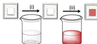
Fig. 6. Stepwise, on-surface assembly of [\text{Cu}(\text{L}_{\text{anchor}})(\text{L}_{\text{ancillary}})]^+ dyes involves soaking an FTO/ \text{TiO}_2 electrode (i) in a colourless solution of \text{L}_{\text{anchor}} , and then (ii) in a coloured solution containing [\text{Cu}(\text{L}_{\text{ancillary}})_2]^+ or a mixture of [\text{Cu}(\text{NCMe})_4]^+ and \text{L}_{\text{ancillary}} , followed by drying of the electrode.
