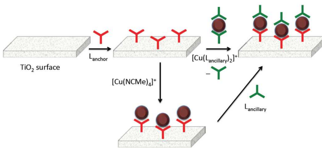
Fig. 7. 'Surfaces-as-ligands, surfaces-as-complexes' approach to heteroleptic copper(I) dyes. In the route shown at the top of the figure, ligand exchange involves a homoleptic complex and there is wastage of one equivalent of \text{L}_{\text{ancillary}} (shown in green). In the second route, a 1 : 1 ratio of [\text{Cu}(\text{NCMe})_4]^+ and \text{L}_{\text{ancillary}} is used either in one dye-bath or sequential dye baths.
