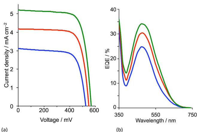
Fig. 10. (a) J-V curves and (b) EQE spectra of DSCs containing [\text{Cu}(\mathbf{3})(\mathbf{4})]^+ (blue), [\text{Cu}(\mathbf{3})(\mathbf{5})]^+ (red) and [\text{Cu}(\mathbf{3})(\mathbf{6})]^+ (green). 38
