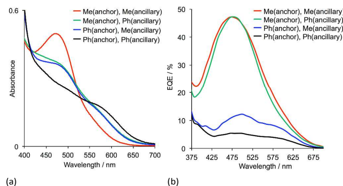
Fig. 9. (a) Solid-state absorption spectra and (b) EQE spectra of \text{TiO}_2 electrodes with adsorbed dyes containing 6,6'-Me 2 bpy or 6,6'-Ph 2 bpy copper-binding domains. 30 The ligands are shown in Fig. 8b.
