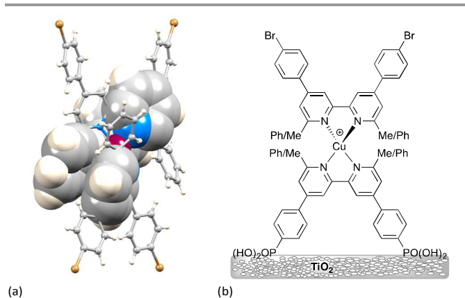
Fig. 8. (a) Flattening of the tetrahedral geometry around the Cu atom caused by \pi -stacking of two pairs of phenyl-pyridine rings; the structure shown was crystallographically determined for a homoleptic complex containing two 4,4'-bis(4-bromophenyl)-6,6'-diphenyl-2,2'-bipyridine ligands. 36 The rings involved in \pi - \pi interactions are shown in space-filling representations. (b) Structures of the dyes used to demonstrate the effects of having 6,6'-Me 2 bpy or 6,6'-Ph 2 bpy copper-binding domains in anchoring versus ancillary ligands.
