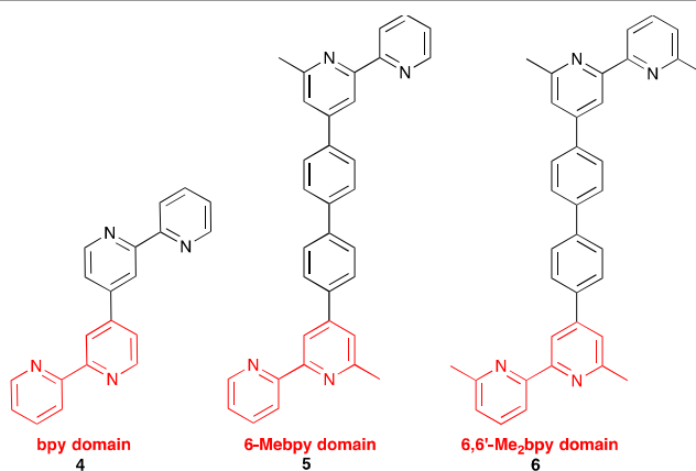
Scheme 5. Ancillary ligands used to combine with anchor 3 (Scheme 5) in the dyes [\text{Cu}(\mathbf{3})(\mathbf{4})]^+ , [\text{Cu}(\mathbf{3})(\mathbf{5})]^+ and [\text{Cu}(\mathbf{3})(\mathbf{6})]^+ . The copper-binding domain is shown in red.
