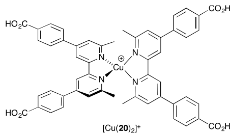
Scheme 10. Structure of the dye [Cu(20)_2]^+ used by Biagini and coworkers to demonstrate the effects of \Gamma/I_3^- electrolyte composition on DSC performance.
