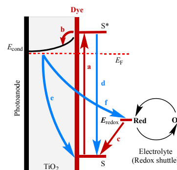
Fig. 3. Summary of electron transfer processes at the photoanode in an n-type DSC: desired transfers are shown in red, and back reactions in blue. (a) Photoexcitation of the dye; (b) electron injection; (c) electron transfer from reduced form of the electrolyte to oxidized form of the dye; (d) decay of the excited state dye back to the ground state; (e) recombination of the injected electron with the oxidized dye; (f) recombination of the injected electron with the oxidized electrolyte.
