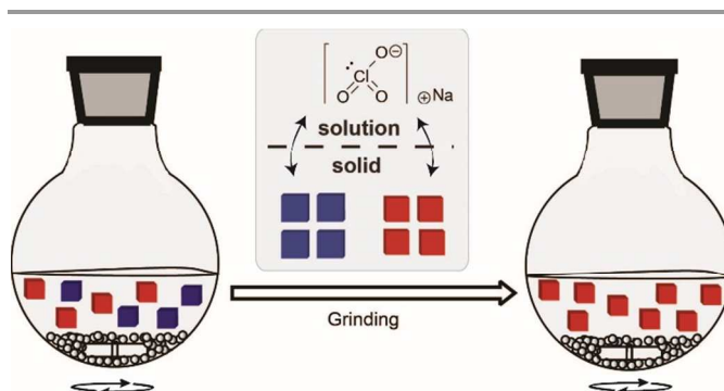
Fig. 7 Schematic representation of Viedma’s experiment.
