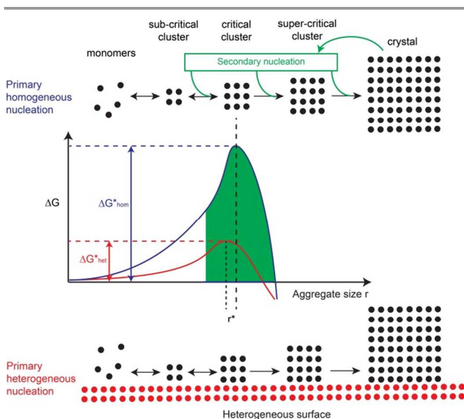
Fig. 2 The formation of crystals from solution proceeds either through primary-(homogeneous or heterogeneous) or through secondary nucleation.
