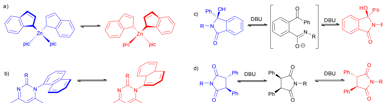
Fig. 11 Selected conglomerate-forming chiral molecules that racemise differently in solution.
