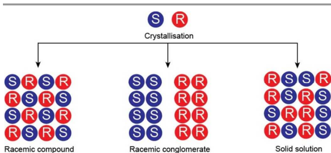
Fig. 3 Enantiomers crystallise either as a racemic compound, racemic conglomerate or a solid solution.
