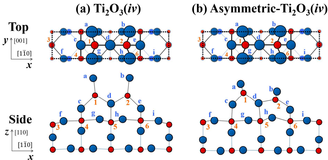
Figs. 6 Schematic top and side views of the structures for (a) the \text{Ti}_2\text{O}_3(iv) and (b) the asymmetric- \text{Ti}_2\text{O}_3(iv) models after adjustment of the atomic positions. Each dotted rectangle indicates a (1 \times 2) unit cell. The red circles labelled with numbers indicate Ti atoms and the blue circles labelled with lowercase letters indicate O atoms. Each is drawn in accordance with the x , y and z coordinates of atomic positions adjusted for the best (smallest) value of R within the model, as listed in Table 1.
