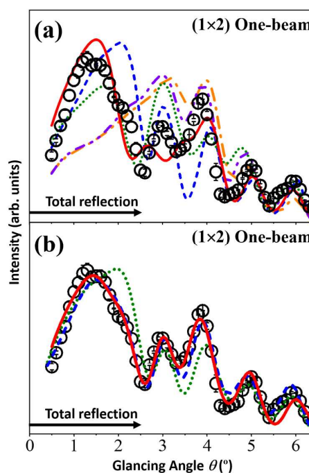
Figs. 4 The TRHEPD rocking-curves for the rutile- \text{TiO}_2 (110)- (1\times 2) surface under the one-beam condition. Open circles in (a) and (b) are the same experimental data. Uncertainties estimated as for the data in Figure 3 are also shown. The single-dotted-broken (orange), broken (blue), double-dotted-broken (purple), dotted (green) and solid (red) curves are calculated results from the missing-row, the \text{Ti}_2\text{O}_3 , the \text{Ti}_2\text{O} , the \text{Ti}_3\text{O}_5 and the asymmetric- \text{Ti}_2\text{O}_3 models, respectively, using the z coordinates (a) proposed in the original studies and (b) adjusted to give better R values.
