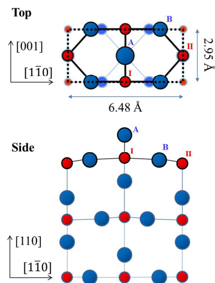
Fig. 1 Schematic top and side views of the established rutile-TiO 2 (110)-(1×1) surface. The dotted rectangle indicates a (1×1) unit cell. Red and blue circles, labelled with Roman numerals and uppercase letters, represent Ti and O atoms, respectively. In the top view, Ti and O atoms at higher positions are depicted by circles with larger diameters.
