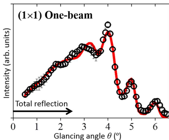
Fig. 3 The TRHEPD rocking-curve for the rutile- \text{TiO}_2 (110)- (1\times 1) surface under the one-beam condition. The open circles denote experimental data. The uncertainty is shown by a bar on each circle. The red solid curve shows the calculated result.
