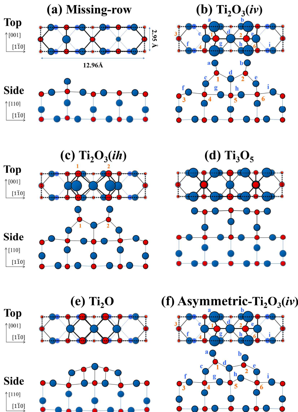
Figs. 2 Schematic top and side views of structural models of the rutile-TiO 2 (110)-(1×2) surface: (a) missing-row 29 ; (b) Ti 2 O 3 (iv) 23 ; (c) Ti 2 O 3 (ih) 24 ; (d) Ti 3 O 5 21 ; (e) Ti 2 O 27 ; and (f) asymmetric-Ti 2 O 3 (iv) 25 models. Each dotted rectangle indicates (1×2) unit cell. The red circles indicate Ti atoms, labelled with numbers in (b), (c) and (f), and the blue circles indicate O atoms, labelled with lowercase letters.
