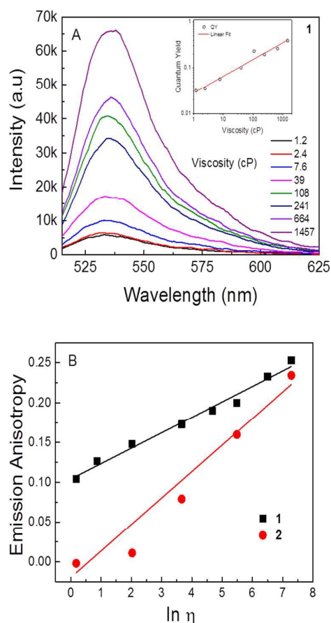
Fig 2. A: emission spectra of dye 1 in different viscosity mixtures of ethanol:glycerol; inset: quantum yield as function of viscosity. B: steady state emission anisotropy of 1 and 2 as a function of viscosity
