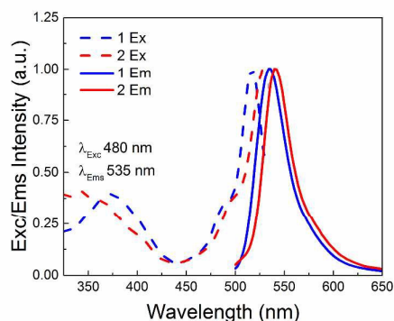
Fig 1: Excitation and emission spectra of 1 and 2
