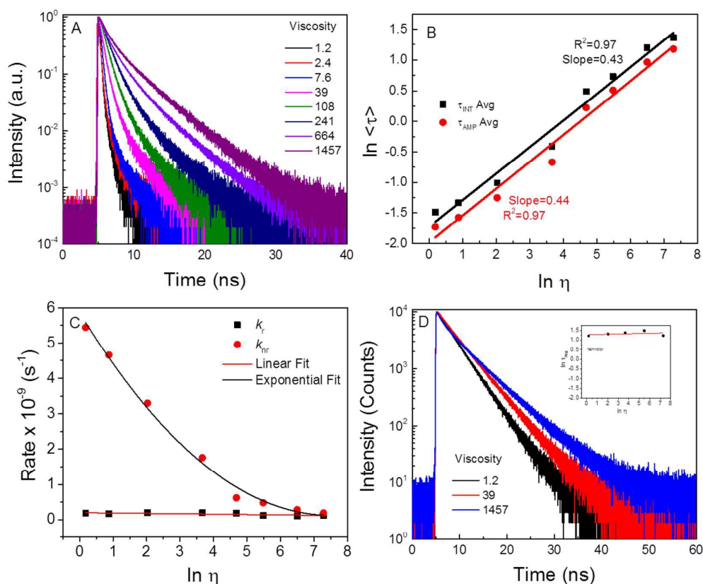
Fig 3. A: Fluorescence intensity decays of rotor 1 in media of different viscosities. B: Average fluorescence lifetimes of 1 as function of viscosity. C: Radiative ( k_r ) and non-radiative ( k_{nr} ) rates of 1 as a function of viscosity. D: Intensity decays of 2 in media of different viscosity. Inset: Lifetime as a function of viscosity.
