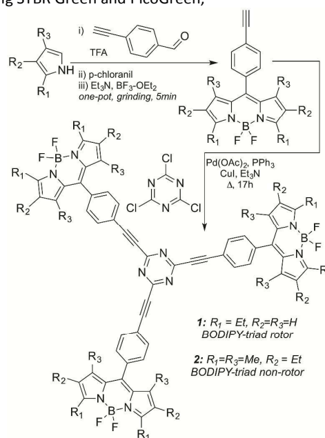
Scheme 1: Synthesis of BODIPY trimer 1 and 2
