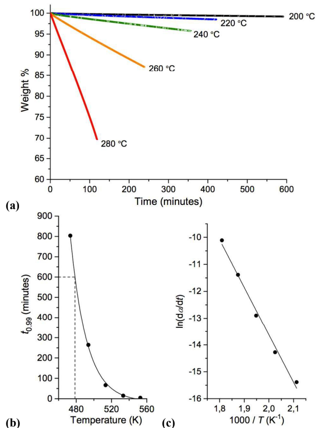
Fig. 6 Determination of the long-term thermal stability of [7+6]Cl, 8 : (a) Isothermal TGA thermographs; (b) Exponential fit of T (K) vs. t_{0.99} (mins) to determine T_{0.01/10} ; (c) Determination of E_a and A .
