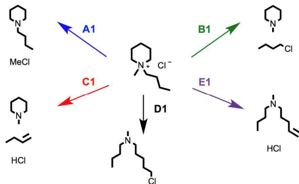
Fig. 7 Proposed S_N2 (A1, B1 and D1) and E2 Hofmann elimination (C1 and E1) thermal decomposition pathways for [C_4C_1\text{pip}]\text{Cl} 2 .
