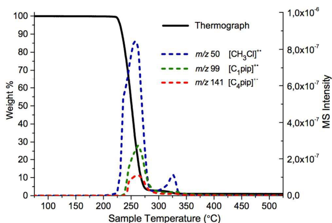
Fig. 8 TGA-MS evaluation of [C_4C_1\text{pip}]\text{Cl} 2 . The continuous line denotes the TGA thermograph, the coloured dashed lines denote MS intensities for select m/z values. The assigned products are indicated. The thermograph is shown in the range 75–525 ^\circ\text{C} , for clarity.
