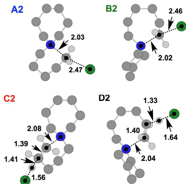
Fig. 12 TS structures for [7+6]Cl, 8 , representing S_N2 (A2, B2) and E2 (C2, D2) mechanisms relative to the lowest energy ‘ \gamma_{\text{chair1}}\delta_{\text{chair}}\alpha\alpha' ’ ion pair conformer (Fig. 4). Atom distances are in angstroms.
