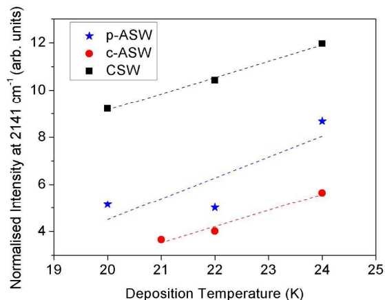
Figure 3: Intensity measured at 2141 cm -1 in the RAIR spectra normalized by the total area of the νCO band for each substrate, as a function of deposition temperature. The dotted line results from a linear fit of the data and is only presented here to guide the eye.
