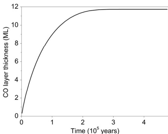
Figure 5: The accumulation of monolayers of CO as a function of time on grains of initial radius 0.1\mu\text{m} , for the physical conditions in B68 outlined in the text.
