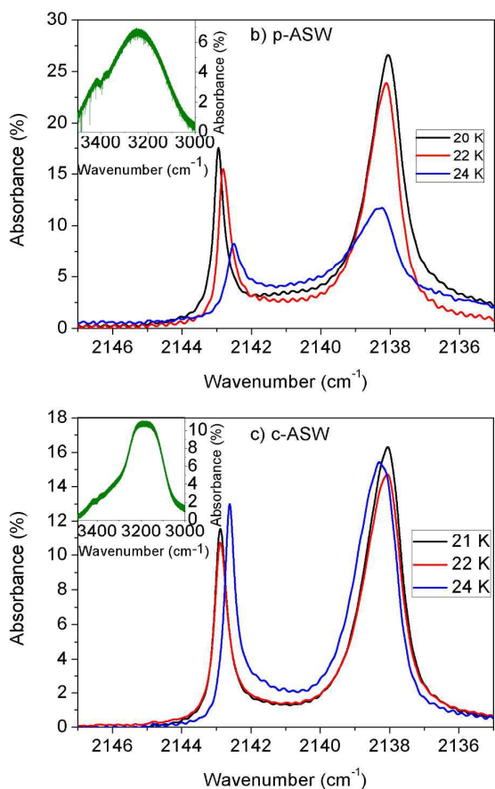
Figure 1: RAIR spectra collected after CO has been deposited at 20 or 21 (black), 22 (red) and 24 (blue) K on CSW (a), p ASW (b) and c ASW (c). The inserts in each graph show the OH stretch for the water substrate beneath the CO layer. In each case a contraction in the LO-TO splitting of the CO stretching mode is seen as the deposition temperature increases.
