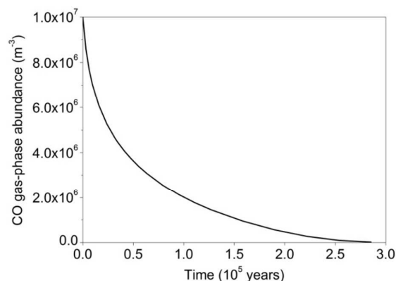
Figure 4: the removal of CO with respect to time from the gas phase, initially at 10^7 m^{-3} , through condensation onto dust grains, according to Eq.9. The physical conditions are CO/H_2 = 10^{-4} , n_{H_2} = 10^{11} m^{-3} , T = 10 K, initial grain radius at t=0 , a_b = 10^{-7} m, with other relevant parameters given in Table 6 .
