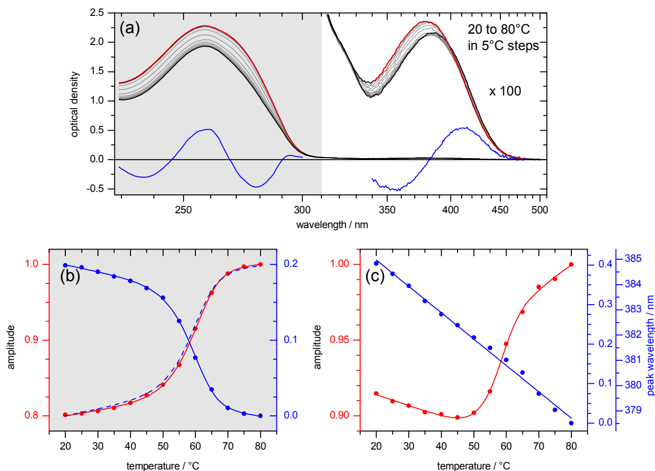
Fig. 4 (a) Absorption spectra of ds13mer4AP-DAP upon raising temperature from 20°C to 80°C ( c_T = 20.5 \mu\text{M} ). Decomposition was performed separately for the range \lambda < 310 \text{ nm} (nucleobases) and \lambda > 340 \text{ nm} (4AP). Generally the first component (red) is taken to be the 80°C spectrum, i.e. it represents the fully separated single strands. The remaining second component (blue) therefore describes the change of spectral form and position for lower temperatures.
