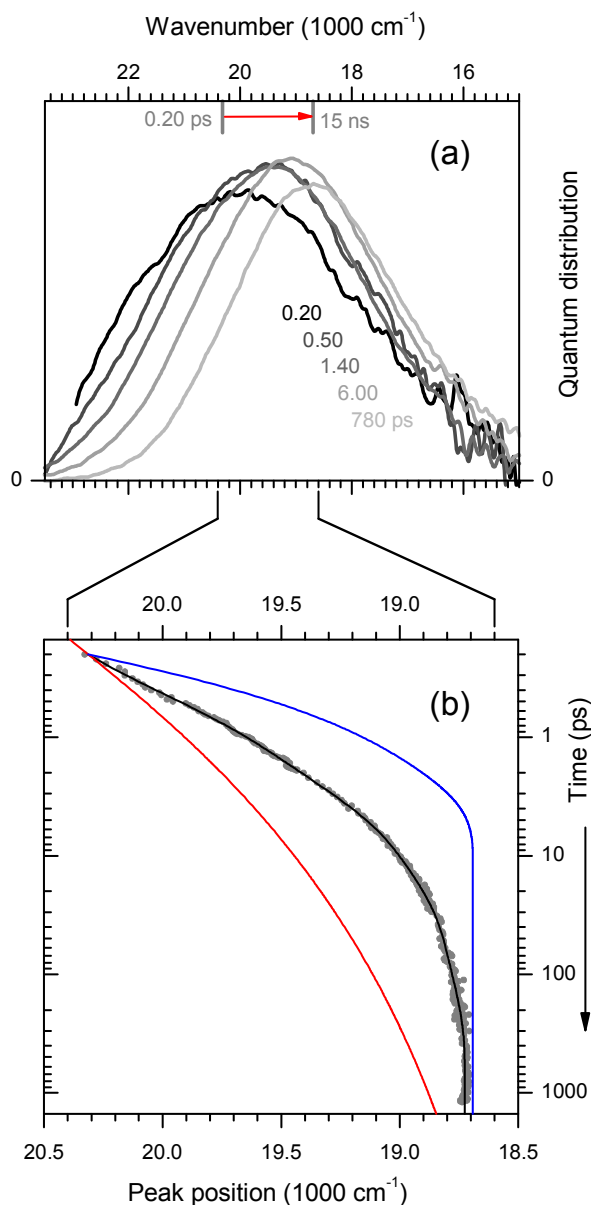
Fig. 6 (a) Transient 4AP fluorescence spectra from the duplex in \text{H}_2\text{O} buffer, measured by broadband upconversion with 100 fs time resolution.
