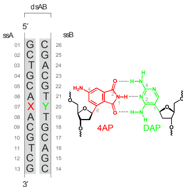
Fig. 1 Chemical structure of the base pair analogue 4AP-DAP and sequence of the double-stranded oligomer ds13mer4AP-DAP. Native DNA is marked black and modifications, including backbone, red for site X or green for site Y, respectively.
