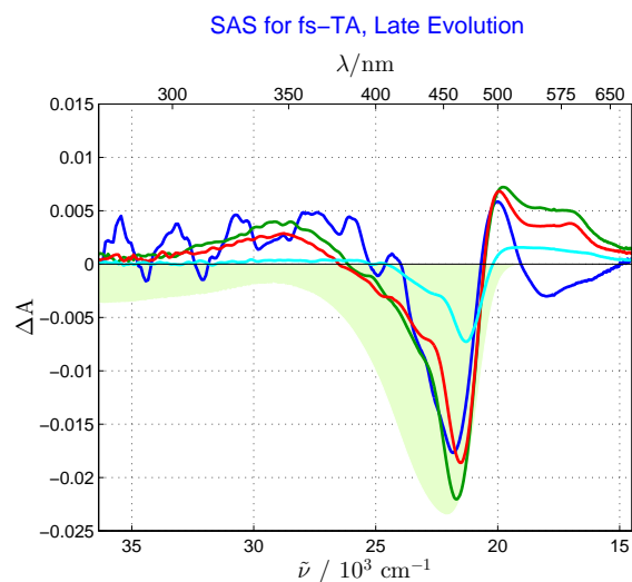
Fig. 4 SAS obtained from the kinetic analysis in the 100 ps time scale with constant steps of 200 fs. Ultrafast wavepacket spreading and IVR in state A goes unnoticed in this time scale ( A , blue). B (green) relaxes to B cold (red) mainly by vibrational cooling. C (cyan) is the long-living component that forms by 2-photon excitation in the fs experiments. The mechanism for one-photon excitation, from which the A , B and B cold -SAS derive, is shown in Scheme 2. Optimal values of the associated rate constants are collected in Table 2.
