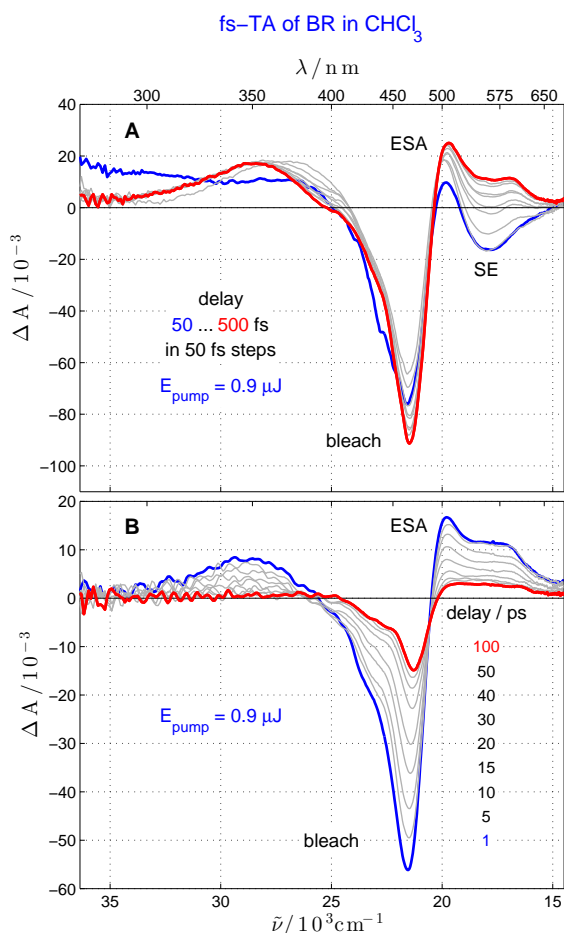
Fig. 1 Spectral evolution of BR in CHCl 3 observed during the earliest 500 fs in the UV-Vis spectral window after 400 nm excitation with parallel pump-probe polarization (panel A). Spectra measured between 50 (blue) and 500 fs (red) delays are shown in 50 fs steps. SE decays in this time scale. The spectral evolution is not obvious in the bleach and ESA regions because of the underlying coherent contribution and the signal oscillations from a vibrational wavepacket in the solvent (see Figure SI 2). Panel B shows the spectral evolution in the 100 ps time scale with the same experimental conditions. The time delays are color-coded.
