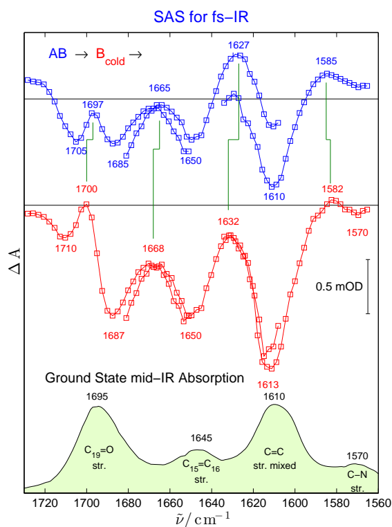
Fig. 6 SAS obtained for the Vis-pump/mid-IR probe transient absorption spectra of BR in chloroform after the mechanism in the inset of Figure 3, as seen with the time resolution of the mid-IR experiment. The C–N, C=C and C=O str regions were studied. The steady-state mid-IR absorption spectrum is shown as a light-green-filled curve. Transient spectra were measured in three independent windows (1580–1635, 1610–1680 and 1650–1730 \text{cm}^{-1} ) and fitted globally by target analysis. The green lines show the shift of the excited-state signals during the AB (blue) to B cold (red) transformation. A tentative band assignment of the steady-state mid-IR spectrum is indicated.
