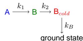
Scheme 2 Mechanism for the deactivation of BR after 1-photon excitation.
