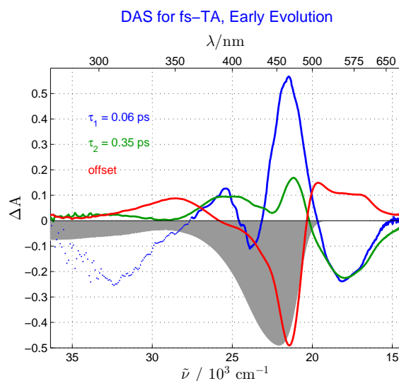
Fig. 2 Decay associated spectra (DAS) obtained from the fits in Figure SI 2. Decay times of 0.06 and 0.35 ps were deduced. The amplitude of the faster component is uncertain to the blue of 350 nm (blue dotted line) because of the longer cross-correlation in the UV. Note that the global fit procedure assumes constant cross-correlation across the spectral window. This assumption distorts spectra associated to ultrafast decay times in the UV and near-IR, where the instrumental cross-correlation is broader. Hence, the DAS of the 0.06 ps component is unreliable to the blue of 350 nm and to the red of 650 nm. The steady-state absorption spectrum of BR is shown as an inverted grey-filled curve for comparison.
