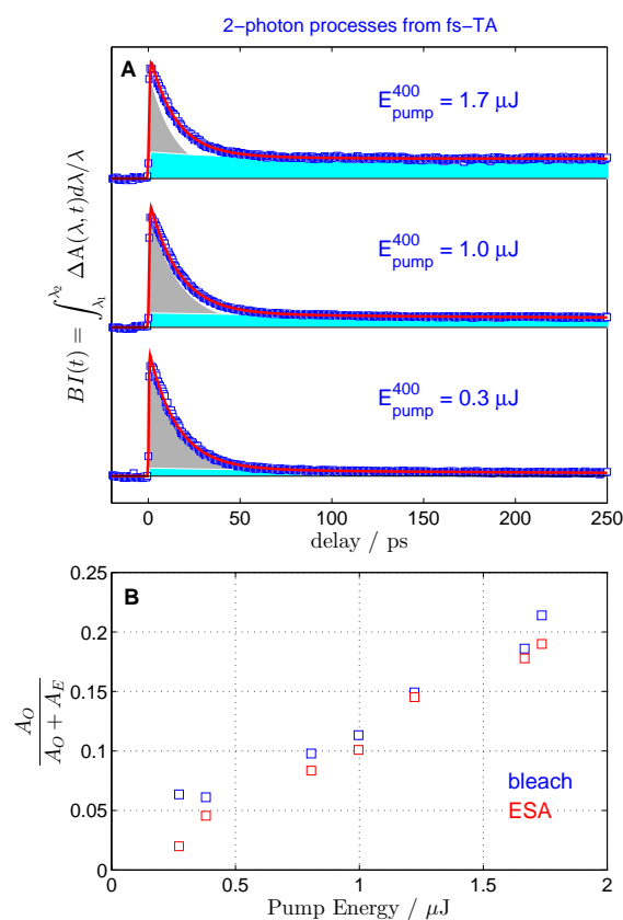
Fig. 3 The panel A shows the normalized bleach band integrals calculated between 415 and 475 nm at the indicated pump energies (blue squares). The pump-probe polarization is parallel. The fit with a biexponential function and a non-decaying component is shown in red. The fast exponential, ca. 15 ps, is shown as a gray-filled curve whereas the contributions of the long exponential ( \approx 200 ps, due to rotational diffusion) and the offset are quantified by the cyan-filled curve. Panel B shows how the relative amplitudes of the long-living components depend on pump energy. They are calculated as the ratio between the time-zero amplitudes of the long exponential (accounting for rotational diffusion) and the offset ( A_0 ) and the full amplitude A_0 + A_E , where A_E is the time-zero amplitude of the fast exponential. The blue squares show the calculations for the bleach band while the red squares refer to the ESA band at about 600 nm. The ESA band integral is calculated from 525 to 625 nm.
