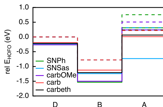
Fig. 6 Energy levels of the HOFO of the hole acceptor candidates and the HOFOs of the linearly conjugated biphenyl bridge and PMI in the DBA molecules (solid line) compared to the isolated fragments (dashed line).
