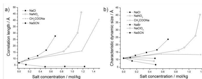
Figure 3. a) Correlation lengths \xi_x in Å obtained from SAXS; and b) characteristic dynamic size \xi_D in Å obtained from DLS plotted against the anion concentration in mol/kg.
