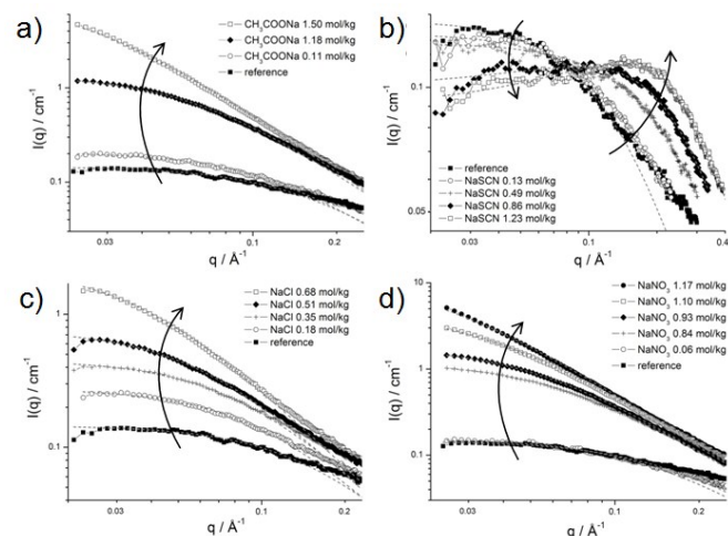
Figure 2. SAXS spectra on a log-log scale and in absolute units of the formulation water/ethanol/1-octanol in presence of a) \text{CH}_3\text{COONa} ; b) \text{NaSCN} ; c) \text{NaCl} ; and d) \text{NaNO}_3 . The dotted lines are the fits done with the Ornstein-Zernike equation or with equation (3) in the case of \text{NaSCN} .
