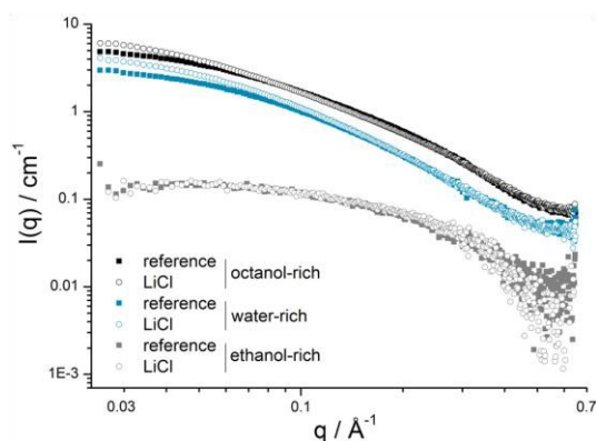
Figure 7. SANS curves on a log-log scale and in absolute units of the formulation corresponding to point \alpha with 0.5 mol/kg \text{LiCl} . The correlation length \xi_N stays almost the same for the octanol-rich contrast and is equal to 16 Å. \xi_N increases from 6.3 to 6.6 Å for the ethanol-rich contrast and from 16.0 to 19.0 Å for the water-rich contrast.
