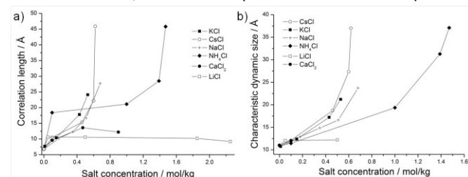
Figure 6. a) Correlation length \xi_x in Å obtained from SAXS; b) characteristic dynamic size \xi_D in Å obtained from DLS plotted against the cation concentration in mol/kg.
