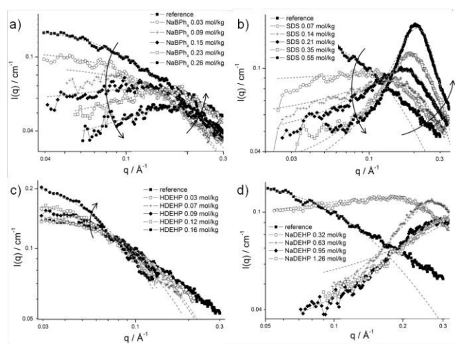
Figure 8. SAXS spectra on a log-log scale and in absolute units for the system water/ethanol/1-octanol in presence of a) NaBPh 4 ; b) SDS; c) HDEHP; and d) NaDEHP. The dotted lines are the fits corresponding to the Ornstein-Zernike equation or to equation (3).
