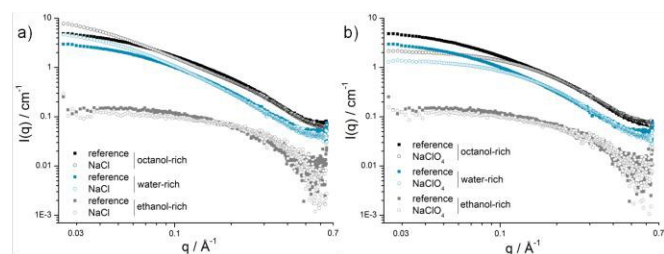
Figure 4. SANS curves on a log-log scale and in absolute units of the formulation corresponding to point \alpha with a) 0.35 mol/kg \text{NaCl} , and b) 0.46 mol/kg \text{NaClO}_4 . For \text{NaCl} , the correlation length \xi_N increases from 16.3 to 18.8 Å for the octanol-rich contrast, from 16.0 to 22.0 Å for the water-rich contrast, and decreases from 6.3 to 5.1 Å for the ethanol-rich contrast. For \text{NaClO}_4 , the correlation length \xi_N decreases from 16.3 to 8.6 Å for the octanol-rich contrast, from 16.0 to 9.4 Å for the water-rich contrast, and from 6.3 to 5.8 Å for the ethanol-rich contrast.
