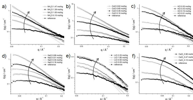
Figure 5. SAXS spectra on a log-log scale and in absolute units for the system water/ethanol/1-octanol in presence of a) \text{NH}_4\text{Cl} ; b) \text{CsCl} ; c) \text{KCl} ; d) \text{NaCl} ; e) \text{LiCl} ; and f) \text{CaCl}_2 . The dotted lines are the fits done with the Ornstein-Zernike equation.
