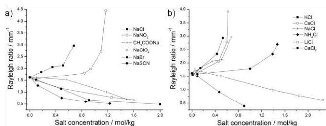
Figure 9. a) Rayleigh ratio in \text{mm}^{-1} obtained from DLS plotted against the anion concentration in \text{mol/kg} ; and b) Rayleigh ratio in \text{mm}^{-1} obtained from DLS plotted against the cation concentration in \text{mol/kg} .
