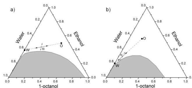
Figure 1. a) Ternary phase diagram in weight fractions of the system water/ethanol/1-octanol, at 25°C; b) Ternary phase diagram in mole fractions of the same system, at 25°C. The clear and homogeneous phase is represented in white, the multiphase domain in gray. Positions corresponding to the octanol-rich and water-rich pseudo-phases are shown as points respectively labeled O and W. Direction of fluctuations considered in dynamic studies are shown with the arrows: the black arrows represent the local fluctuation of aggregates concentration, the gray arrows represent the in-out fluctuation of ethanol between both pseudo-phases.
