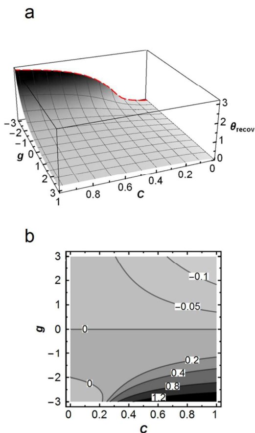
Figure 3. a) Recovered Frumkin isotherms for a range of g values. Red dashed border delineates the shape of the isotherm for g = -3 . b) Error in recovery \theta_n for Frumkin isotherms, as defined in the text.
