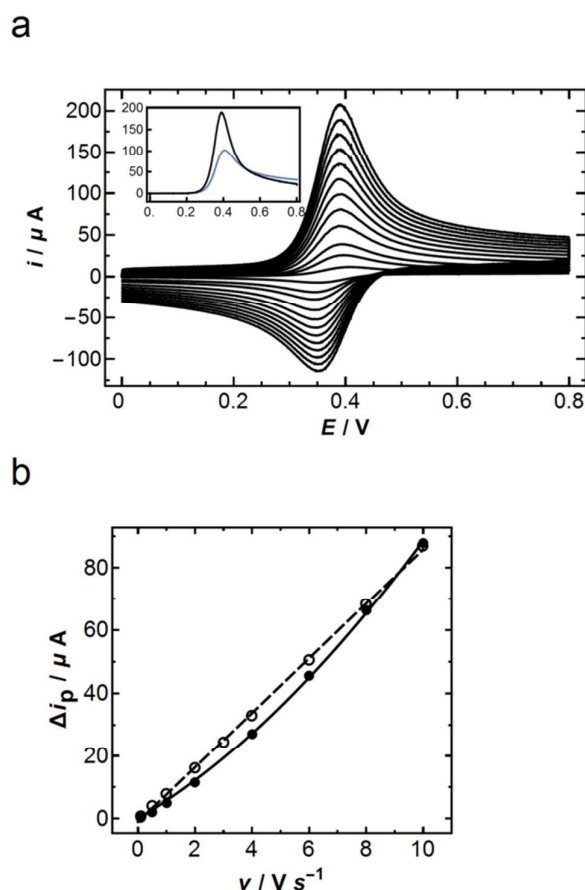
Figure 4. a) CVs for the oxidation of 0.25 mM FcTMA + in 1 M KCl at freshly cleaved AM grade HOPG with scan rates of 0.1, 0.5 and 1–10 V s -1 (with an increment of 1 V s -1 ). The inset shows the experimental forward wave at 10 V s -1 (black) compared with the corresponding computed diffusional wave (blue), crossing at ca. 0.55 V b) Peak current difference \Delta i_p plotted vs scan rate. Filled circles are for FcTMA + data from the CVs presented in a with the fit to a second-order polynomial y(x) = C_1x + C_2x^2 . Open circles are for FcCOOH (0.25 mM in 1 M KCl) with the fit to a straight line. Electrode areas were ca. 0.2 cm 2 .
