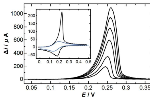
Figure 7. a) Difference plot ( \Delta i = i_{\text{tot}} - i_{\text{diff}} ): forward waves for 0.25 mM FcCH 2 OH at a freshly cleaved AM HOPG with a scan rate of 0.1, 0.5 and 1–10 V s -1 (with increment of 1 V s -1 ). The inset shows a full experimental CV (black) and a computed diffusional one (blue) for v = 1 V s -1 .
