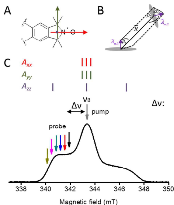
Fig. 7 (A) Hyperfine tensor-frame of the nitroxide C spin label ( ^{14}\text{N} ) A with the principal components x, y and z (orthonormal to the nitroxide plane) marked in red, green and purple, respectively. (B) Three angle restraints and one distance restraint are accessible in an orientation selective PELDOR experiment at X-band frequencies from one spin label pair. \beta_1 and \beta_2 are the angles between the distance vector \vec{R} and the, \vec{A}_{zz,1} and \vec{A}_{zz,2} vectors, respectively. \alpha_2 is the angle between the plane containing the vectors \vec{R} and \vec{A}_{zz,1} and the plane containing vectors \vec{R} and \vec{A}_{zz,2} . (C) Nitroxide EPR spectrum with corresponding ^{14}\text{N} hyperfine stick diagram for X-band frequencies. Arrows indicate the fixed pump ( \nu_B ) frequency and the variable probe ( \nu_A ) frequencies with offsets ranging from \Delta\nu = 40 to 90 MHz.
