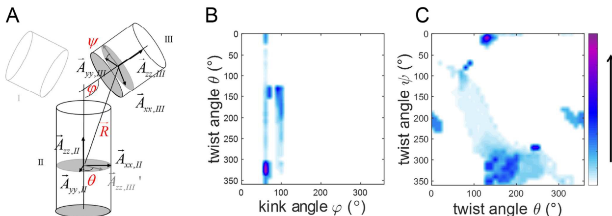
Fig. 5 (A) Definition of bend \varphi and twist angles ( \theta and \psi ). Both helices are represented as cylinders. More details can be found in the Supporting Information. (B) Density plot of twist angle \theta against bend angle \varphi for the conformers found from the simulation of the 2D PELDOR data set for aptamer 1 in the cocaine-bound state. (C) Density plot of twist angle \psi against twist angle \theta . Color bar specifies the density of the conformers to the solution. The data points are interpolated.
