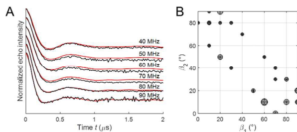
Fig. 4 (A) Experimental X-band 2D PELDOR data set for the aptamer 1 in the cocaine-bound state (black) and fit by an ensemble of spin label conformers (red). (B) Angles \beta_1 and \beta_2 of the 53 spin label conformers used to fit the experimental 2D PELDOR data set. Each circle represents a spin label
