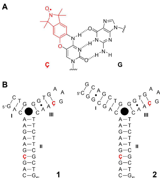
Fig. 1 (A) Spin-labeled nucleoside ̢ , an analogue of 2'-deoxycytidine (modification in red), base-paired to guanine. (B) Secondary structures of the cocaine aptamer constructs 1 and 2 used in this study. Both aptamers have the same sequence and labeling position with the exception of a longer helix I for aptamer 2 . The filled black circle represents the ligand cocaine. The positions that were independently labeled with nucleoside ̢ are shown in red and bold.
