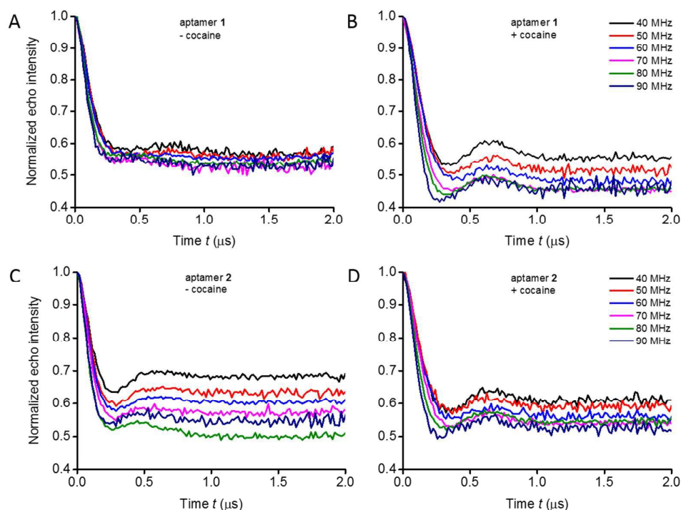
Fig. 2 Experimental background-divided PELDOR time traces measured at frequency offsets \Delta\nu from 40 to 90 MHz at X-band for spin-labeled aptamers 1 (A), (B) and 2 (C), (D) in the absence and presence of cocaine, respectively.
