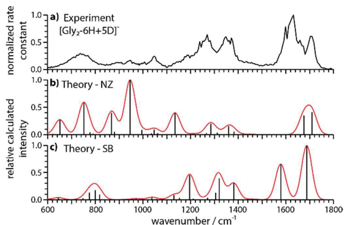
Figure 4 Comparison of a) the experimental IRMPD spectrum of [\text{Gly}_2\text{-6H+5D}]^- with calculated harmonic vibrational spectra for b) NZ and c) SB isomers. The theoretical IR spectra were computed at the B3LYP/6-311++G** level of theory and a uniform scaling factor of 0.985 was used to correct for the systematic errors of harmonic vibrational frequency calculations.
