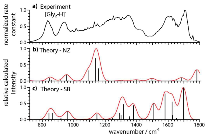
Figure 2 Comparison of a) the experimental IRMPD spectrum of [\text{Gly}_2\text{-H}]^- with calculated harmonic vibrational spectra for b) NZ and c) SB isomers. The theoretical IR spectra were computed at the B3LYP/6-311++G** level of theory and a uniform scaling factor of 0.985 was used to correct for the systematic errors of harmonic vibrational frequency calculations.
