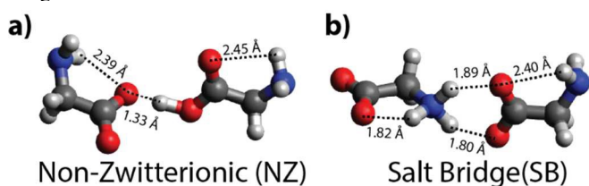
Figure 3 Structural isomers for [\text{Gly}_2\text{-H}]^- with a) a non-zwitterionic (NZ) and b) a salt bridge structure (SB) computed at the B3LYP/6-311++G** level of theory. The hydrogen bonds are indicated by dashed lines and the corresponding bond lengths are included. Oxygen, nitrogen, carbon and hydrogen atoms are represented by red, blue, grey and white spheres, respectively.
