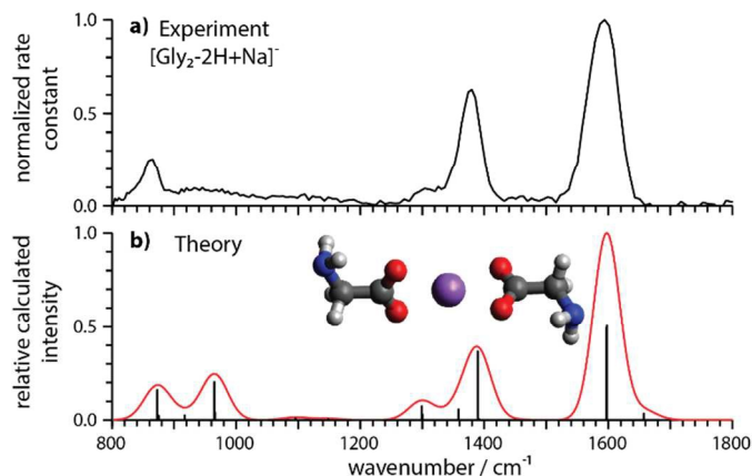
Figure 1 Comparison of a) the experimental IRMPD spectrum of [Gly 2 -2H+Na] - with b) the calculated harmonic vibrational spectrum of the lowest energy isomer (structure inset). The theoretical IR spectra were computed at the B3LYP/6-311++G** level of theory and a uniform scaling factor of 0.985 was used to correct for the systematic errors of harmonic vibrational frequency calculations.
