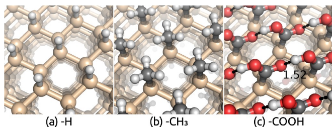
Fig. 1 Geometry of (a) hydrogen, (b) methyl and (c) carboxylic acid terminated Si(111) surfaces. Calculations used an inversion-symmetric 1 \times 1 surface unit cell with four layers and atom positions optimized self-consistently in both vacuum and solution.
