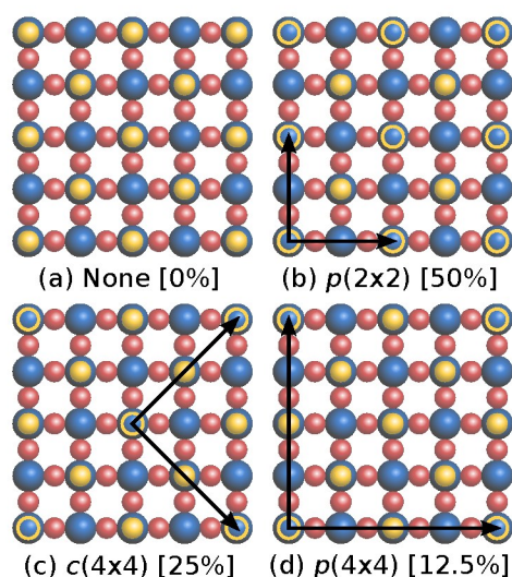
Fig. 5 Schematic top view of configurations of O vacancies on the \text{WO}_3(001) surface ((a) 0%, (b) 50%, (c) 25%, (d) 12.5%). The solid yellow circles are the surface O atoms, empty yellow circles mark the O vacancies and black arrows indicate the lattice vectors of the supercell. For clarity, the monoclinic distortions (see Fig. 4) have been omitted in this illustration.
