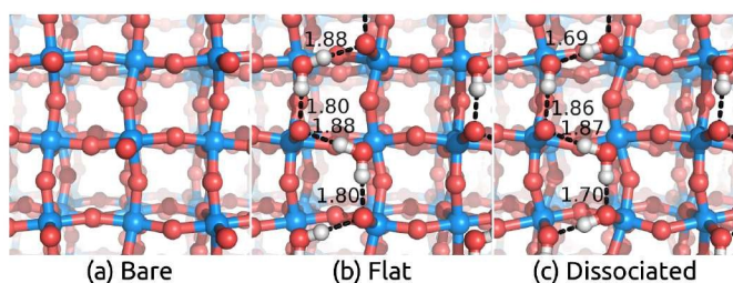
Fig. 4 Geometry of (a) bare \text{WO}_3(001) surface and surfaces with (b) flat adsorbed water molecules and (c) dissociated adsorbed water molecules. Calculations used an inversion-symmetric 1 \times 1 four layer surface unit cell with self-consistent atom positions in solution.
