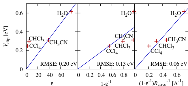
Fig. 7 Correlation of the predicted solvation shift of IrO 2 (110) band positions in various solvents with various combinations of solvent dielectric constant \epsilon and vdW radius R_{\text{vdW}} .
